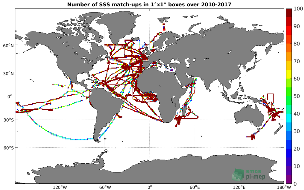
Figure 4: Number of SSS match-ups between TSG (GOSUD-Research-vessel) SSS and the SMOS SSS L3 v2 - Monthly - 0.25 Deg (CATDS-CECOS-IFREMER) SSS product for the Global Ocean Pi-MEP region over 1^\circ \times 1^\circ boxes and for the full satellite product period.
