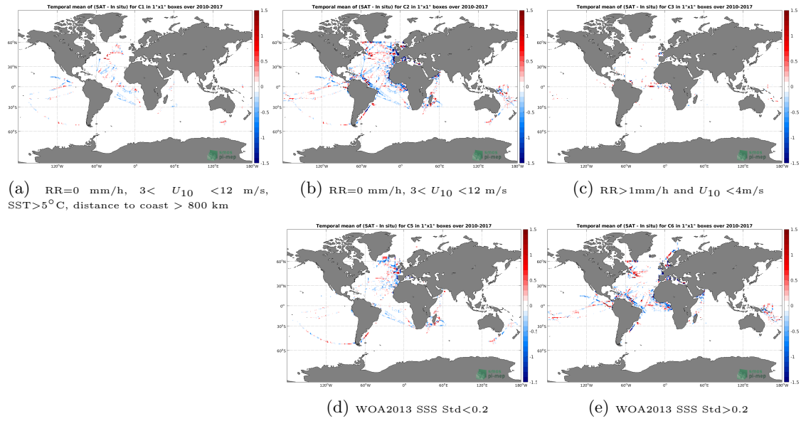
Figure 12: Temporal mean gridded over spatial boxes of size 1^\circ \times 1^\circ of \Delta SSS (SMOS SSS L3 v2 - Monthly - 0.25 Deg (CATDS-CECOS-IFREMER) - TSG (GOSUD-Research-vessel)) for 5 different subdatasets corresponding to: RR=0 mm/h, 3 < U_{10} < 12 m/s, SST > 5^\circ C , distance to coast > 800 km (a), RR=0 mm/h, 3 < U_{10} < 12 m/s (b), RR > 1 mm/h and U_{10} < 4 m/s (c), WOA2013 SSS Std < 0.2 (d), WOA2013 SSS Std > 0.2 (e).
