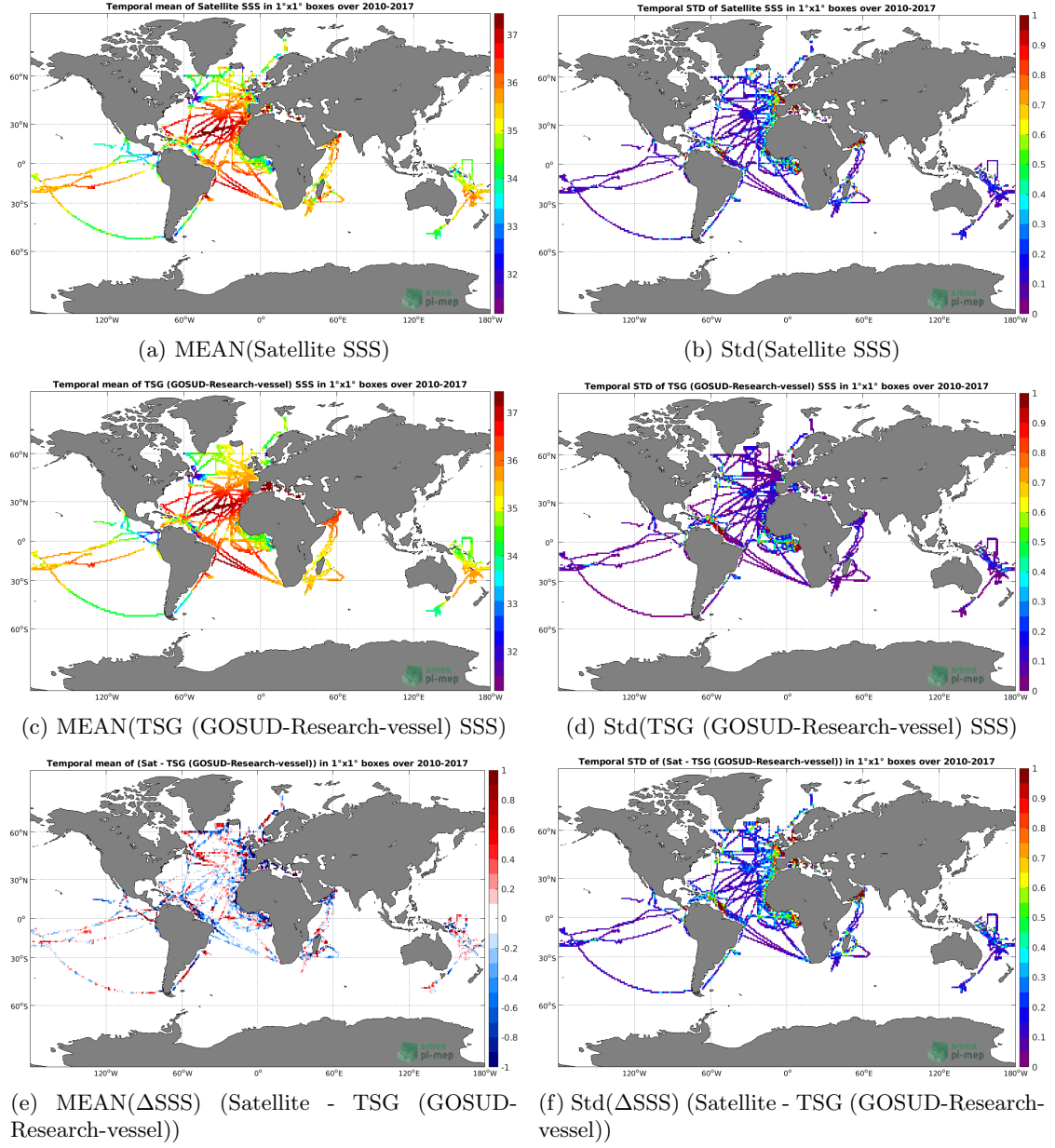
Figure 6: Temporal mean (left) and Std (right) of SSS from SMOS SSS L3 v2 - Monthly - 0.25 Deg (CATDS-CECOS-IFREMER) (top), TSG (GOSUD-Research-vessel) (middle), and of \Delta SSS (Satellite - TSG (GOSUD-Research-vessel)). Only match-up pairs are used to generate these maps.
