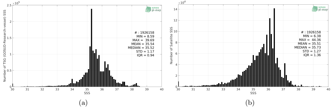
Figure 2: Histograms of SSS from TSG (GOSUD-Research-vessel) (a) and SMOS SSS L3 v2 - Monthly - 0.25 Deg (CATDS-CECOS-IFREMER) (b) considering all match-up pairs per bins of 0.1 over the Global Ocean Pi-MEP region and for the full satellite product period.
