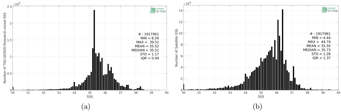
Figure 2: Histograms of SSS from TSG-GOSUD-Research-vessel (a) and SMOS L3 v2 - Monthly - 0.25 Deg (CATDS-CECOS-IFREMER) (b) considering all match-up pairs per bins of 0.1 over the Global Ocean Pi-MEP region and for the full satellite product period.
