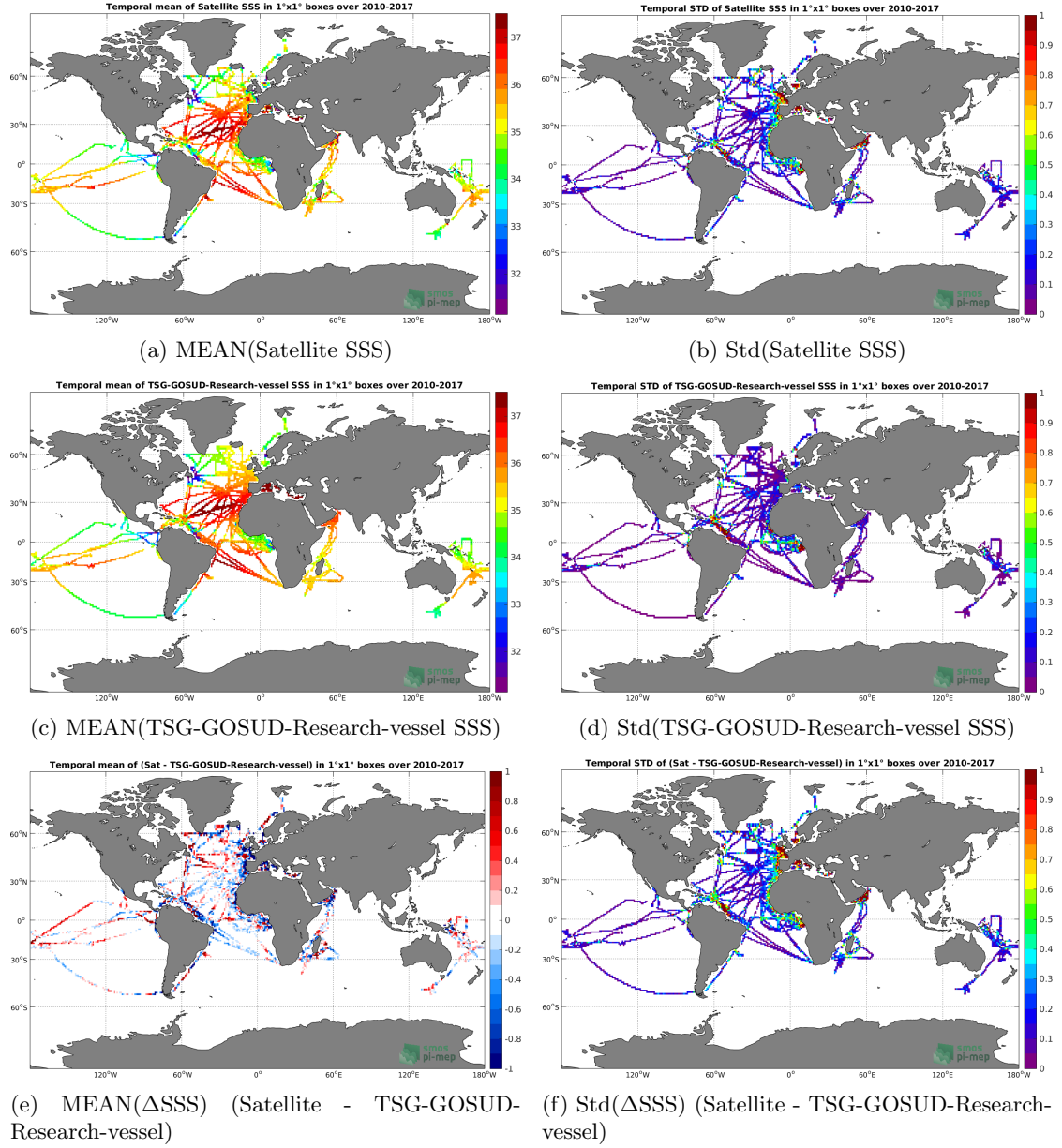
Figure 6: Temporal mean (left) and Std (right) of SSS from SMOS L3 v2 - Monthly - 0.25 Deg (CATDS-CECOS-IFREMER) (top), TSG-GOSUD-Research-vessel (middle), and of \Delta SSS (Satellite - TSG-GOSUD-Research-vessel). Only match-up pairs are used to generate these maps.
