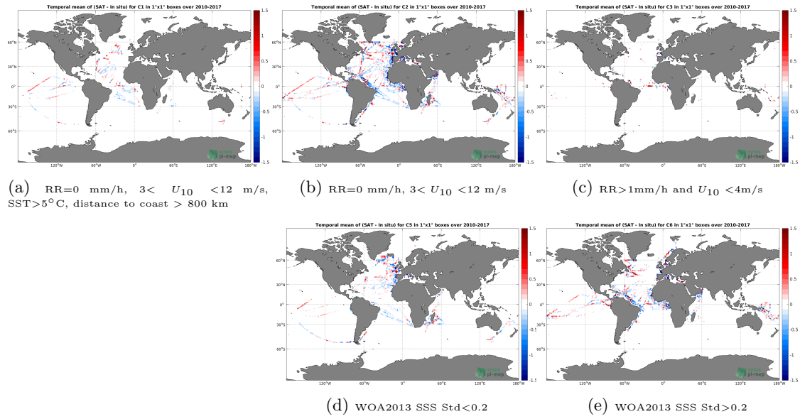
Figure 12: Temporal mean gridded over spatial boxes of size 1^\circ \times 1^\circ of \Delta SSS (SMOS L3 v2 - Monthly - 0.25 Deg (CATDS-CECOS-IFREMER) - TSG-GOSUD-Research-vessel) for 5 different subdatasets corresponding to:RR=0 mm/h, 3 < U_{10} < 12 m/s, SST >5^\circ C, distance to coast > 800 km (a), RR=0 mm/h, 3 < U_{10} < 12 m/s (b), RR >1 mm/h and U_{10} < 4 m/s (c), WOA2013 SSS Std <0.2 (d), WOA2013 SSS Std >0.2 (e).
