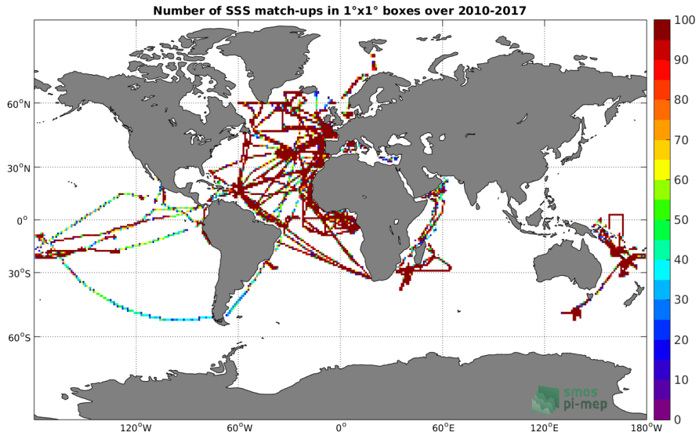
Figure 4: Number of SSS match-ups between TSG-GOSUD-Research-vessel SSS and the SMOS L3 v2 - Monthly - 0.25 Deg (CATDS-CECOS-IFREMER) SSS product for the Global Ocean Pi-MEP region over 1°x1° boxes and for the full satellite product period.
