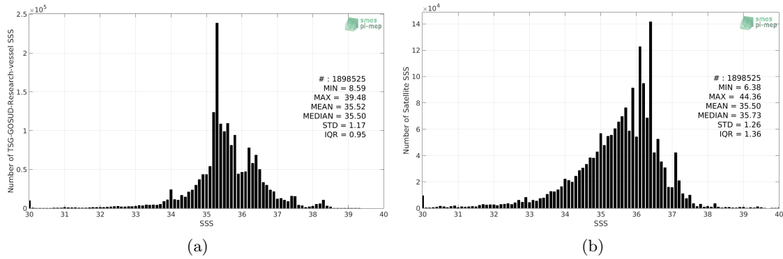
Figure 2: Histograms of SSS from TSG-GOSUD-Research-vessel (a) and SMOS-L3-CATDS-IFREMER-CECOS-V2-MONTHLY-0.25DEG (b) considering all match-up pairs per bins of 0.1 over the Global Ocean Pi-MEP region and for the full satellite product period.
