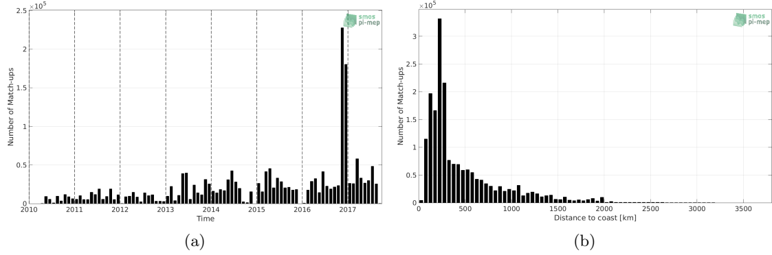
Figure 1: Number of match-ups between TSG-GOSUD-Research-vessel and SMOS-L3-CATDS-IFREMER-CECOS-V2-MONTHLY-0.25DEG SSS as a function of time (a) and as function of the distance to coast (b) over the Global Ocean Pi-MEP region and for the full satellite product period.
