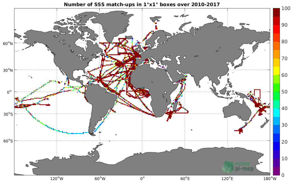
Figure 4: Number of SSS match-ups between TSG-GOSUD-Research-vessel SSS and the SMOS-L3-CATDS-IFREMER-CECOS-V2-MONTHLY-0.25DEG SSS product for the Global Ocean Pi-MEP region over 1°x1° boxes and for the full satellite product period.
