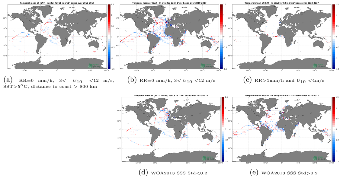
Figure 12: Temporal mean gridded over spatial boxes of size 1^\circ \times 1^\circ of \Delta SSS (SMOS-L3-CATDS-IFREMER-CECOS-V2-MONTHLY-0.25DEG - TSG-GOSUD-Research-vessel) for 5 different subdatasets corresponding to: RR=0 mm/h, 3 < U_{10} < 12 m/s, SST > 5^\circ\text{C} , distance to coast > 800 km (a), RR=0 mm/h, 3 < U_{10} < 12 m/s (b), RR > 1\text{mm/h} and U_{10} < 4\text{m/s} (c), WOA2013 SSS Std < 0.2 (d), WOA2013 SSS Std > 0.2 (e).
