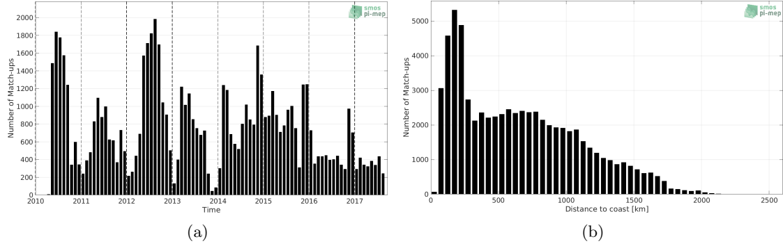
Figure 1: Number of match-ups between Sea mammals and SMOS SSS L3 v2 - Monthly - 0.25 Deg (CATDS-CECOS-IFREMER) SSS as a function of time (a) and as function of the distance to coast (b) over the Global Ocean Pi-MEP region and for the full satellite product period.
