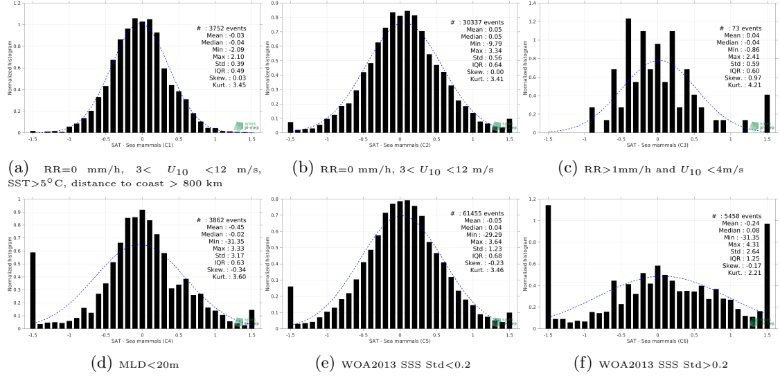
Figure 13: Normalized histogram of \Delta SSS (SMOS SSS L3 v2 - Monthly - 0.25 Deg (CATDS-CECOS-IFREMER) - Sea mammals) for 6 different subdatasets corresponding to: RR=0 mm/h, 3 < U_{10} < 12 m/s, SST>5°C, distance to coast > 800 km (a), RR=0 mm/h, 3 < U_{10} < 12 m/s (b), RR>1mm/h and U_{10} < 4 m/s (c), MLD<20m (d), WOA2013 SSS Std<0.2 (e), WOA2013 SSS Std>0.2 (f).
