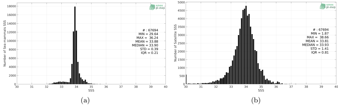
Figure 2: Histograms of SSS from Sea mammals (a) and SMOS SSS L3 v2 - Monthly - 0.25 Deg (CATDS-CECOS-IFREMER) (b) considering all match-up pairs per bins of 0.1 over the Global Ocean Pi-MEP region and for the full satellite product period.
