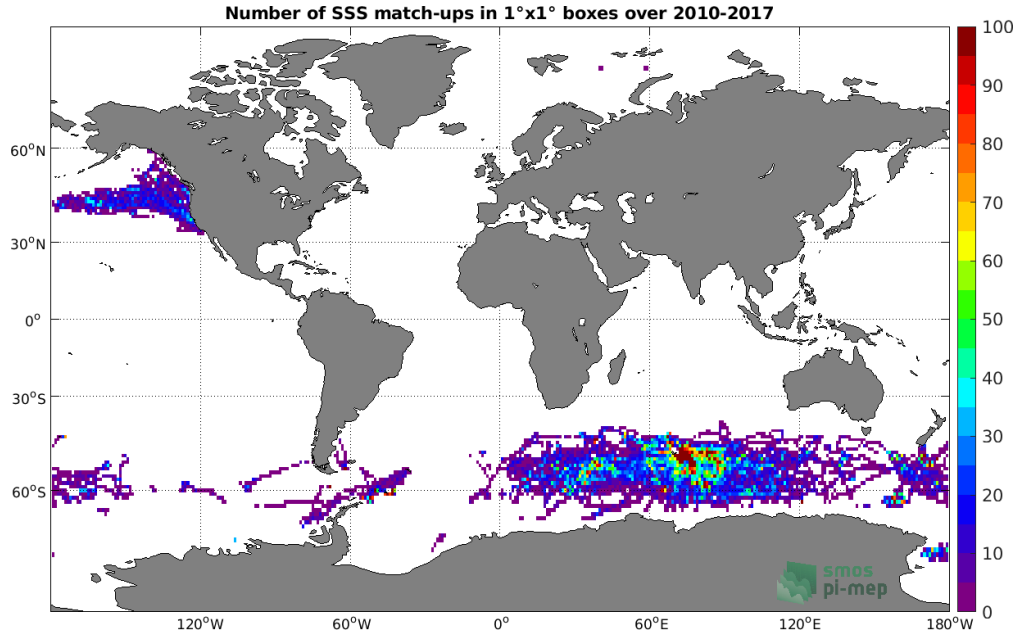
Figure 4: Number of SSS match-ups between Sea mammals SSS and the SMOS SSS L3 v2 - Monthly - 0.25 Deg (CATDS-CECOS-IFREMER) SSS product for the Global Ocean Pi-MEP region over 1^\circ \times 1^\circ boxes and for the full satellite product period.
