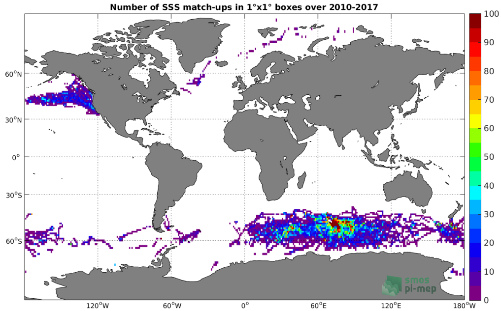
Figure 4: Number of SSS match-ups between Sea mammals SSS and the SMOS SSS L3 v2 - Monthly - 0.25 Deg (CATDS-CECOS-IFREMER) SSS product for the Global Ocean Pi-MEP region over 1°x1° boxes and for the full satellite product period.
