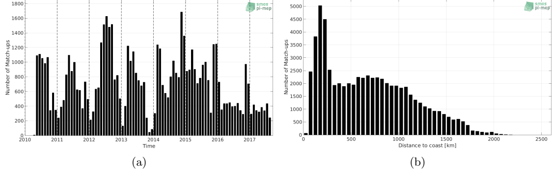
Figure 1: Number of match-ups between Sea mammals and SMOS L3 v2 - Monthly - 0.25 Deg (CATDS-CECOS-IFREMER) SSS as a function of time (a) and as function of the distance to coast (b) over the Global Ocean Pi-MEP region and for the full satellite product period.
