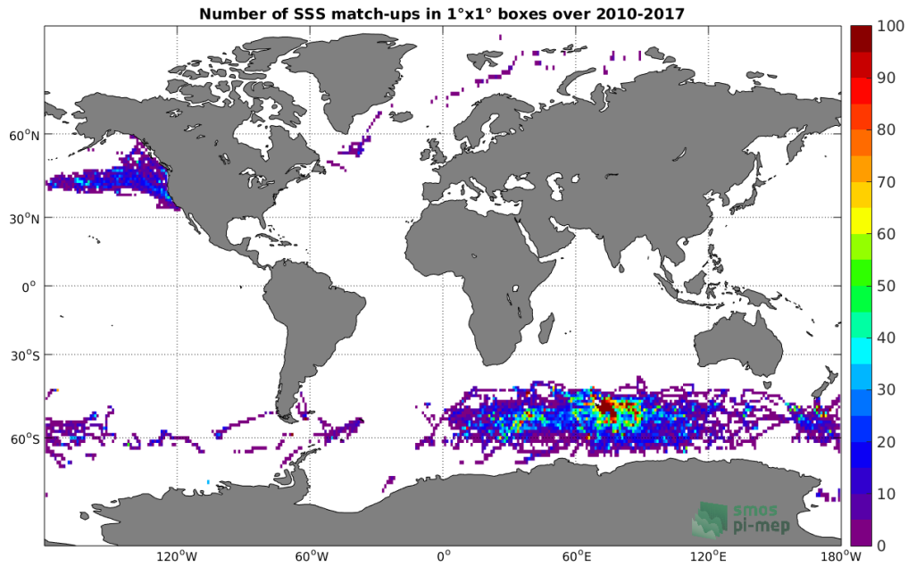
Figure 4: Number of SSS match-ups between Sea mammals SSS and the SMOS L3 v2 - Monthly - 0.25 Deg (CATDS-CECOS-IFREMER) SSS product for the Global Ocean Pi-MEP region over 1^\circ \times 1^\circ boxes and for the full satellite product period.
