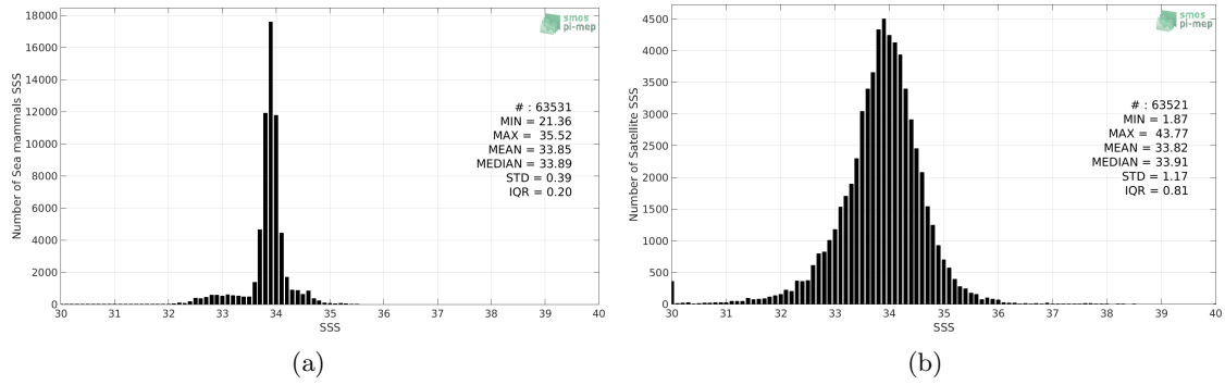
Figure 2: Histograms of SSS from Sea mammals (a) and SMOS L3 v2 - Monthly - 0.25 Deg (CATDS-CECOS-IFREMER) (b) considering all match-up pairs per bins of 0.1 over the Global Ocean Pi-MEP region and for the full satellite product period.
