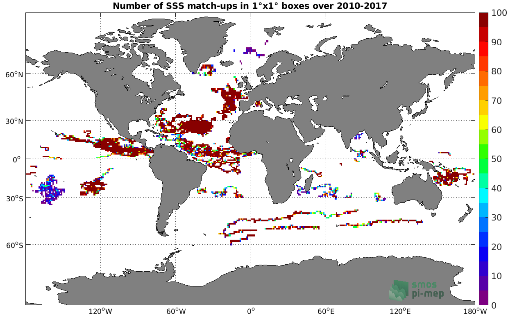
Figure 3: Number of SSS match-ups between Surface drifters SSS and the SMOS SSS L3 v2 - Monthly - 0.25 Deg (CATDS-CECOS-IFREMER) SSS product for the Global Ocean Pi-MEP region over 1^\circ \times 1^\circ boxes and for the full satellite product period.
