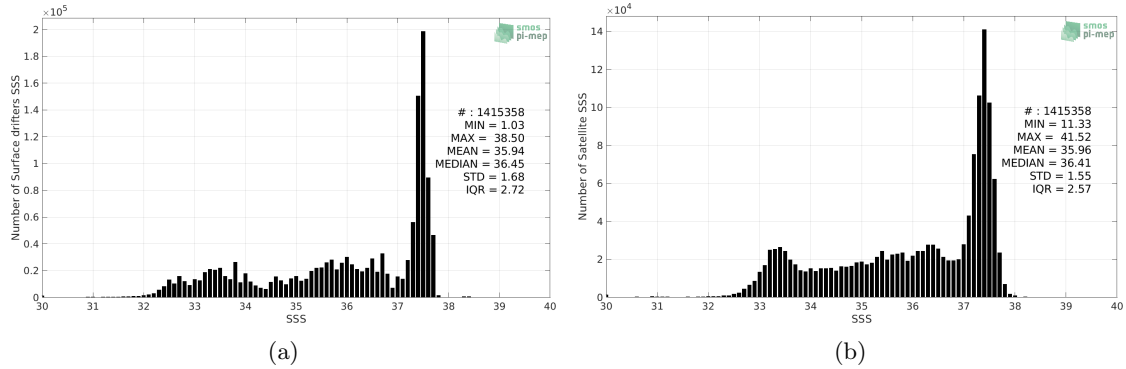
Figure 2: Histograms of SSS from Surface drifters (a) and SMOS SSS L3 v2 - Monthly - 0.25 Deg (CATDS-CECOS-IFREMER) (b) considering all match-up pairs per bins of 0.1 over the Global Ocean Pi-MEP region and for the full satellite product period.
