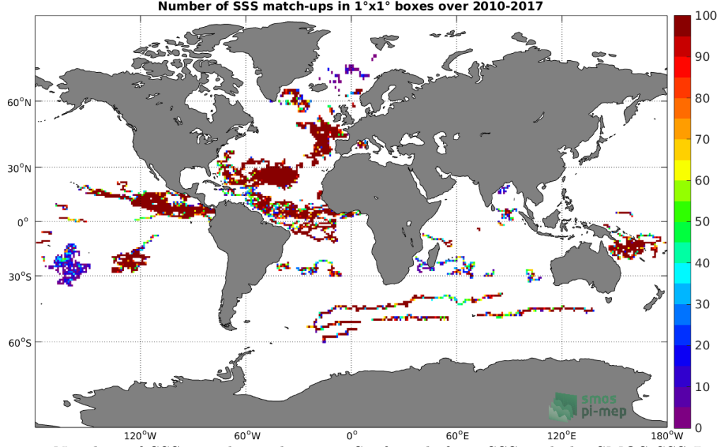
Figure 3: Number of SSS match-ups between Surface drifters SSS and the SMOS SSS L3 v2 - Monthly - 0.25 Deg (CATDS-CECOS-IFREMER) SSS product for the Global Ocean Pi-MEP region over 1°x1° boxes and for the full satellite product period.
