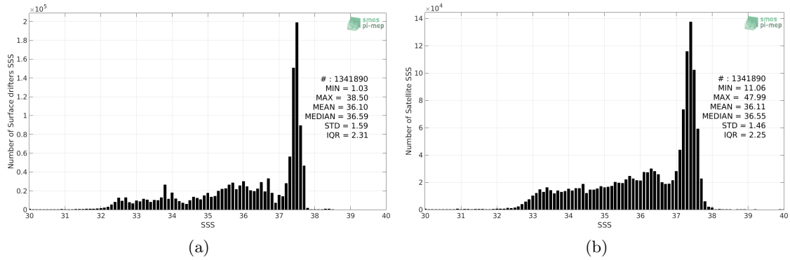
Figure 2: Histograms of SSS from Surface drifters (a) and SMOS L3 v2 - Monthly - 0.25 Deg (CATDS-CECOS-IFREMER) (b) considering all match-up pairs per bins of 0.1 over the Global Ocean Pi-MEP region and for the full satellite product period.
