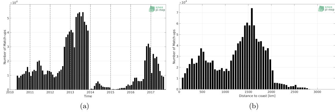
Figure 1: Number of match-ups between Surface drifters and SMOS L3 v2 - Monthly - 0.25 Deg (CATDS-CECOS-IFREMER) SSS as a function of time (a) and as function of the distance to coast (b) over the Global Ocean Pi-MEP region and for the full satellite product period.
