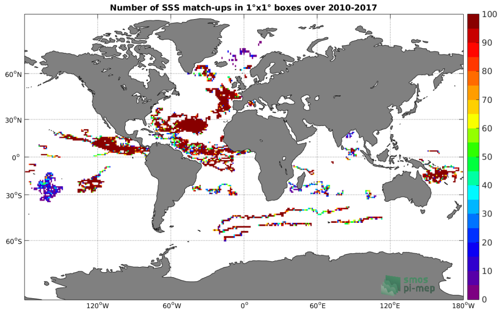
Figure 3: Number of SSS match-ups between Surface drifters SSS and the SMOS L3 v2 - Monthly - 0.25 Deg (CATDS-CECOS-IFREMER) SSS product for the Global Ocean Pi-MEP region over 1°x1° boxes and for the full satellite product period.
