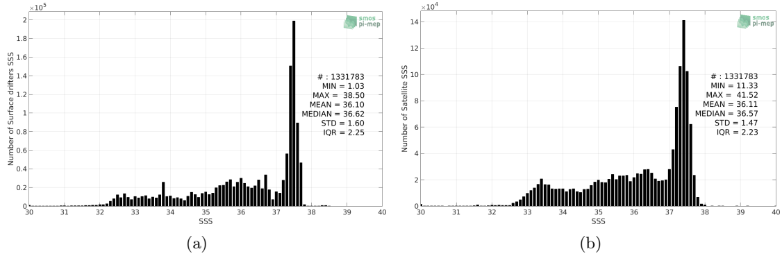
Figure 2: Histograms of SSS from Surface drifters (a) and SMOS-L3-CATDS-IFREMER-CECOS-V2-MONTHLY-0.25DEG (b) considering all match-up pairs per bins of 0.1 over the Global Ocean Pi-MEP region and for the full satellite product period.
