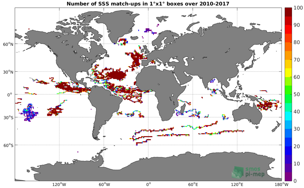
Figure 3: Number of SSS match-ups between Surface drifters SSS and the SMOS-L3-CATDS-IFREMER-CECOS-V2-MONTHLY-0.25DEG SSS product for the Global Ocean Pi-MEP region over 1°x1° boxes and for the full satellite product period.
