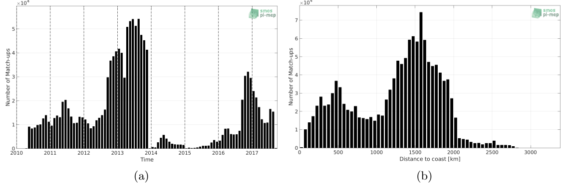
Figure 1: Number of match-ups between Surface drifters and SMOS-L3-CATDS-IFREMER-CECOS-V2-MONTHLY-0.25DEG SSS as a function of time (a) and as function of the distance to coast (b) over the Global Ocean Pi-MEP region and for the full satellite product period.
