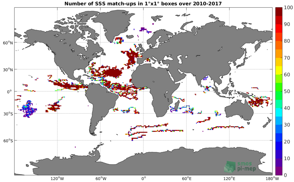
Figure 3: Number of SSS match-ups between Surface drifters SSS and the SMOS-L3-CATDS-IFREMER-CECOS-V2-MONTHLY-0.25DEG SSS product for the Global Ocean Pi-MEP region over 1^\circ \times 1^\circ boxes and for the full satellite product period.
