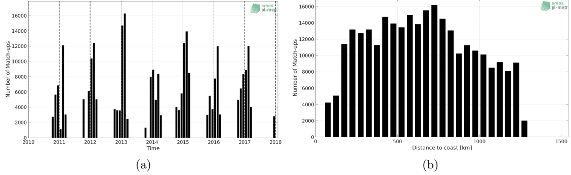
Figure 1: Number of match-ups between TSG (LEGOS-Survostral) and SMOS SSS L3 v2 - Daily - 0.5 Deg (CATDS-CECOS-IFREMER) SSS as a function of time (a) and as function of the distance to coast (b) over the Global Ocean Pi-MEP region and for the full satellite product period.
