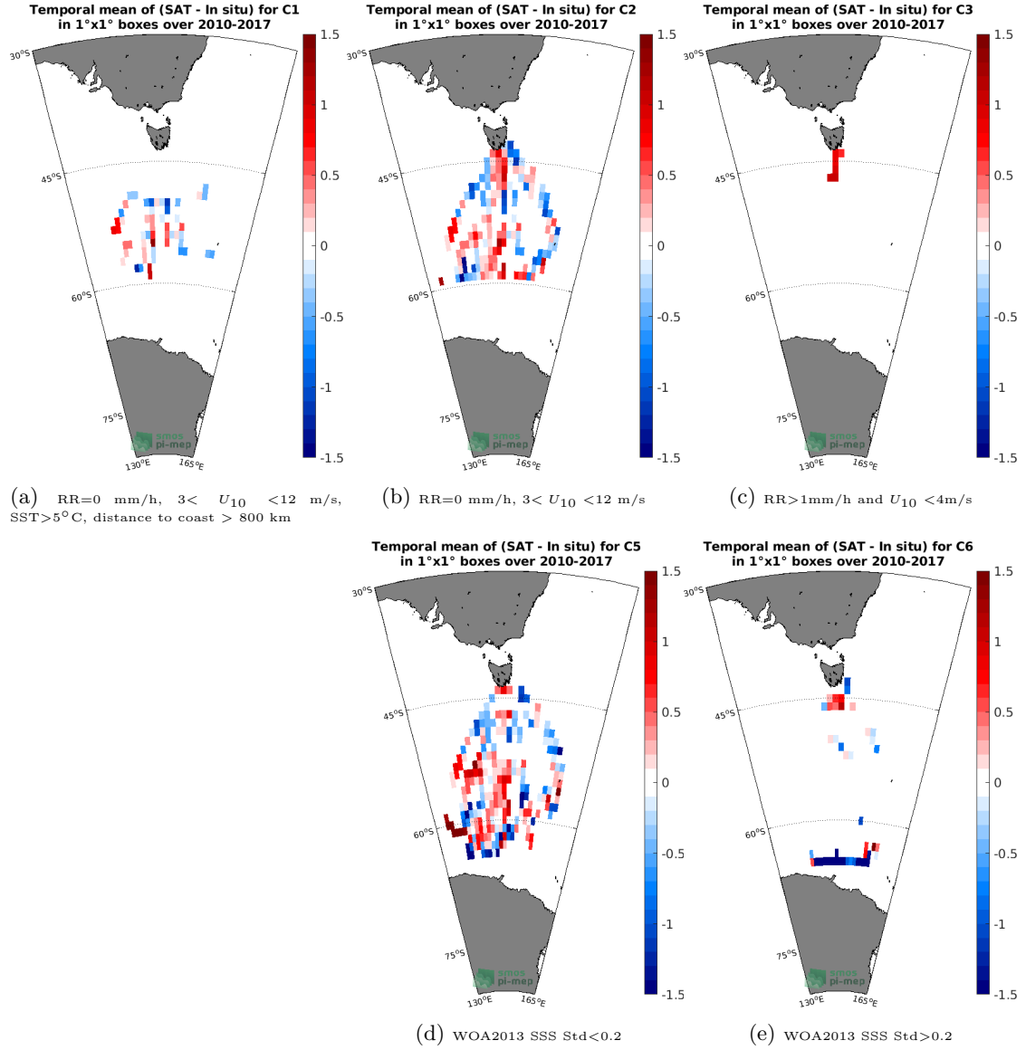
Figure 12: Temporal mean gridded over spatial boxes of size 1°x1° of \Delta\text{SSS} (SMOS SSS L3 v2 - Daily - 0.5 Deg (CATDS-CECOS-IFREMER) - TSG (LEGOS-Survostral)) for 5 different subdatasets corresponding to: RR=0 mm/h, 3 < U_{10} < 12 m/s, SST > 5^{\circ}\text{C} , distance to coast > 800 km (a), RR=0 mm/h, 3 < U_{10} < 12 m/s (b), RR > 1\text{mm/h} and U_{10} < 4\text{m/s} (c), WOA2013 SSS Std <0.2 (d), WOA2013 SSS Std >0.2 (e).
