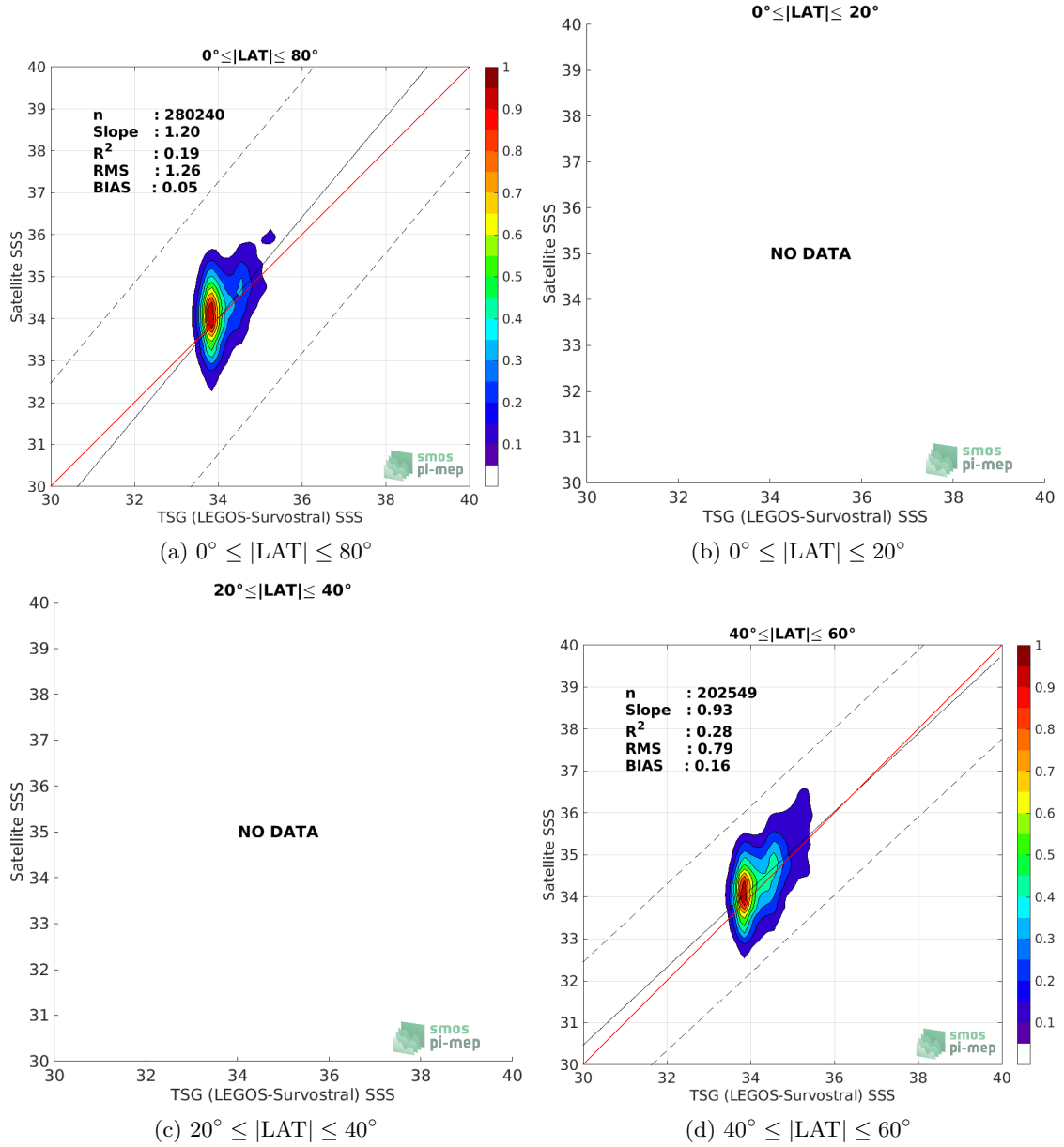
Figure 9: Contour maps of the concentration of SMOS SSS L3 v2 - Daily - 0.5 Deg (CATDS-CECOS-IFREMER) SSS (y-axis) versus TSG (LEGOS-Survostral) SSS (x-axis) at match-up pairs for different latitude bands. For each plot, the red line shows x=y . The black thin and dashed lines indicate a linear fit through the data cloud and the \pm 95\% confidence levels, respectively. The number match-up pairs n , the slope and R^2 coefficient of the linear fit, the root mean square (RMS) and the mean bias between satellite and in situ data are indicated for each latitude band in each plots.
