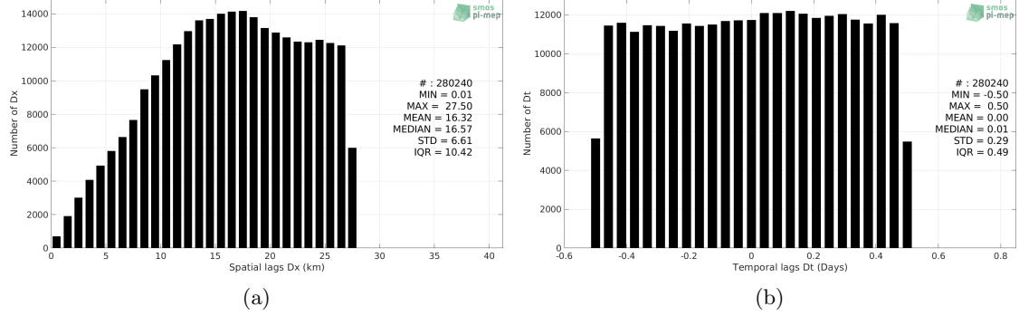
Figure 5: Histograms of the spatial (a) and temporal (b) lags between the location/time of the TSG (LEGOS-Survostral) measurement and the date of the corresponding SMOS SSS L3 v2 - Daily - 0.5 Deg (CATDS-CECOS-IFREMER) SSS pixel.
