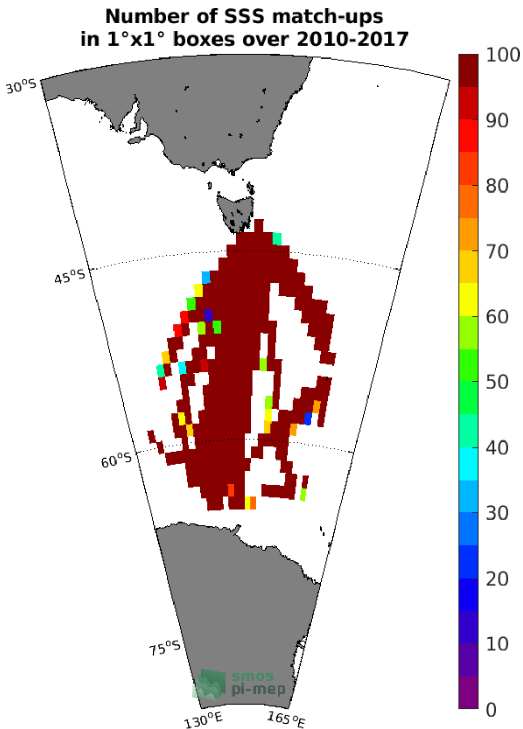
Figure 4: Number of SSS match-ups between TSG (LEGOS-Survostral) SSS and the SMOS SSS L3 v2 - Daily - 0.5 Deg (CATDS-CECOS-IFREMER) SSS product for the Global Ocean Pi-MEP region over 1°x1° boxes and for the full satellite product period.
