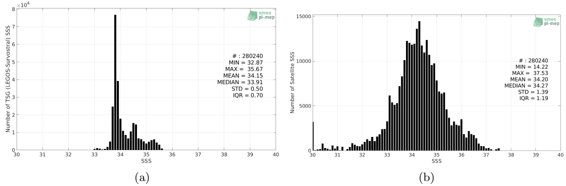
Figure 2: Histograms of SSS from TSG (LEGOS-Survostral) (a) and SMOS SSS L3 v2 - Daily - 0.5 Deg (CATDS-CECOS-IFREMER) (b) considering all match-up pairs per bins of 0.1 over the Global Ocean Pi-MEP region and for the full satellite product period.
