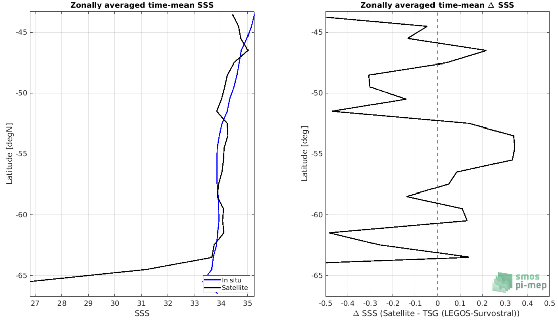
Figure 8: Left panel: Zonal mean SSS from SMOS SSS L3 v2 - Daily - 0.5 Deg (CATDS-CECOS-IFREMER) satellite product (black) and from TSG (LEGOS-Survostral) (blue). Right panel: Zonal mean of \Delta SSS (Satellite - TSG (LEGOS-Survostral)) for all the collected Pi-MEP match-up pairs estimated over the full satellite product period.
