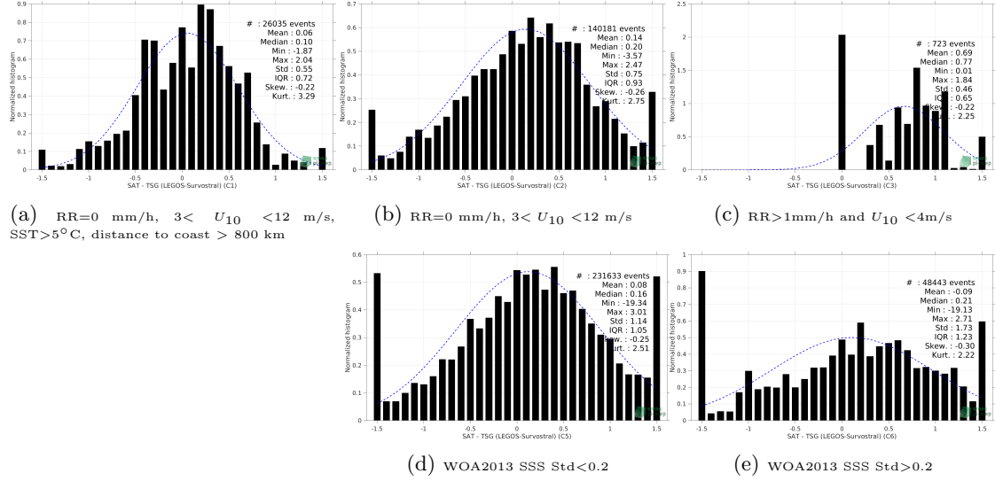
Figure 13: Normalized histogram of \Delta SSS (SMOS SSS L3 v2 - Daily - 0.5 Deg (CATDS-CECOS-IFREMER) - TSG (LEGOS-Survostral)) for 5 different subdatasets corresponding to: RR=0 mm/h, 3 < U_{10} < 12 m/s, SST > 5°C, distance to coast > 800 km (a), RR=0 mm/h, 3 < U_{10} < 12 m/s (b), RR > 1mm/h and U_{10} < 4 m/s (c), WOA2013 SSS Std < 0.2 (d), WOA2013 SSS Std > 0.2 (e).
