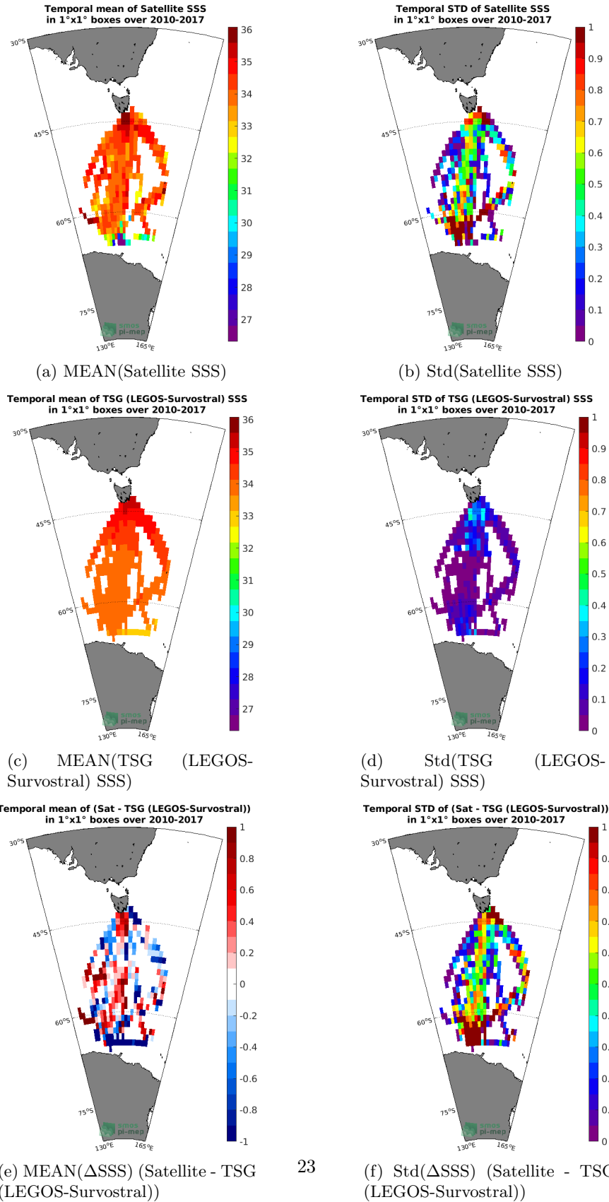
Figure 6: Temporal mean (left) and Std (right) of SSS from SMOS SSS L3 v2 - Daily - 0.5 Deg (CATDS-CECOS-IFREMER) (top), TSG (LEGOS-Survostral) (middle), and of \Delta SSS (Satellite - TSG (LEGOS-Survostral)). Only match-up pairs are used to generate these maps.
