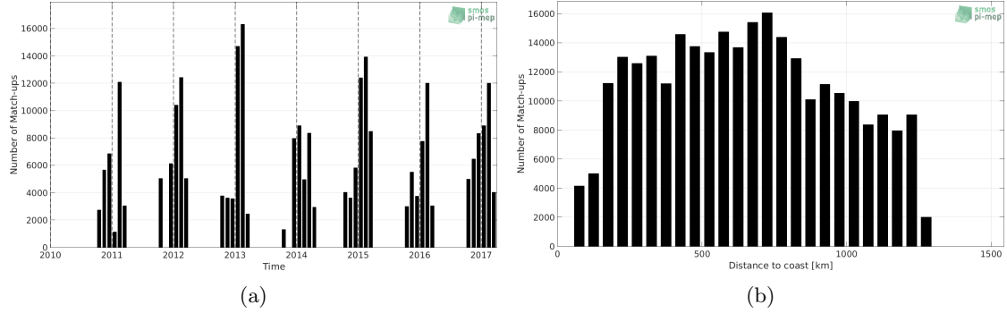
Figure 1: Number of match-ups between TSG-LEGOS-Survostral and SMOS L3 v2 - Daily - 0.5 Deg (CATDS-CECOS-IFREMER) SSS as a function of time (a) and as function of the distance to coast (b) over the Global Ocean Pi-MEP region and for the full satellite product period.
