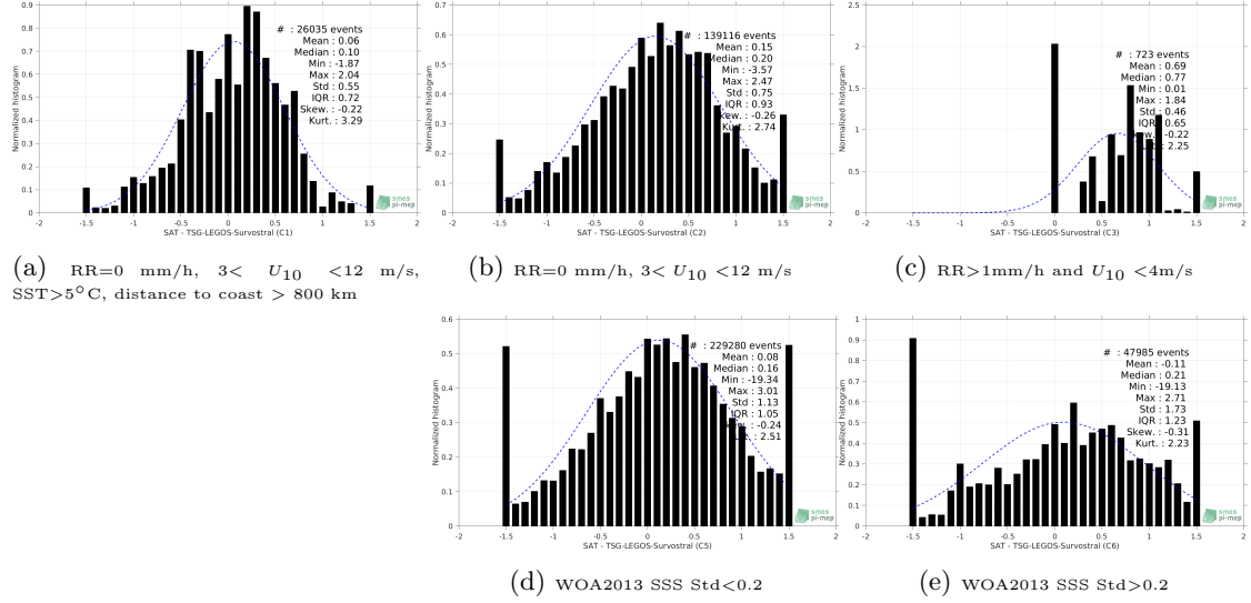
Figure 13: Normalized histogram of \Delta SSS (SMOS L3 v2 - Daily - 0.5 Deg (CATDS-CECOS-IFREMER) - TSG-LEGOS-Survostral) for 5 different subdatasets corresponding to: RR=0 mm/h, 3 < U_{10} < 12 m/s, SST > 5°C, distance to coast > 800 km (a), RR=0 mm/h, 3 < U_{10} < 12 m/s (b), RR > 1mm/h and U_{10} < 4 m/s (c), WOA2013 SSS Std < 0.2 (d), WOA2013 SSS Std > 0.2 (e).
