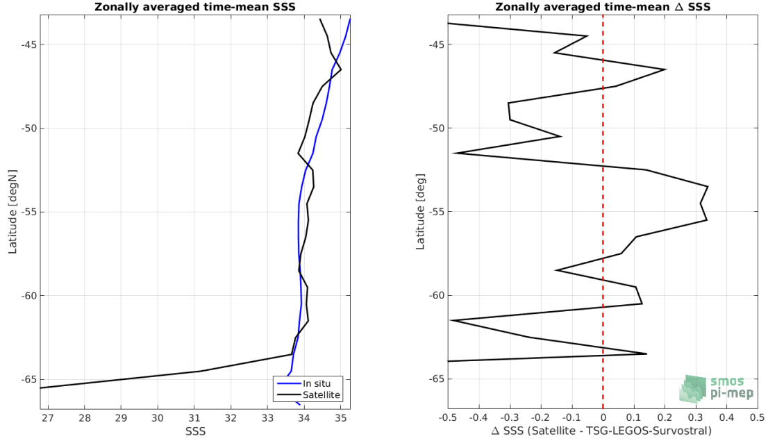
Figure 8: Left panel: Zonal mean SSS from SMOS L3 v2 - Daily - 0.5 Deg (CATDS-CECOS-IFREMER) satellite product (black) and from TSG-LEGOS-Survostral (blue). Right panel: Zonal mean of \Delta SSS (Satellite - TSG-LEGOS-Survostral) for all the collected Pi-MEP match-up pairs estimated over the full satellite product period.
