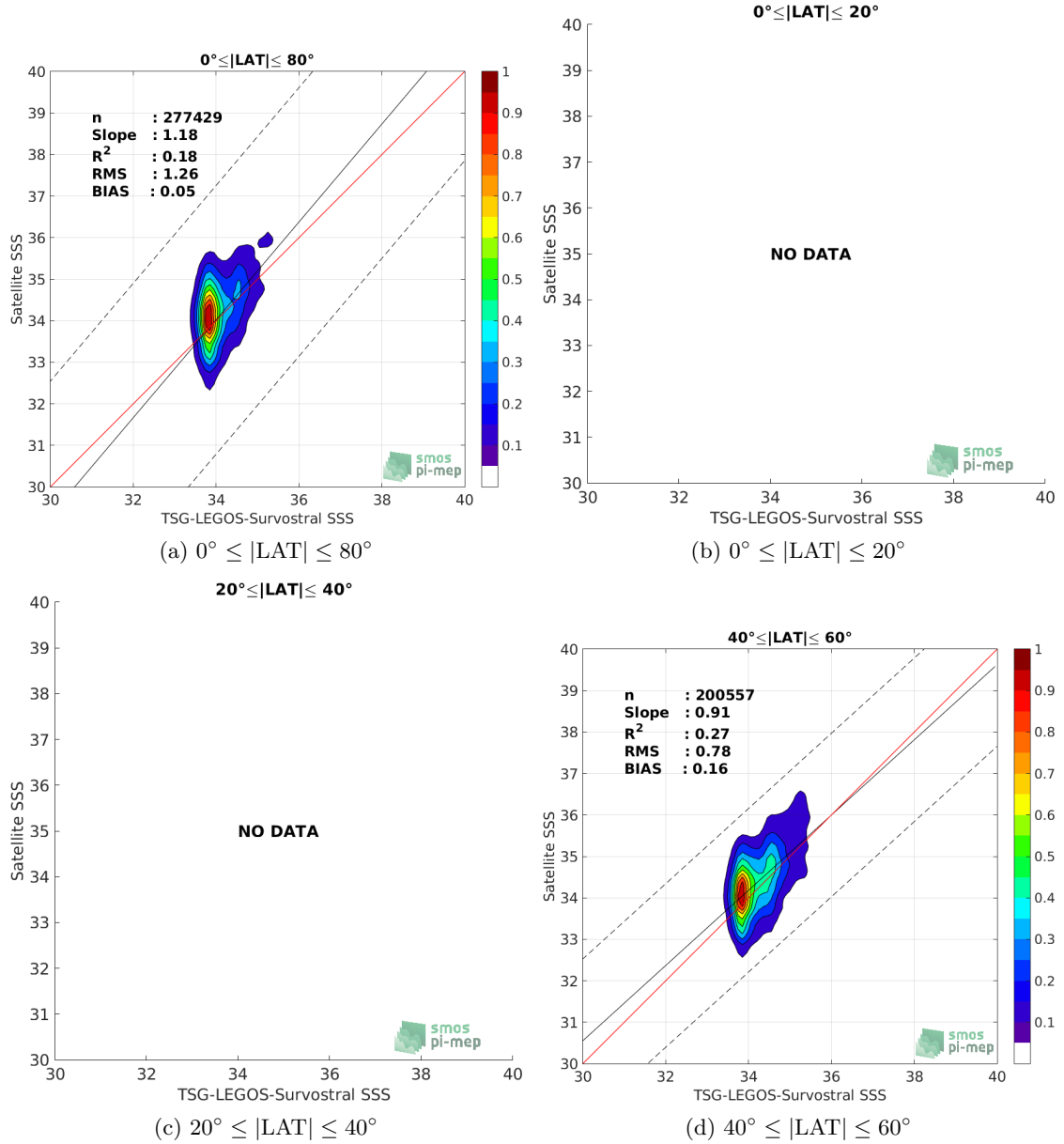
Figure 9: Contour maps of the concentration of SMOS L3 v2 - Daily - 0.5 Deg (CATDS-CECOS-IFREMER) SSS (y-axis) versus TSG-LEGOS-Survostral SSS (x-axis) at match-up pairs for different latitude bands. For each plot, the red line shows x=y . The black thin and dashed lines indicate a linear fit through the data cloud and the \pm 95\% confidence levels, respectively. The number match-up pairs n , the slope and R^2 coefficient of the linear fit, the root mean square (RMS) and the mean bias between satellite and in situ data are indicated for each latitude band in each plots.
