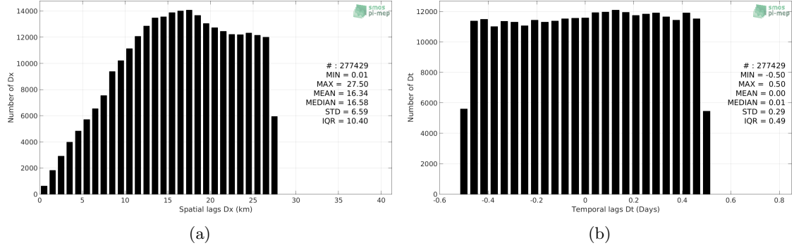
Figure 5: Histograms of the spatial (a) and temporal (b) lags between the time of the TSG-LEGOS-Survostral measurements and the date of the corresponding SMOS L3 v2 - Daily - 0.5 Deg (CATDS-CECOS-IFREMER) SSS product.
