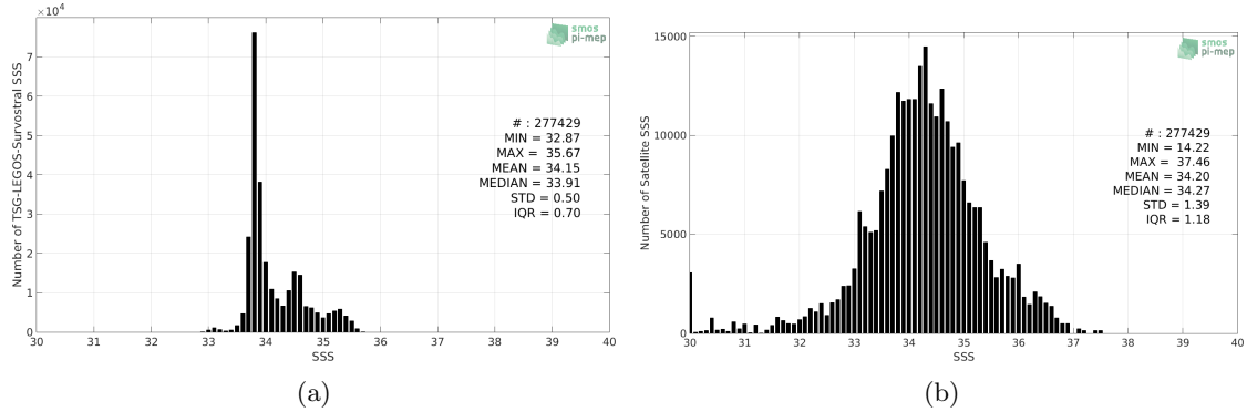
Figure 2: Histograms of SSS from TSG-LEGOS-Survostral (a) and SMOS L3 v2 - Daily - 0.5 Deg (CATDS-CECOS-IFREMER) (b) considering all match-up pairs per bins of 0.1 over the Global Ocean Pi-MEP region and for the full satellite product period.
