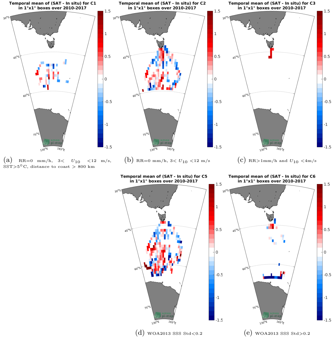
Figure 12: Temporal mean gridded over spatial boxes of size 1°x1° of \Delta\text{SSS} (SMOS L3 v2 - Daily - 0.5 Deg (CATDS-CECOS-IFREMER) - TSG-LEGOS-Survostral) for 5 different subdatasets corresponding to: RR=0 mm/h, 3 < U_{10} < 12 m/s, SST > 5^{\circ}\text{C} , distance to coast > 800 km (a), RR=0 mm/h, 3 < U_{10} < 12 m/s (b), RR > 1\text{mm/h} and U_{10} < 4\text{m/s} (c), WOA2013 SSS Std < 0.2 (d), WOA2013 SSS Std > 0.2 (e).
