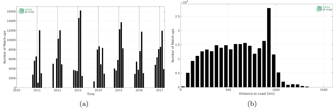
Figure 1: Number of match-ups between TSG-LEGOS-Survostral and SMOS-L3-CATDS-CECOS-IFREMER-V2-1DAY-0.5DEG SSS as a function of time (a) and as function of the distance to coast (b) over the Global Ocean Pi-MEP region and for the full satellite product period.
