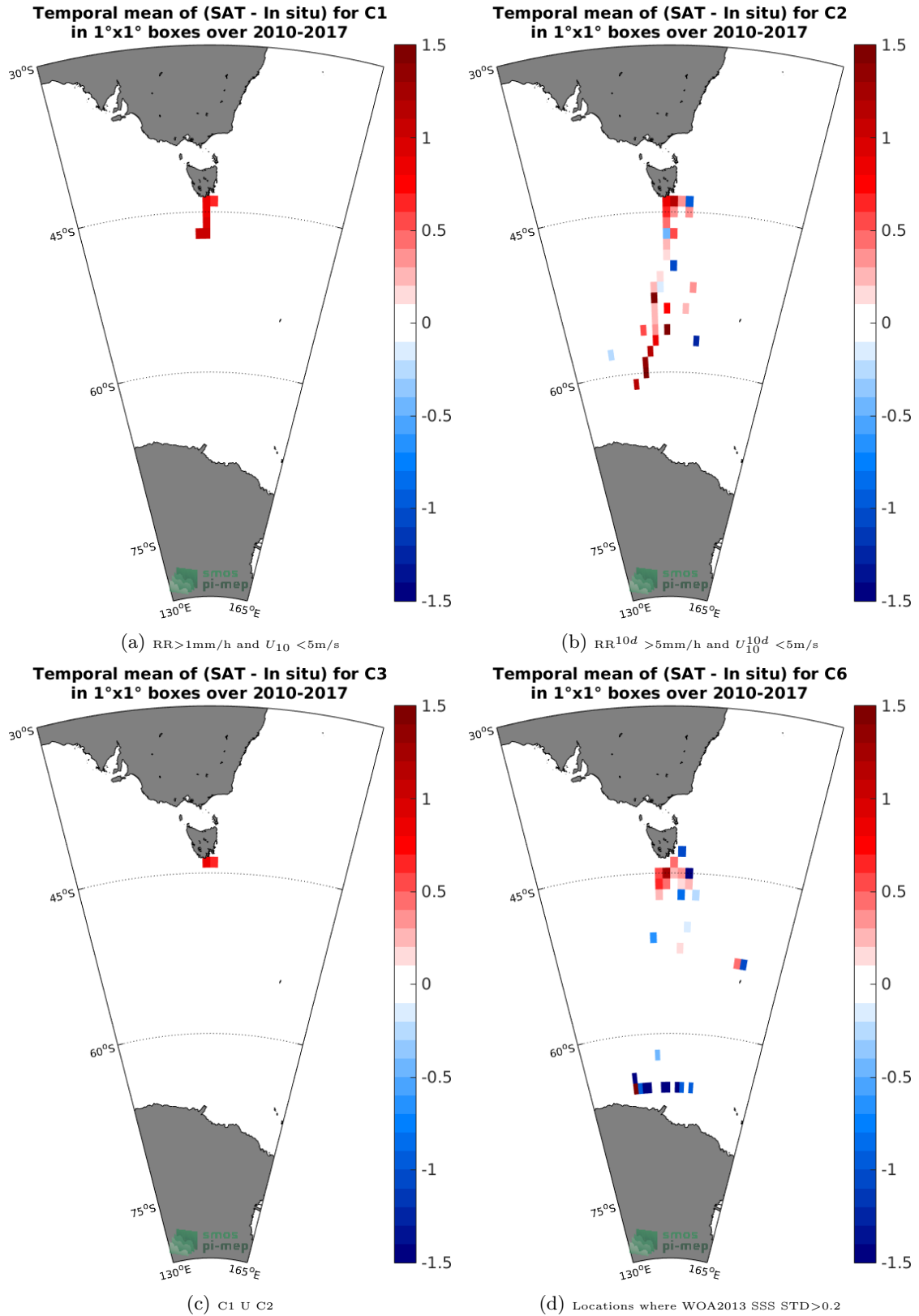
Figure 12: Temporal mean gridded over spatial boxes of size 1°x1° of \Delta\text{SSS} (SMOS-L3-CATDS-CECOS-IFREMER-V2-1DAY-0.5DEG - TSG-LEGOS-Survostral) for 4 different subdatasets corresponding to: RR > 1\text{mm/h} and U_{10} < 5\text{m/s} (a), RR^{10d} > 5\text{mm/h} and U_{10}^{10d} < 5\text{m/s} (b), C1 U C2 (c), Locations where WOA2013 SSS STD > 0.2 (d).
