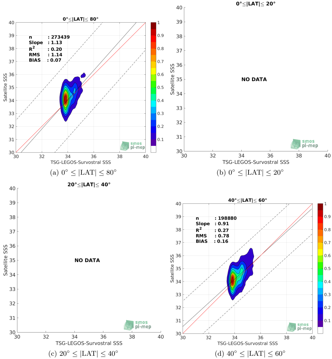
Figure 9: Contour maps of the concentration of SMOS-L3-CATDS-CECOS-IFREMER-V2-1DAY-0.5DEG SSS (y-axis) versus TSG-LEGOS-Survostral SSS (x-axis) at match-up pairs for different latitude bands. For each plot, the red line shows x=y . The black thin and dashed lines indicate a linear fit through the data cloud and the \pm 95\% confidence levels, respectively. The number match-up pairs n , the slope and R^2 coefficient of the linear fit, the root mean square (RMS) and the mean bias between satellite and in situ data are indicated for each latitude band in each plots.
