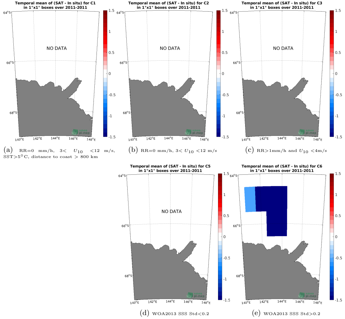
Figure 12: Temporal mean gridded over spatial boxes of size 1°x1° of \Delta SSS (SMOS SSS L3 v2 - Daily - 0.5 Deg (CATDS-CECOS-IFREMER) - TSG (LEGOS-Surv-Adel)) for 5 different subdatasets corresponding to: RR=0 mm/h, 3 < U_{10} < 12 m/s, SST>5°C, distance to coast > 800 km (a), RR=0 mm/h, 3 < U_{10} < 12 m/s (b), RR>1mm/h and U_{10} < 4 m/s (c), WOA2013 SSS Std<0.2 (d), WOA2013 SSS Std>0.2 (e).
