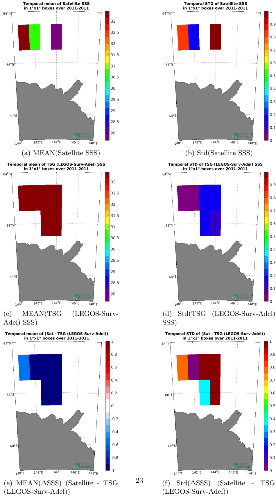
Figure 6: Temporal mean (left) and Std (right) of SSS from SMOS SSS L3 v2 - Daily - 0.5 Deg (CATDS-CECOS-IFREMER) (top), TSG (LEGOS-Surv-Adel) (middle), and of \Delta SSS (Satellite - TSG (LEGOS-Surv-Adel)). Only match-up pairs are used to generate these maps.
