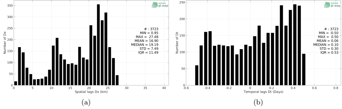
Figure 5: Histograms of the spatial (a) and temporal (b) lags between the location/time of the TSG (LEGOS-Surv-Adel) measurement and the date of the corresponding SMOS SSS L3 v2 - Daily - 0.5 Deg (CATDS-CECOS-IFREMER) SSS pixel.
