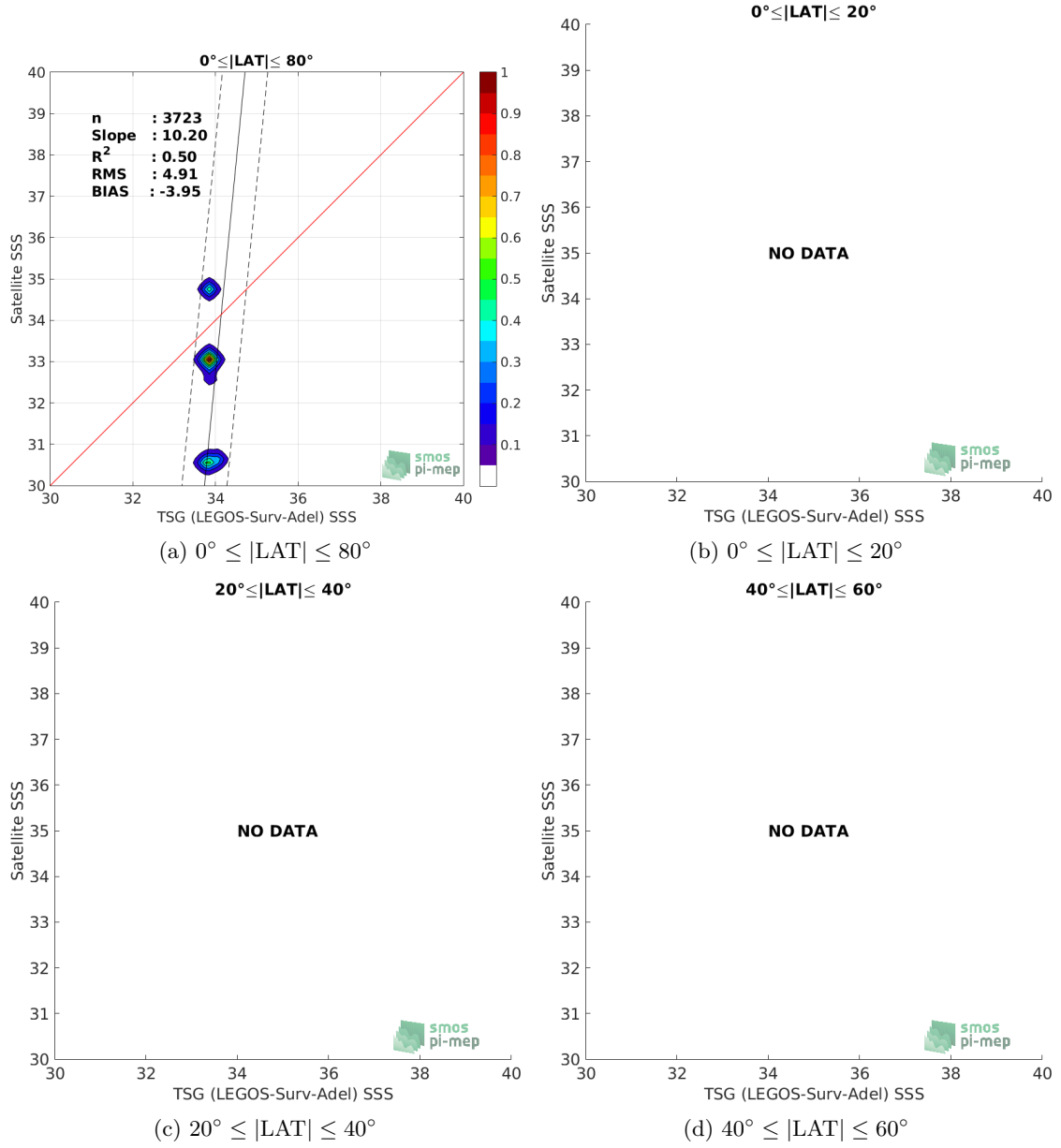
Figure 9: Contour maps of the concentration of SMOS SSS L3 v2 - Daily - 0.5 Deg (CATDS-CECOS-IFREMER) SSS (y-axis) versus TSG (LEGOS-Surv-Adel) SSS (x-axis) at match-up pairs for different latitude bands. For each plot, the red line shows x=y . The black thin and dashed lines indicate a linear fit through the data cloud and the \pm 95\% confidence levels, respectively. The number match-up pairs n , the slope and R^2 coefficient of the linear fit, the root mean square (RMS) and the mean bias between satellite and in situ data are indicated for each latitude band in each plots.
