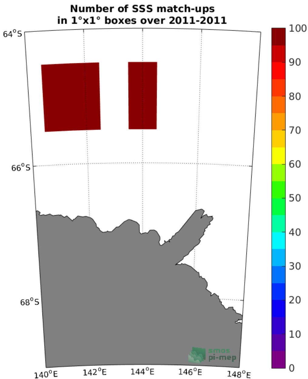
Figure 4: Number of SSS match-ups between TSG (LEGOS-Surv-Adel) SSS and the SMOS SSS L3 v2 - Daily - 0.5 Deg (CATDS-CECOS-IFREMER) SSS product for the Global Ocean Pi-MEP region over 1°x1° boxes and for the full satellite product period.
