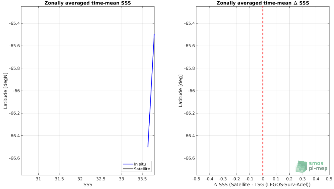
Figure 8: Left panel: Zonal mean SSS from SMOS SSS L3 v2 - Daily - 0.5 Deg (CATDS-CECOS-IFREMER) satellite product (black) and from TSG (LEGOS-Surv-Adel) (blue). Right panel: Zonal mean of \Delta SSS (Satellite - TSG (LEGOS-Surv-Adel)) for all the collected Pi-MEP match-up pairs estimated over the full satellite product period.
