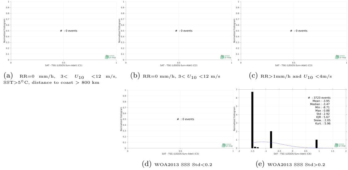
Figure 13: Normalized histogram of \Delta\text{SSS} (SMOS SSS L3 v2 - Daily - 0.5 Deg (CATDS-CECOS-IFREMER) - TSG (LEGOS-Surv-Adel)) for 5 different subdatasets corresponding to: RR=0 mm/h, 3 < U_{10} < 12 m/s, SST > 5^\circ\text{C} , distance to coast > 800 km (a), RR=0 mm/h, 3 < U_{10} < 12 m/s (b), RR > 1\text{mm/h} and U_{10} < 4\text{m/s} (c), WOA2013 SSS Std < 0.2 (d), WOA2013 SSS Std > 0.2 (e).
