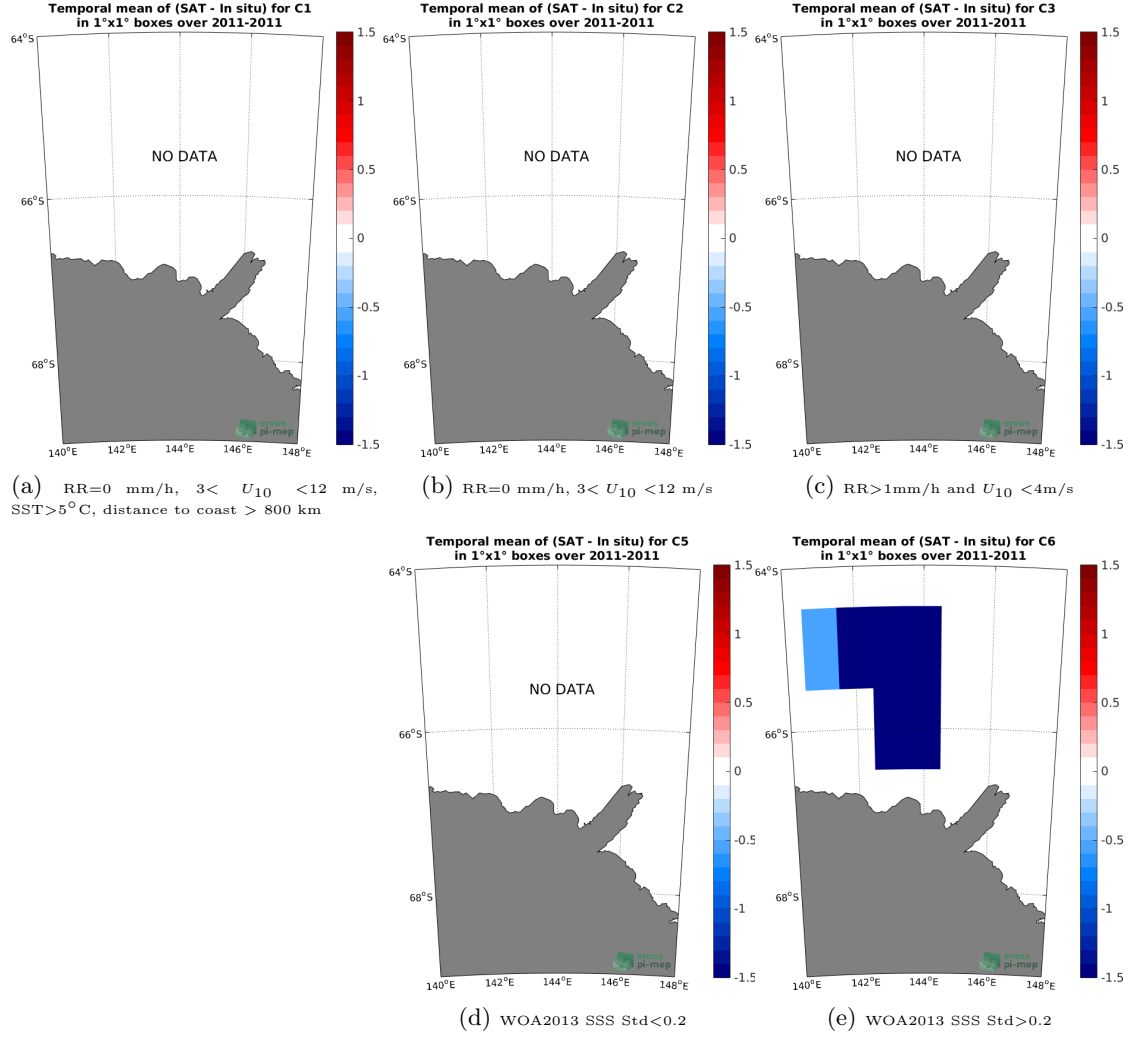
Figure 12: Temporal mean gridded over spatial boxes of size 1°x1° of \Delta\text{SSS} (SMOS SSS L3 v2 - Daily - 0.5 Deg (CATDS-CECOS-IFREMER) - TSG (LEGOS-Surv-Adel)) for 5 different subdatasets corresponding to: RR=0 mm/h, 3 < U_{10} < 12 m/s, SST > 5^\circ\text{C} , distance to coast > 800 km (a), RR=0 mm/h, 3 < U_{10} < 12 m/s (b), RR > 1 mm/h and U_{10} < 4 m/s (c), WOA2013 SSS Std < 0.2 (d), WOA2013 SSS Std > 0.2 (e).
