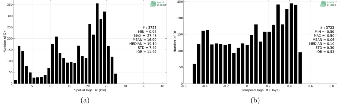
Figure 5: Histograms of the spatial (a) and temporal (b) lags between the time of the TSG (LEGOS-Surv-Adel) measurements and the date of the corresponding SMOS SSS L3 v2 - Daily - 0.5 Deg (CATDS-CECOS-IFREMER) SSS product.
