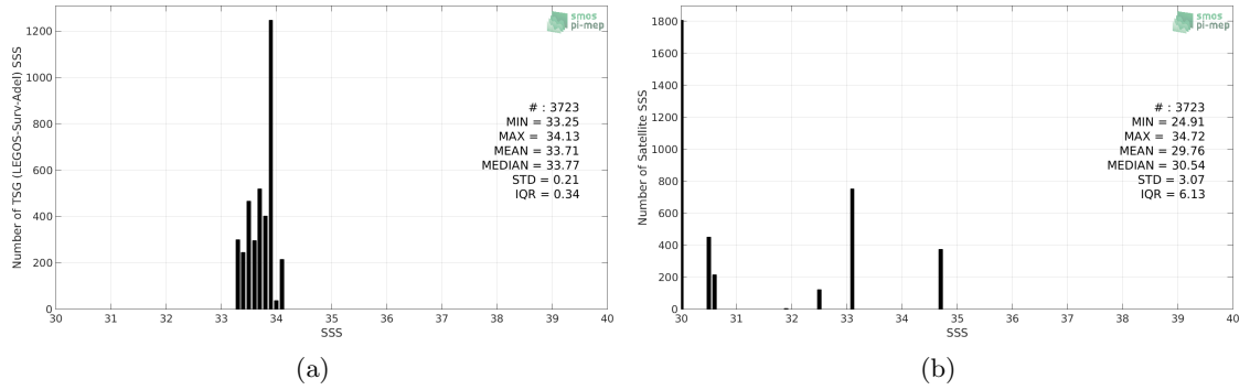
Figure 2: Histograms of SSS from TSG (LEGOS-Surv-Adel) (a) and SMOS SSS L3 v2 - Daily - 0.5 Deg (CATDS-CECOS-IFREMER) (b) considering all match-up pairs per bins of 0.1 over the Global Ocean Pi-MEP region and for the full satellite product period.
