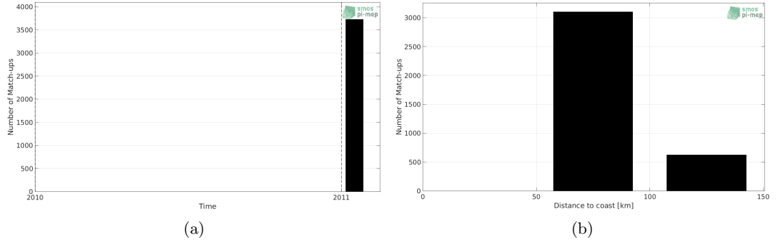
Figure 1: Number of match-ups between TSG (LEGOS-Surv-Adel) and SMOS SSS L3 v2 - Daily - 0.5 Deg (CATDS-CECOS-IFREMER) SSS as a function of time (a) and as function of the distance to coast (b) over the Global Ocean Pi-MEP region and for the full satellite product period.
