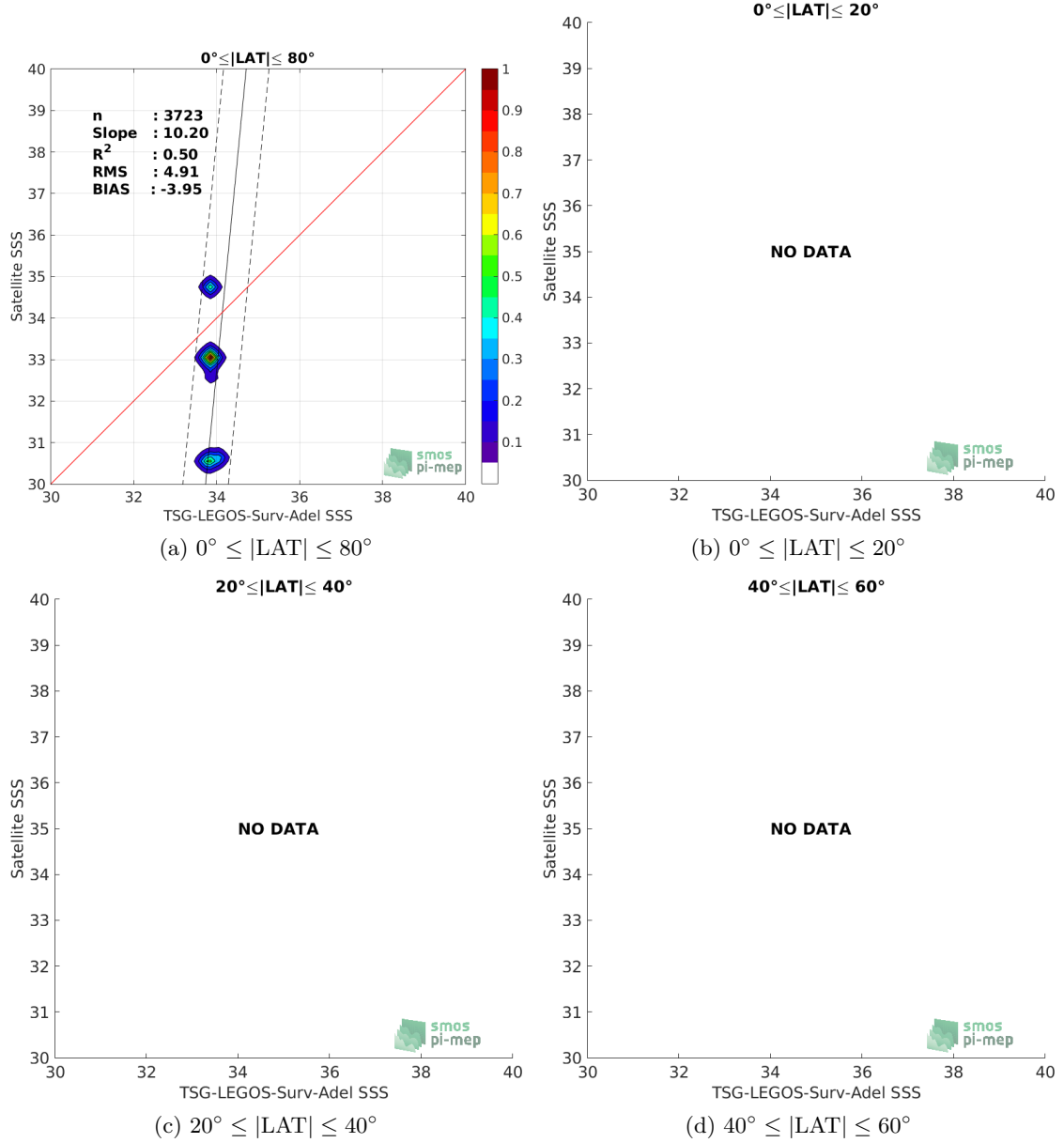
Figure 9: Contour maps of the concentration of SMOS-L3-CATDS-CECOS-IFREMER-V2-1DAY-0.5DEG SSS (y-axis) versus TSG-LEGOS-Surv-Adel SSS (x-axis) at match-up pairs for different latitude bands. For each plot, the red line shows x=y . The black thin and dashed lines indicate a linear fit through the data cloud and the \pm 95\% confidence levels, respectively. The number match-up pairs n , the slope and R^2 coefficient of the linear fit, the root mean square (RMS) and the mean bias between satellite and in situ data are indicated for each latitude band in each plots.
