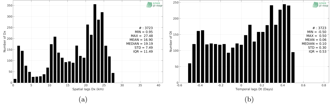
Figure 5: Histograms of the spatial (a) and temporal (b) lags between the time of the TSG-LEGOS-Surv-Adel measurements and the date of the corresponding SMOS-L3-CATDS-CECOS-IFREMER-V2-1DAY-0.5DEG SSS product.
