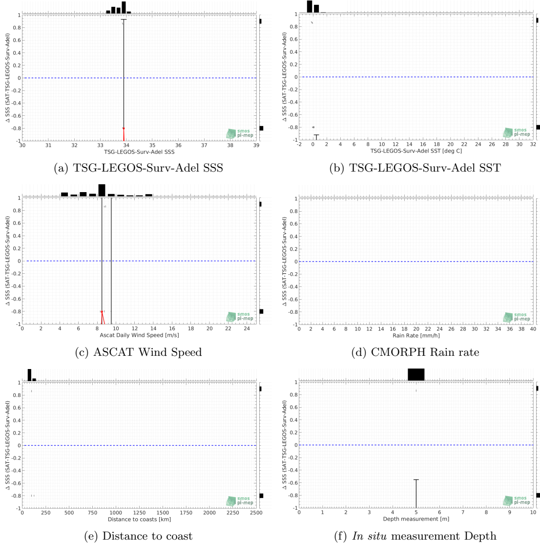
Figure 11: \Delta SSS (Satellite - TSG-LEGOS-Surv-Adel) sorted as function of TSG-LEGOS-Surv-Adel SSS values a), TSG-LEGOS-Surv-Adel SST b), ASCAT Wind speed c), CMORPH rain rate d), distance to coast (e) and in situ measurement depth (f). In all plots the median and Std of \Delta SSS for each bin is indicated by the red curves and black vertical thick bars ( \pm 1 Std)
