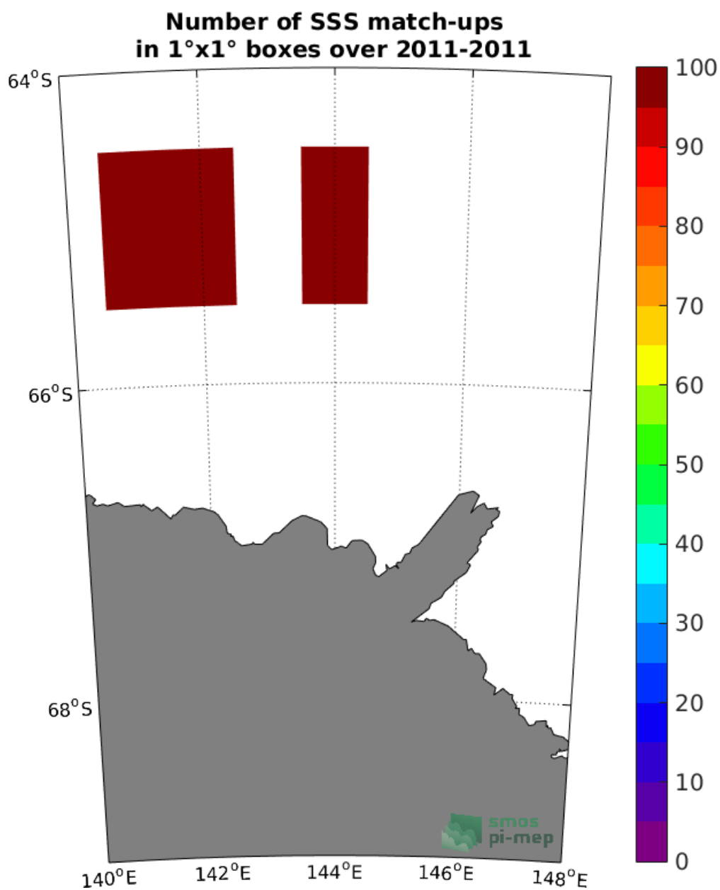
Figure 4: Number of SSS match-ups between TSG-LEGOS-Surv-Adel SSS and the SMOS-L3-CATDS-CECOS-IFREMER-V2-1DAY-0.5DEG SSS product for the Global Ocean Pi-MEP region over 1°x1° boxes and for the full satellite product period.
