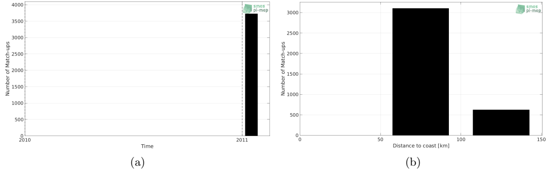
Figure 1: Number of match-ups between TSG-LEGOS-Surv-Adel and SMOS-L3-CATDS-CECOS-IFREMER-V2-1DAY-0.5DEG SSS as a function of time (a) and as function of the distance to coast (b) over the Global Ocean Pi-MEP region and for the full satellite product period.
