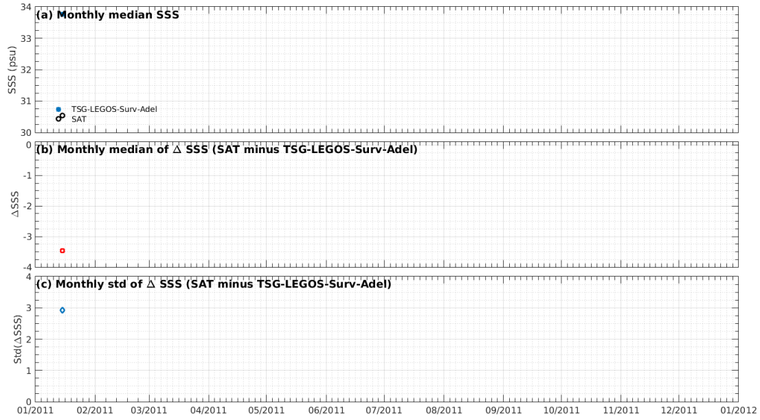
Figure 7: Time series of the monthly median SSS (top), median of \Delta SSS (Satellite - TSG-LEGOS-Surv-Adel) and Std of \Delta SSS (Satellite - TSG-LEGOS-Surv-Adel) over the Global Ocean Pi-MEP region considering all match-ups collected by the Pi-MEP.
