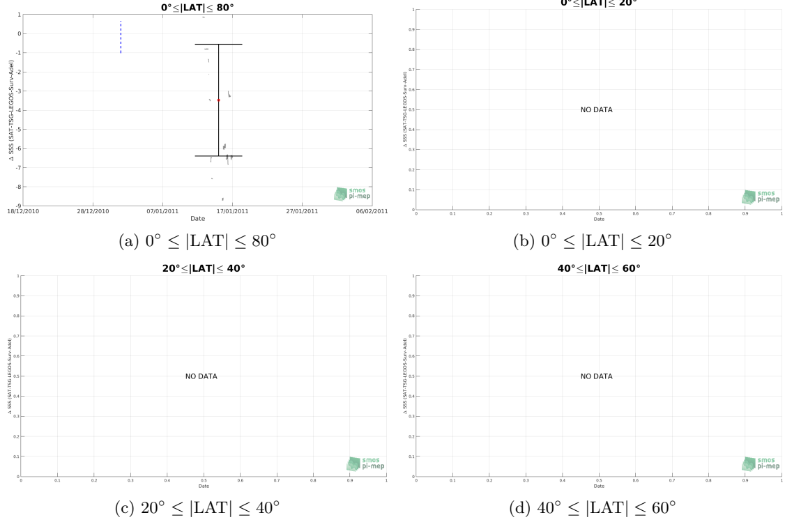
Figure 10: Monthly median (red curves) of \Delta SSS (Satellite - TSG-LEGOS-Surv-Adel) and \pm 1 Std (black vertical thick bars) as function of time for all the collected Pi-MEP match-up pairs estimated over the Global Ocean Pi-MEP region and for the full satellite product period are shown for different latitude bands: (a) 80^\circ\text{S}-80^\circ\text{N} , (b) 20^\circ\text{S}-20^\circ\text{N} , (c) 40^\circ\text{S}-20^\circ\text{S} and 20^\circ\text{N}-40^\circ\text{N} and (d) 60^\circ\text{S}-40^\circ\text{S} and 40^\circ\text{N}-60^\circ\text{N} .
