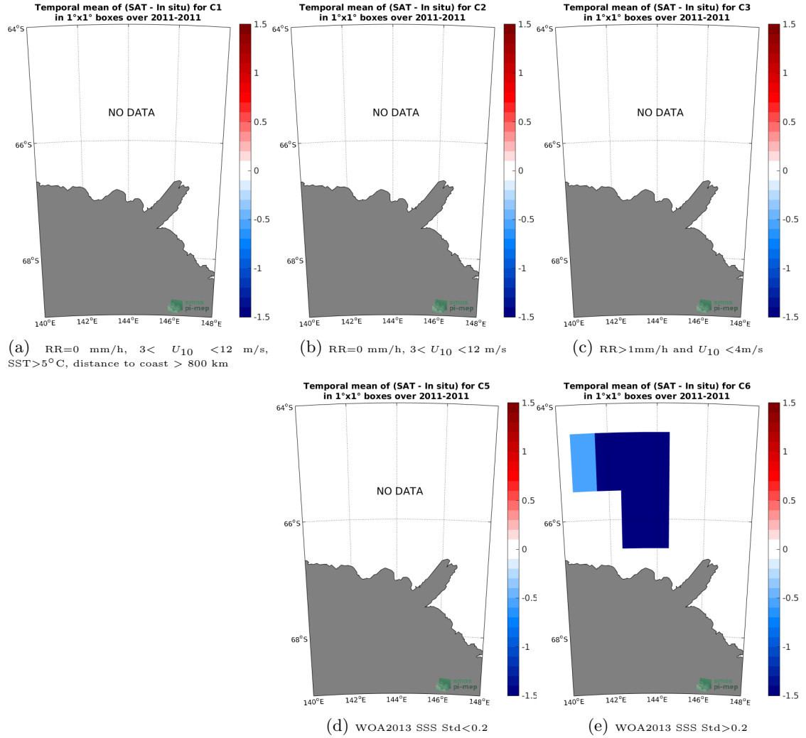
Figure 12: Temporal mean gridded over spatial boxes of size 1^\circ \times 1^\circ of \Delta SSS (SMOS-L3-CATDS-CECOS-IFREMER-V2-1DAY-0.5DEG - TSG-LEGOS-Surv-Adel) for 5 different subdatasets corresponding to: RR=0 mm/h, 3 < U_{10} < 12 m/s, SST >5^\circ\text{C} , distance to coast > 800 km (a), RR=0 mm/h, 3 < U_{10} < 12 m/s (b), RR >1 mm/h and U_{10} < 4 m/s (c), WOA2013 SSS Std <0.2 (d), WOA2013 SSS Std >0.2 (e).
