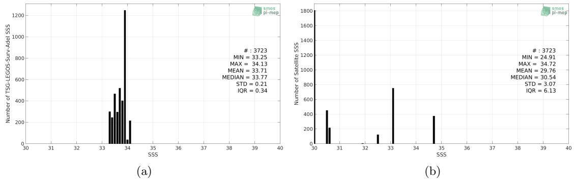
Figure 2: Histograms of SSS from TSG-LEGOS-Surv-Adel (a) and SMOS-L3-CATDS-CECOS-IFREMER-V2-1DAY-0.5DEG (b) considering all match-up pairs per bins of 0.1 over the Global Ocean Pi-MEP region and for the full satellite product period.
