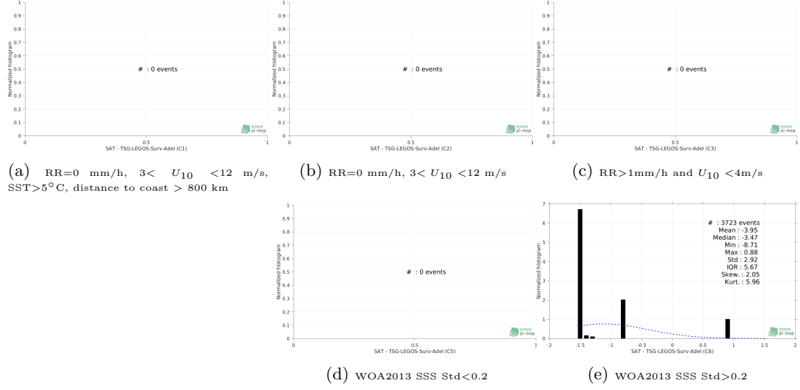
Figure 13: Normalized histogram of \Delta\text{SSS} (SMOS-L3-CATDS-CECOS-IFREMER-V2-1DAY-0.5DEG - TSG-LEGOS-Surv-Adel) for 5 different subdatasets corresponding to: RR=0 mm/h, 3 < U_{10} < 12 m/s, SST > 5^\circ\text{C} , distance to coast > 800 km (a), RR=0 mm/h, 3 < U_{10} < 12 m/s (b), RR > 1\text{mm/h} and U_{10} < 4\text{m/s} (c), WOA2013 SSS Std < 0.2 (d), WOA2013 SSS Std > 0.2 (e).
