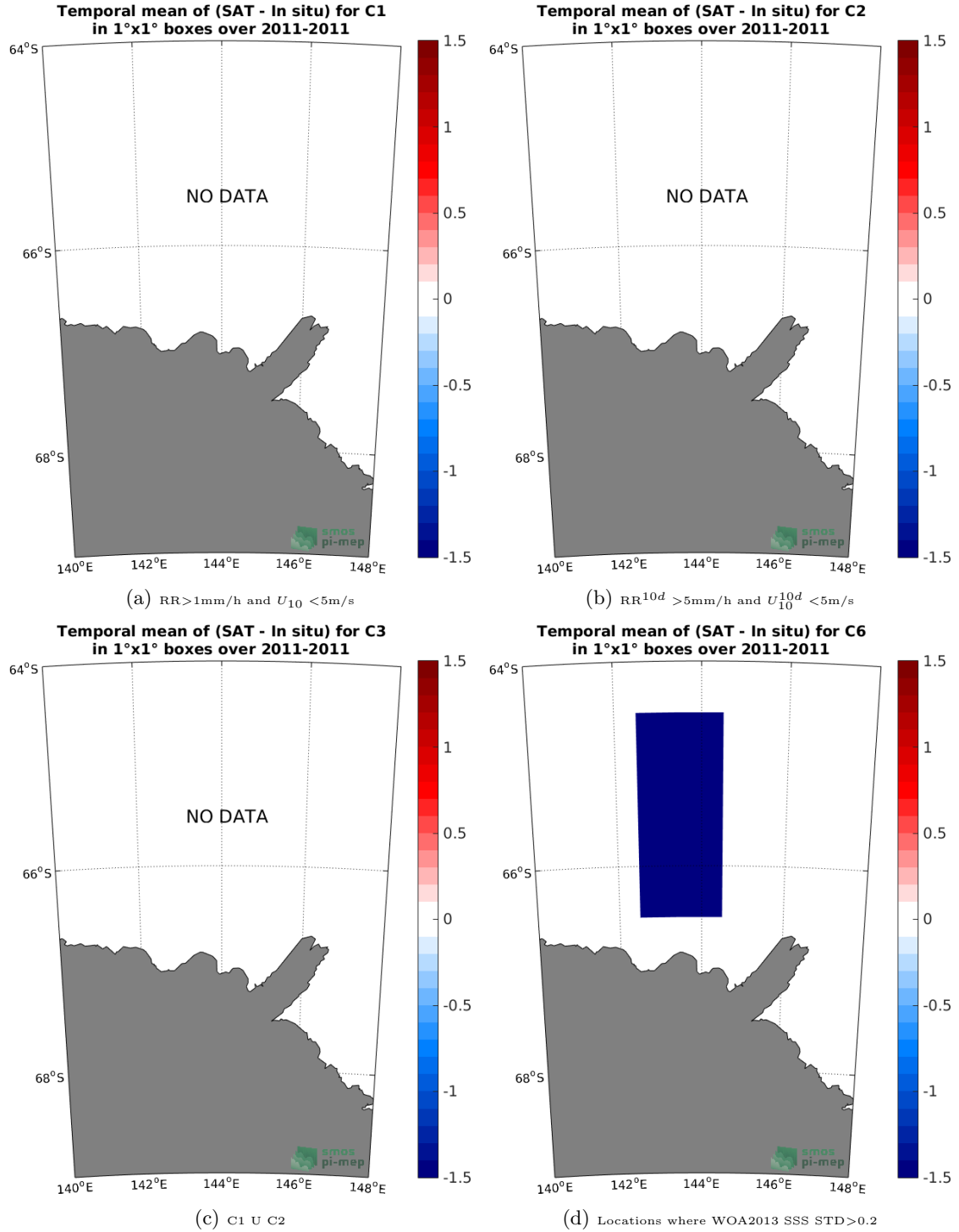
Figure 12: Temporal mean gridded over spatial boxes of size 1^\circ \times 1^\circ of \Delta\text{SSS} (SMOS-L3-CATDS-CECOS-IFREMER-V2-1DAY-0.5DEG - TSG-LEGOS-Surv-Adel) for 4 different subdatasets corresponding to: RR > 1\text{mm/h} and U_{10} < 5\text{m/s} (a), RR^{10d} > 5\text{mm/h} and U_{10}^{10d} < 5\text{m/s} (b), C1 U C2 (c), Locations where WOA2013 SSS STD > 0.2 (d).
