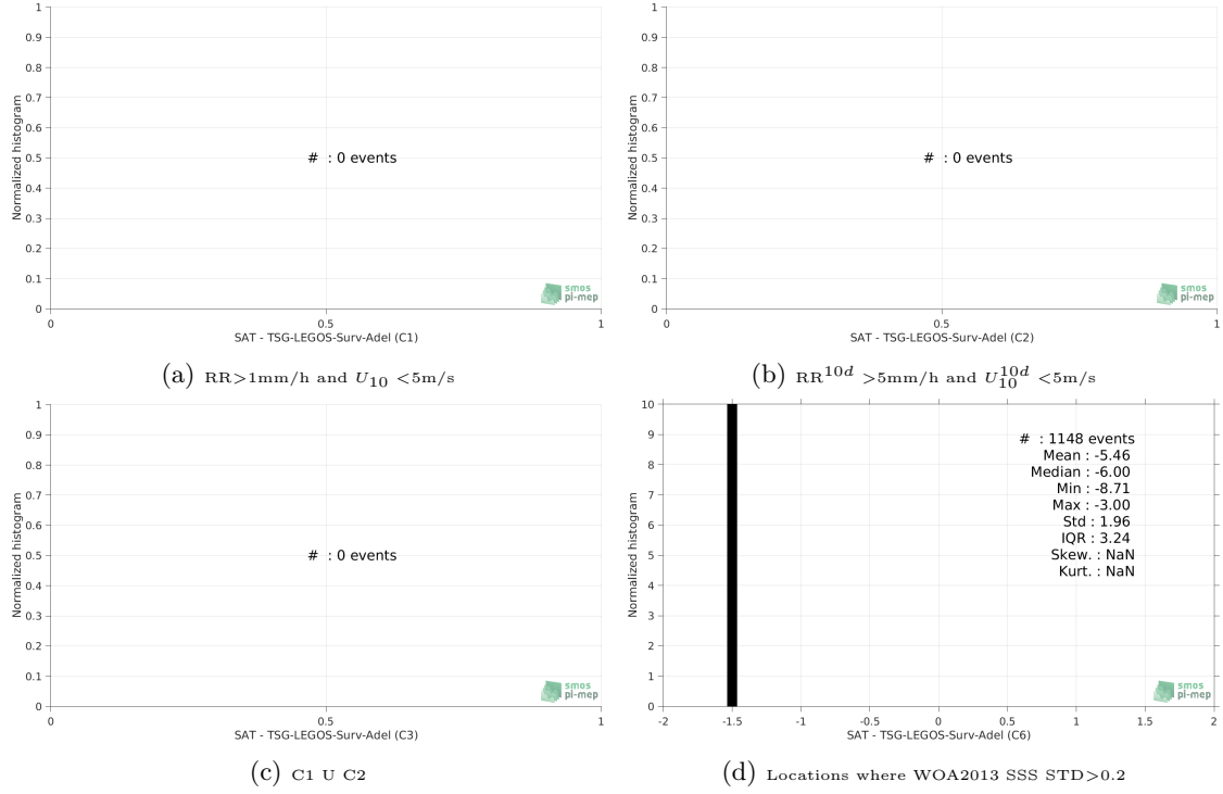
Figure 13: Normalized histogram of \Delta\text{SSS} (SMOS-L3-CATDS-CECOS-IFREMER-V2-1DAY-0.5DEG - TSG-LEGOS-Surv-Adel) for 6 different subdatasets corresponding to: RR > 1\text{mm/h} and U_{10} < 5\text{m/s} (a), RR^{10d} > 5\text{mm/h} and U_{10}^{10d} < 5\text{m/s} (b), C1 \cup C2 (c), Locations where WOA2013 SSS STD > 0.2 (d).
