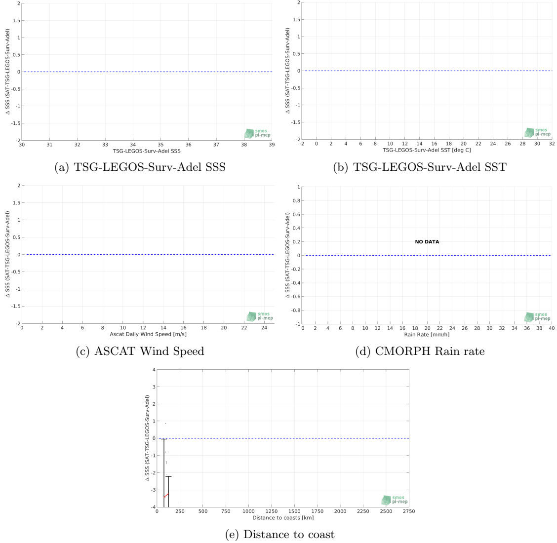
Figure 11: \Delta SSS (Satellite - TSG-LEGOS-Surv-Adel) sorted as function of TSG-LEGOS-Surv-Adel SSS values a), TSG-LEGOS-Surv-Adel SST b), ASCAT Wind speed c), CMORPH rain rate d) and distance to coast (e). In all plots the mean and STD of \Delta SSS for each bin is indicated by the red curves and black vertical thick bars ( \pm 1 STD)
