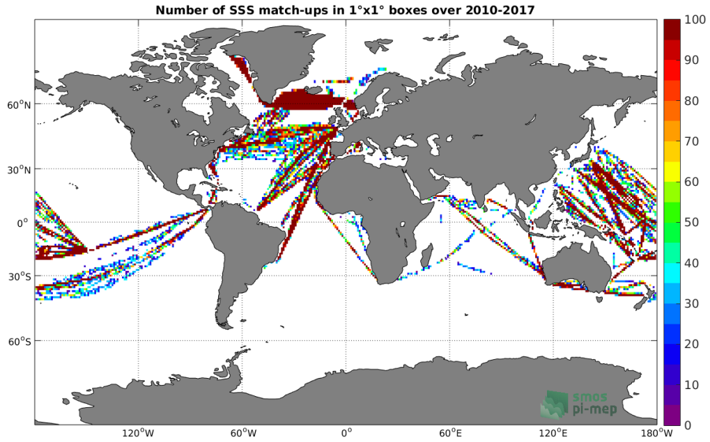
Figure 4: Number of SSS match-ups between TSG (LEGOS-DM) SSS and the SMOS SSS L3 v2 - Daily - 0.5 Deg (CATDS-CECOS-IFREMER) SSS product for the Global Ocean Pi-MEP region over 1^\circ \times 1^\circ boxes and for the full satellite product period.
