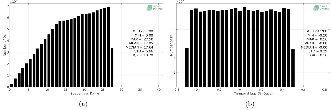
Figure 5: Histograms of the spatial (a) and temporal (b) lags between the time of the TSG (LEGOS-DM) measurements and the date of the corresponding SMOS SSS L3 v2 - Daily - 0.5 Deg (CATDS-CECOS-IFREMER) SSS product.
