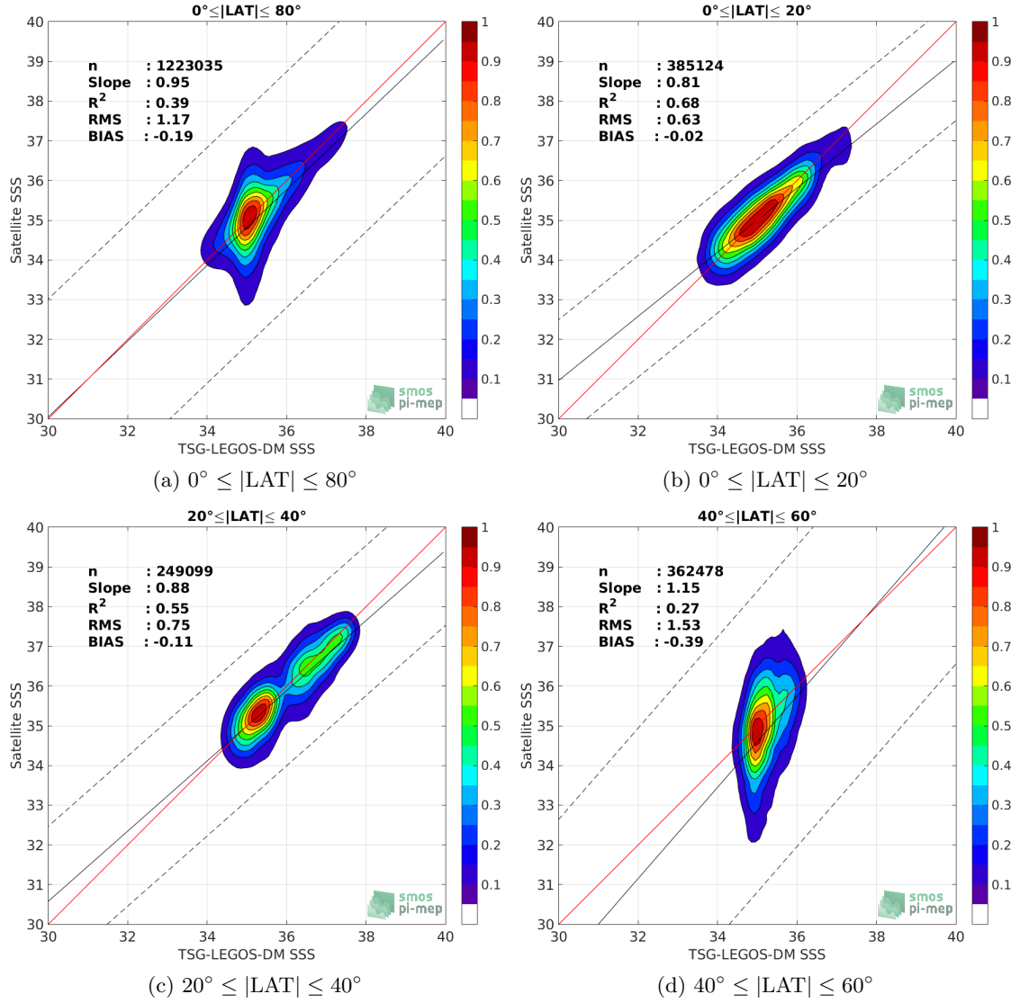
Figure 9: Contour maps of the concentration of SMOS-L3-CATDS-CECOS-IFREMER-V2-1DAY-0.5DEG SSS (y-axis) versus TSG-LEGOS-DM SSS (x-axis) at match-up pairs for different latitude bands. For each plot, the red line shows x=y . The black thin and dashed lines indicate a linear fit through the data cloud and the \pm 95\% confidence levels, respectively. The number match-up pairs n , the slope and R^2 coefficient of the linear fit, the root mean square (RMS) and the mean bias between satellite and in situ data are indicated for each latitude band in each plots.
