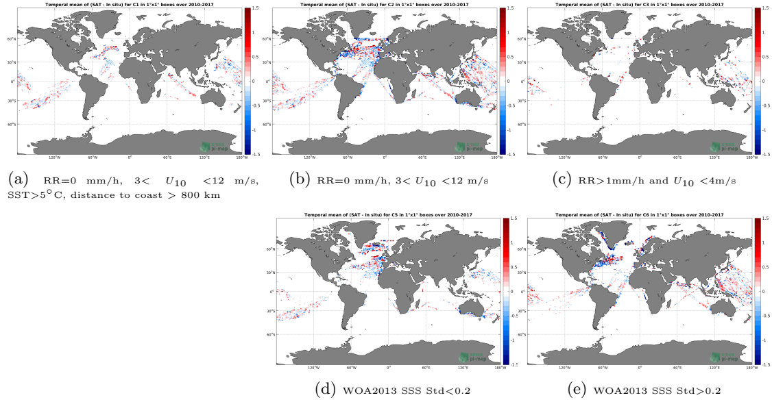
Figure 12: Temporal mean gridded over spatial boxes of size 1^\circ \times 1^\circ of \Delta SSS (SMOS-L3-CATDS-CECOS-IFREMER-V2-1DAY-0.5DEG - TSG-LEGOS-DM) for 5 different subdatasets corresponding to: RR=0 mm/h, 3 < U_{10} < 12 m/s, SST >5^\circ C, distance to coast > 800 km (a), RR=0 mm/h, 3 < U_{10} < 12 m/s (b), RR >1 mm/h and U_{10} < 4 m/s (c), WOA2013 SSS Std <0.2 (d), WOA2013 SSS Std >0.2 (e).
