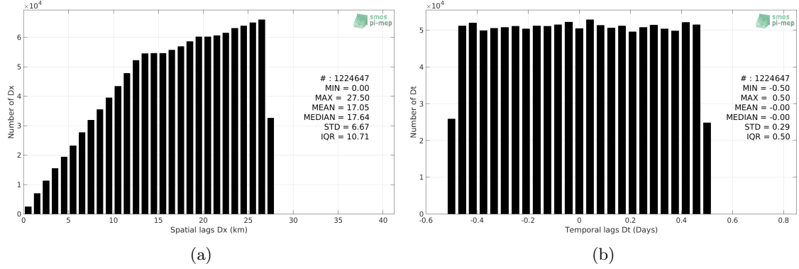
Figure 5: Histograms of the spatial (a) and temporal (b) lags between the time of the TSG-LEGOS-DM measurements and the date of the corresponding SMOS-L3-CATDS-CECOS-IFREMER-V2-1DAY-0.5DEG SSS product.
