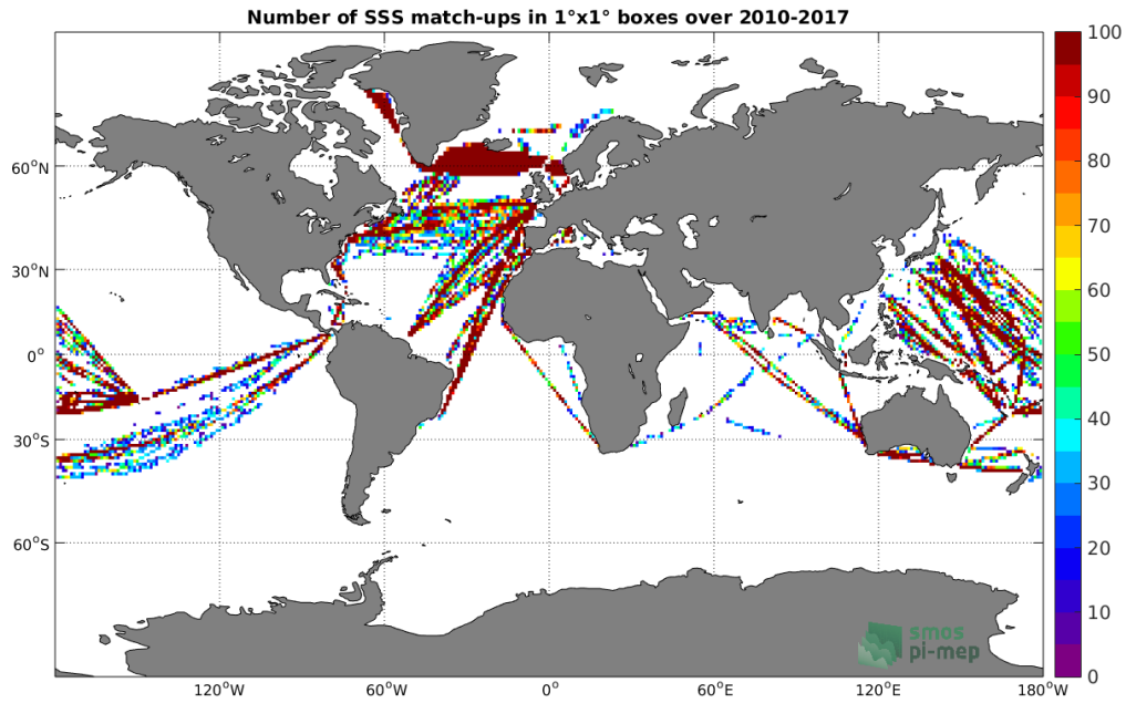
Figure 4: Number of SSS match-ups between TSG-LEGOS-DM SSS and the SMOS-L3-CATDS-CECOS-IFREMER-V2-1DAY-0.5DEG SSS product for the Global Ocean Pi-MEP region over 1°x1° boxes and for the full satellite product period.
