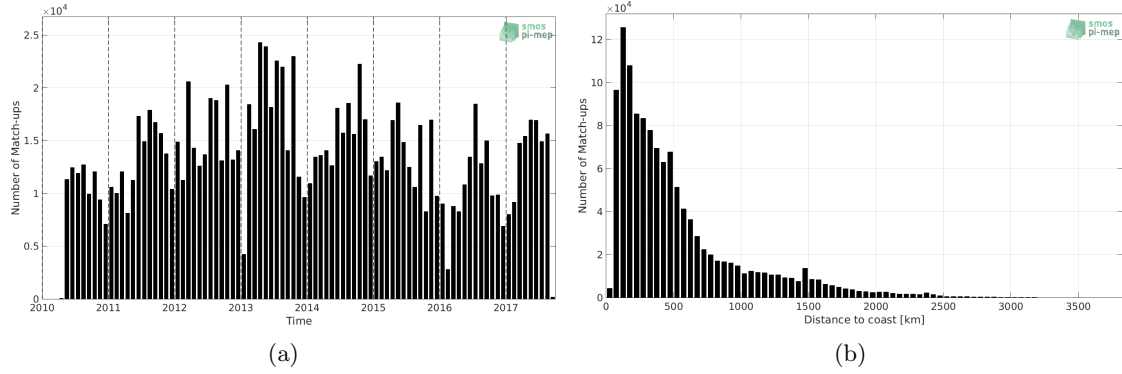
Figure 1: Number of match-ups between TSG-LEGOS-DM and SMOS-L3-CATDS-CECOS-IFREMER-V2-1DAY-0.5DEG SSS as a function of time (a) and as function of the distance to coast (b) over the Global Ocean Pi-MEP region and for the full satellite product period.
