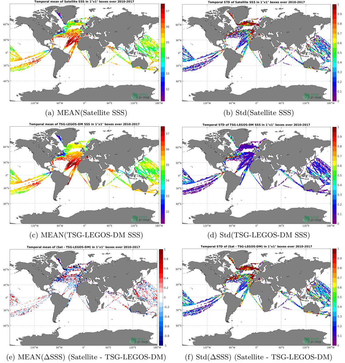
Figure 6: Temporal mean (left) and Std (right) of SSS from SMOS-L3-CATDS-CECOS-IFREMER-V2-1DAY-0.5DEG (top), TSG-LEGOS-DM (middle), and of \Delta SSS (Satellite - TSG-LEGOS-DM). Only match-up pairs are used to generate these maps.
