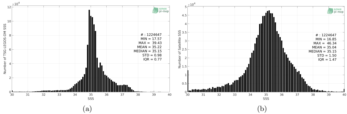
Figure 2: Histograms of SSS from TSG-LEGOS-DM (a) and SMOS-L3-CATDS-CECOS-IFREMER-V2-1DAY-0.5DEG (b) considering all match-up pairs per bins of 0.1 over the Global Ocean Pi-MEP region and for the full satellite product period.
