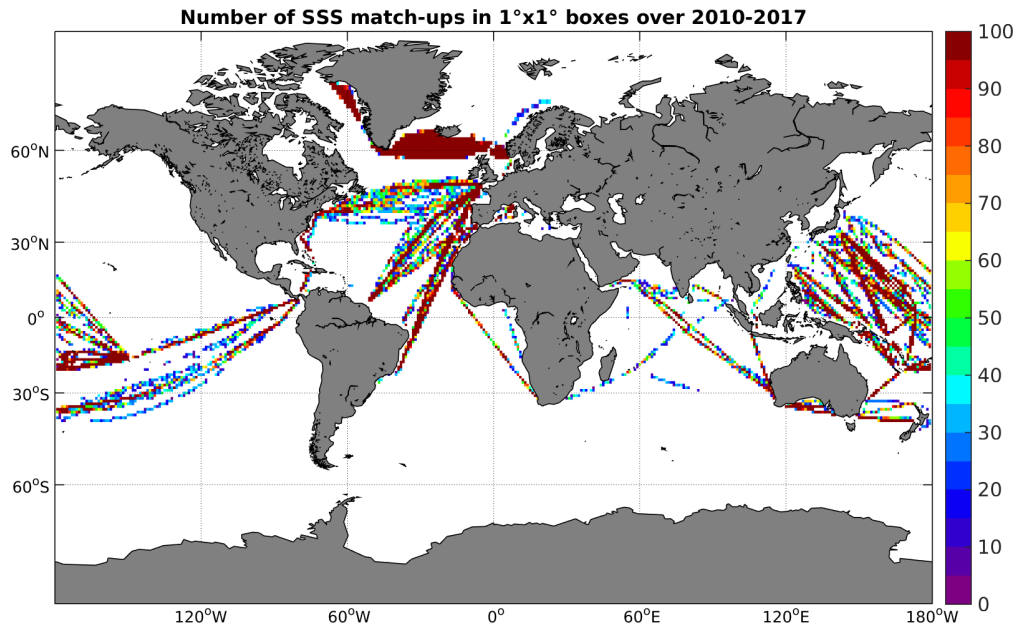
Figure 4: Number of SSS match-ups between TSG-LEGOS-DM SSS and the SMOS-L3-CATDS-CECOS-IFREMER-V2-1DAY-0.5DEG SSS product for the Global Ocean Pi-MEP region over 1^\circ \times 1^\circ boxes and for the full satellite product period.
