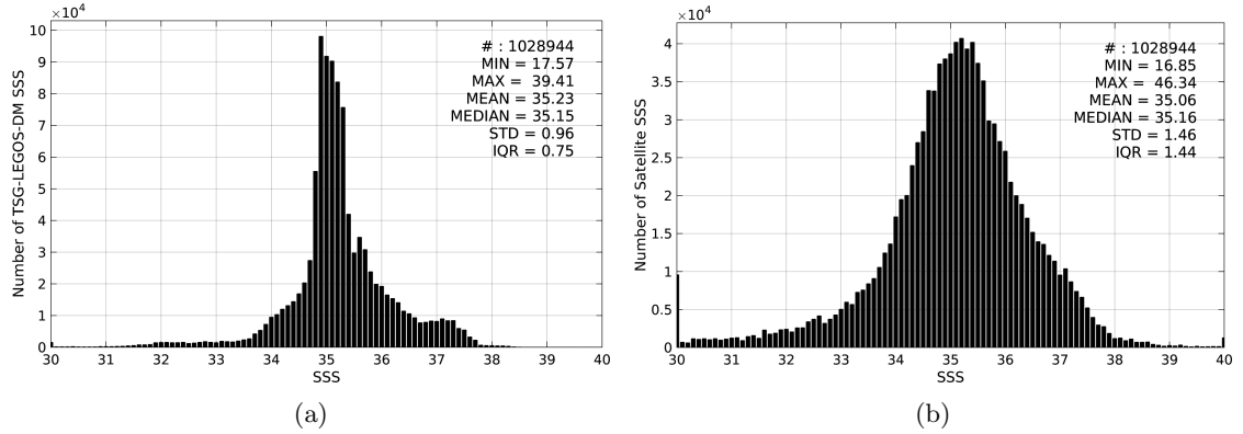
Figure 2: Histograms of SSS from TSG-LEGOS-DM (a) and SMOS-L3-CATDS-CECOS-IFREMER-V2-1DAY-0.5DEG (b) considering all match-up pairs per bins of 0.1 over the Global Ocean Pi-MEP region and for the full satellite product period.
