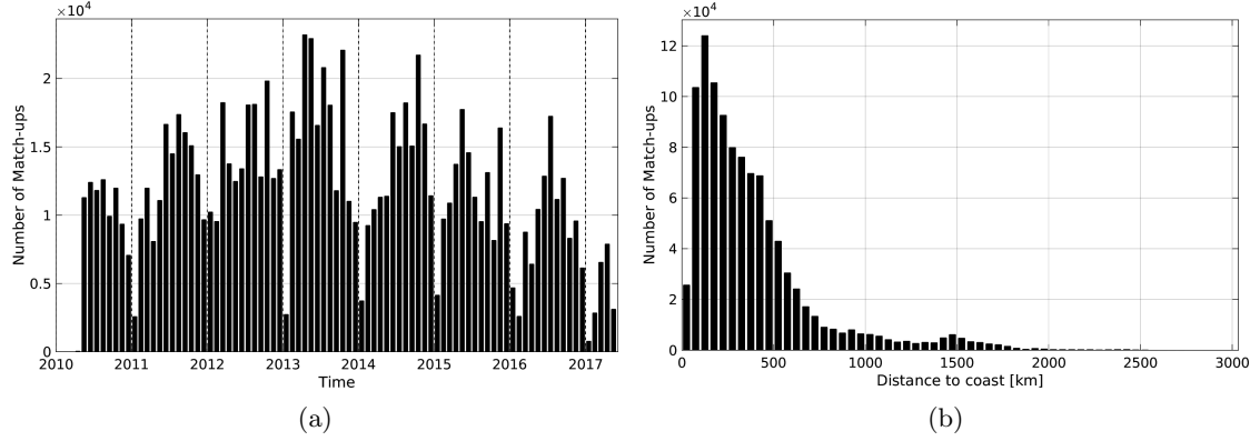
Figure 1: Number of match-ups between TSG-LEGOS-DM and SMOS-L3-CATDS-CECOS-IFREMER-V2-1DAY-0.5DEG SSS as a function of time (a) and as function of the distance to coast (b) over the Global Ocean Pi-MEP region and for the full satellite product period.
