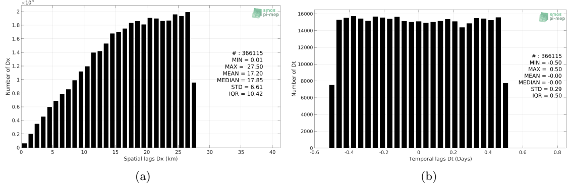
Figure 5: Histograms of the spatial (a) and temporal (b) lags between the time of the TSG (GOSUD-Sailing-ship) measurements and the date of the corresponding SMOS SSS L3 v2 - Daily - 0.5 Deg (CATDS-CECOS-IFREMER) SSS product.
