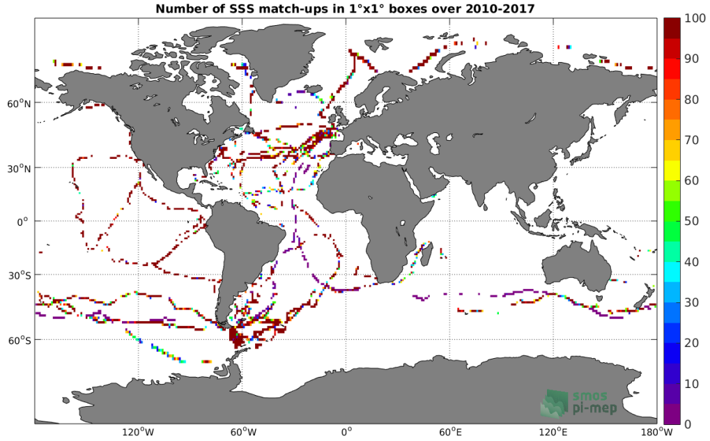
Figure 4: Number of SSS match-ups between TSG (GOSUD-Sailing-ship) SSS and the SMOS SSS L3 v2 - Daily - 0.5 Deg (CATDS-CECOS-IFREMER) SSS product for the Global Ocean Pi-MEP region over 1^\circ \times 1^\circ boxes and for the full satellite product period.
