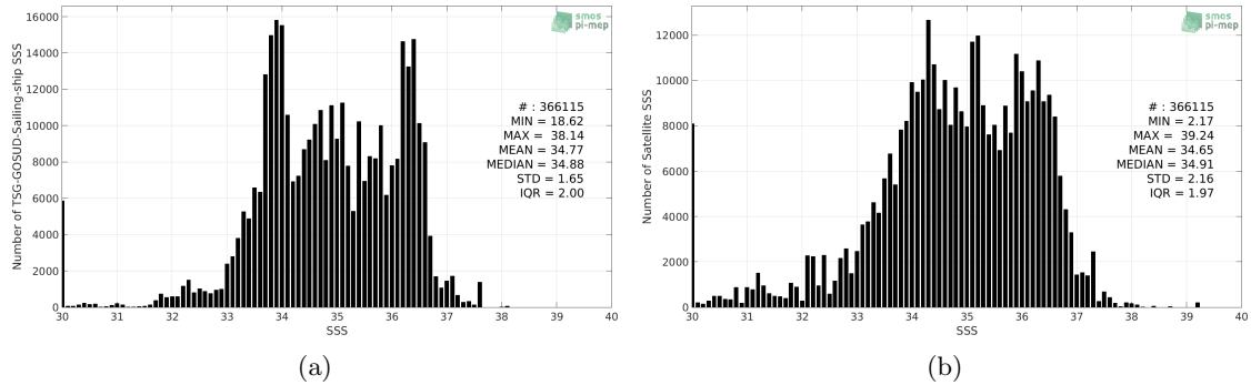
Figure 2: Histograms of SSS from TSG-GOSUD-Sailing-ship (a) and SMOS L3 v2 - Daily - 0.5 Deg (CATDS-CECOS-IFREMER) (b) considering all match-up pairs per bins of 0.1 over the Global Ocean Pi-MEP region and for the full satellite product period.
