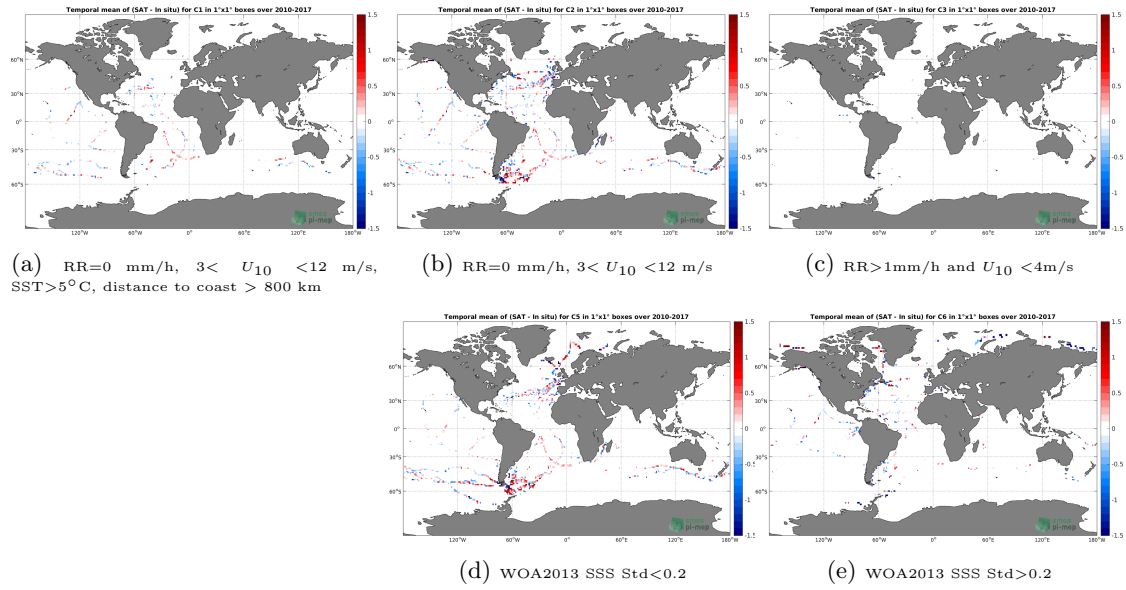
Figure 12: Temporal mean gridded over spatial boxes of size 1^\circ \times 1^\circ of \Delta SSS (SMOS L3 v2 - Daily - 0.5 Deg (CATDS-CECOS-IFREMER) - TSG-GOSUD-Sailing-ship) for 5 different subdatasets corresponding to:RR=0 mm/h, 3 < U_{10} < 12 m/s, SST >5^\circ\text{C} , distance to coast > 800 km (a), RR=0 mm/h, 3 < U_{10} < 12 m/s (b), RR >1 mm/h and U_{10} < 4 m/s (c), WOA2013 SSS Std <0.2 (d), WOA2013 SSS Std >0.2 (e).
