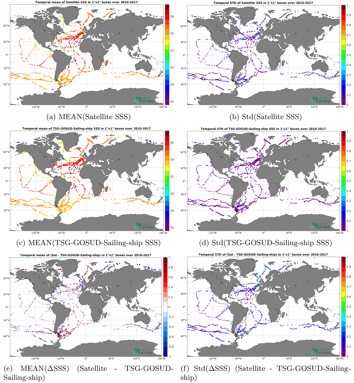
Figure 6: Temporal mean (left) and Std (right) of SSS from SMOS L3 v2 - Daily - 0.5 Deg (CATDS-CECOS-IFREMER) (top), TSG-GOSUD-Sailing-ship (middle), and of \Delta SSS (Satellite - TSG-GOSUD-Sailing-ship). Only match-up pairs are used to generate these maps.
