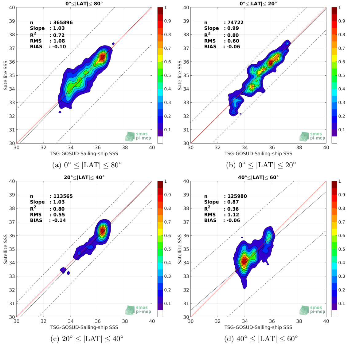
Figure 9: Contour maps of the concentration of SMOS L3 v2 - Daily - 0.5 Deg (CATDS-CECOS-IFREMER) SSS (y-axis) versus TSG-GOSUD-Sailing-ship SSS (x-axis) at match-up pairs for different latitude bands. For each plot, the red line shows x=y . The black thin and dashed lines indicate a linear fit through the data cloud and the \pm 95\% confidence levels, respectively. The number match-up pairs n , the slope and R^2 coefficient of the linear fit, the root mean square (RMS) and the mean bias between satellite and in situ data are indicated for each latitude band in each plots.
