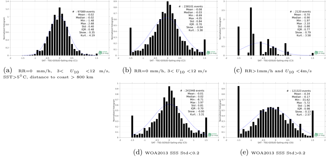
Figure 13: Normalized histogram of \Delta SSS (SMOS L3 v2 - Daily - 0.5 Deg (CATDS-CECOS-IFREMER) - TSG-GOSUD-Sailing-ship) for 5 different subdatasets corresponding to: RR=0 mm/h, 3 < U_{10} < 12 m/s, SST>5°C, distance to coast > 800 km (a), RR=0 mm/h, 3 < U_{10} < 12 m/s (b), RR>1 mm/h and U_{10} < 4 m/s (c), WOA2013 SSS Std<0.2 (d), WOA2013 SSS Std>0.2 (e).
