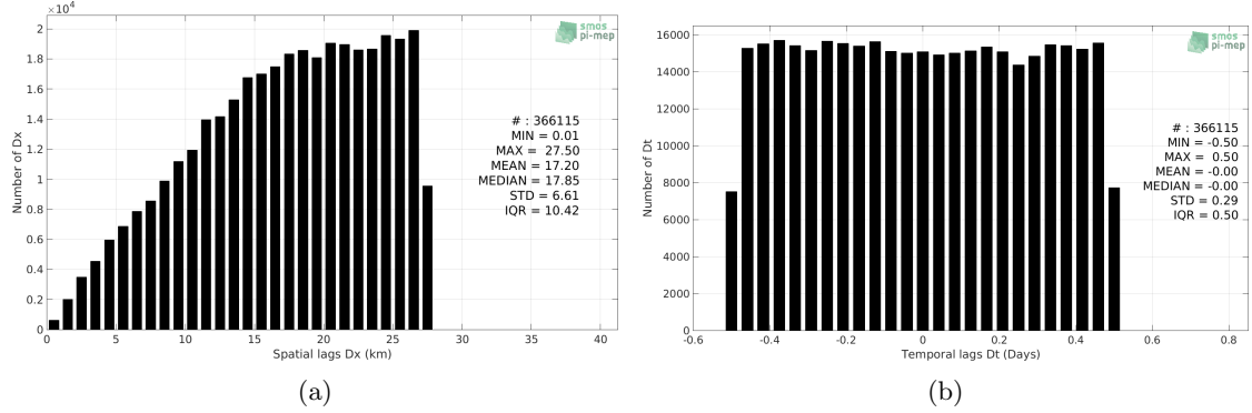
Figure 5: Histograms of the spatial (a) and temporal (b) lags between the time of the TSG-GOSUD-Sailing-ship measurements and the date of the corresponding SMOS L3 v2 - Daily - 0.5 Deg (CATDS-CECOS-IFREMER) SSS product.
