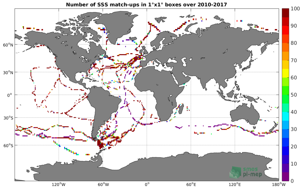
Figure 4: Number of SSS match-ups between TSG-GOSUD-Sailing-ship SSS and the SMOS L3 v2 - Daily - 0.5 Deg (CATDS-CECOS-IFREMER) SSS product for the Global Ocean Pi-MEP region over 1°x1° boxes and for the full satellite product period.
