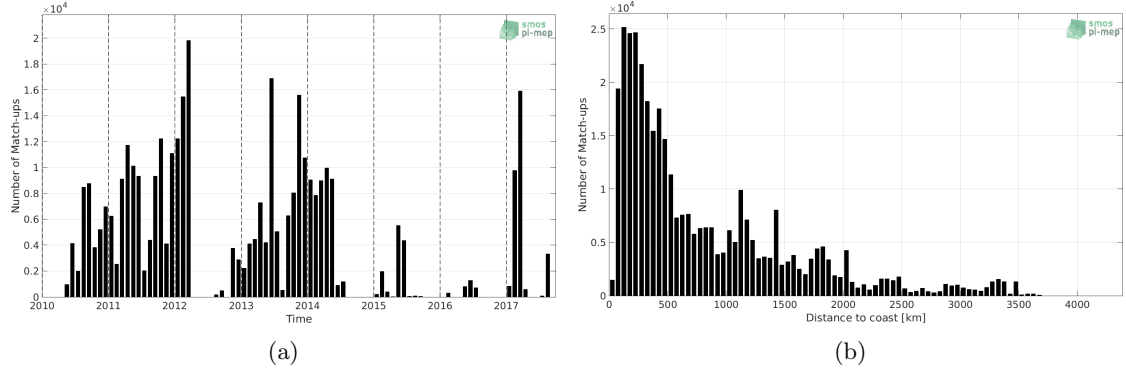
Figure 1: Number of match-ups between TSG-GOSUD-Sailing-ship and SMOS L3 v2 - Daily - 0.5 Deg (CATDS-CECOS-IFREMER) SSS as a function of time (a) and as function of the distance to coast (b) over the Global Ocean Pi-MEP region and for the full satellite product period.
