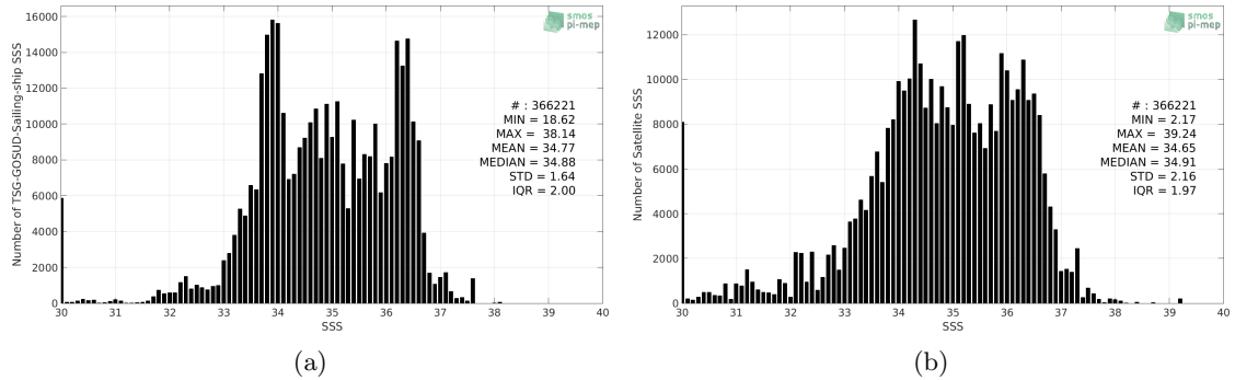
Figure 2: Histograms of SSS from TSG-GOSUD-Sailing-ship (a) and SMOS-L3-CATDS-CECOS-IFREMER-V2-1DAY-0.5DEG (b) considering all match-up pairs per bins of 0.1 over the Global Ocean Pi-MEP region and for the full satellite product period.
