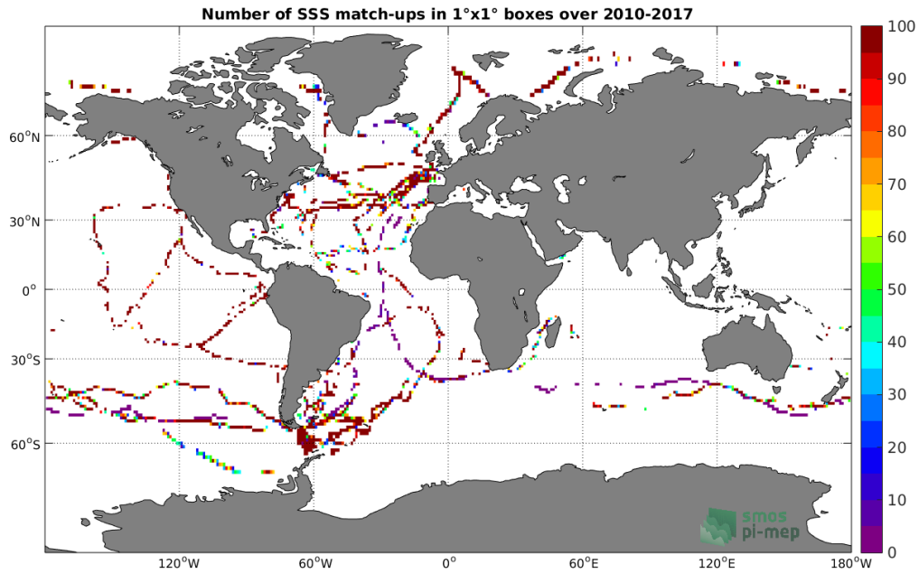
Figure 4: Number of SSS match-ups between TSG-GOSUD-Sailing-ship SSS and the SMOS-L3-CATDS-CECOS-IFREMER-V2-1DAY-0.5DEG SSS product for the Global Ocean Pi-MEP region over 1^\circ \times 1^\circ boxes and for the full satellite product period.
