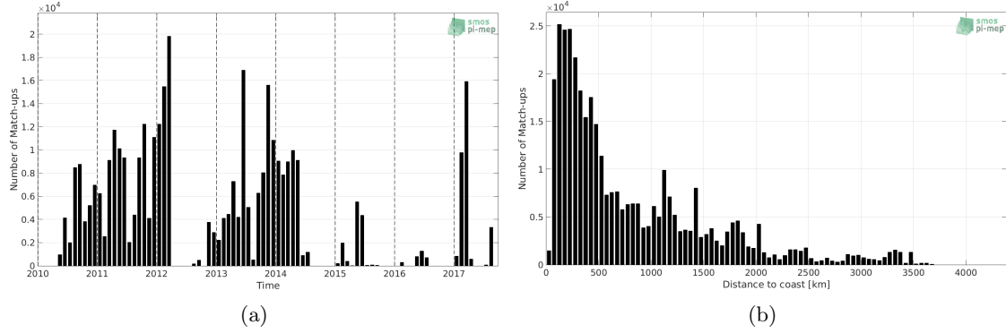
Figure 1: Number of match-ups between TSG-GOSUD-Sailing-ship and SMOS-L3-CATDS-CECOS-IFREMER-V2-1DAY-0.5DEG SSS as a function of time (a) and as function of the distance to coast (b) over the Global Ocean Pi-MEP region and for the full satellite product period.
