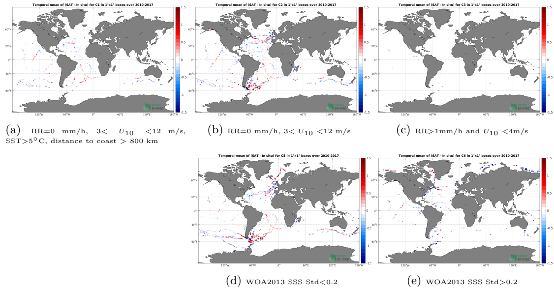
Figure 12: Temporal mean gridded over spatial boxes of size 1^\circ \times 1^\circ of \Delta SSS (SMOS-L3-CATDS-CECOS-IFREMER-V2-1DAY-0.5DEG - TSG-GOSUD-Sailing-ship) for 5 different subdatasets corresponding to:RR=0 mm/h, 3 < U_{10} < 12 m/s, SST>5°C, distance to coast > 800 km (a), RR=0 mm/h, 3 < U_{10} < 12 m/s (b), RR>1mm/h and U_{10} < 4 m/s (c), WOA2013 SSS Std<0.2 (d), WOA2013 SSS Std>0.2 (e).
