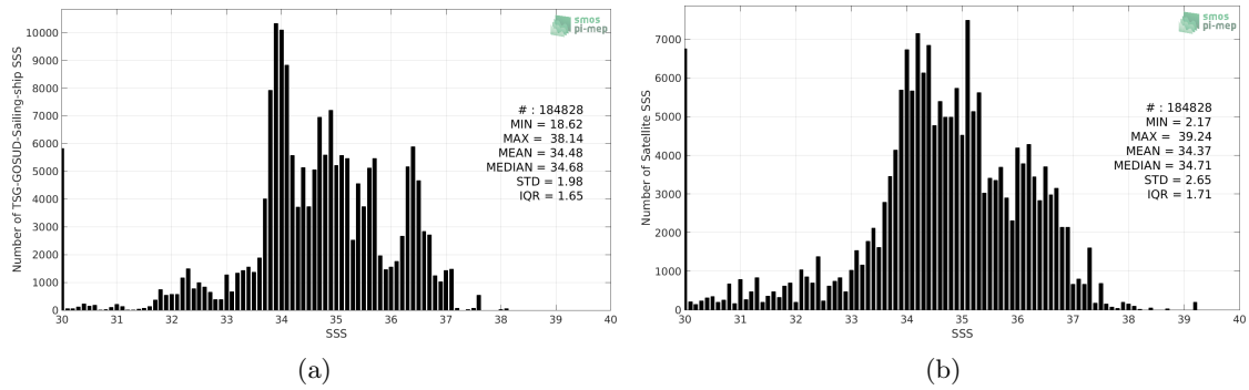
Figure 2: Histograms of SSS from TSG-GOSUD-Sailing-ship (a) and SMOS-L3-CATDS-CECOS-IFREMER-V2-1DAY-0.5DEG (b) considering all match-up pairs per bins of 0.1 over the Global Ocean Pi-MEP region and for the full satellite product period.
