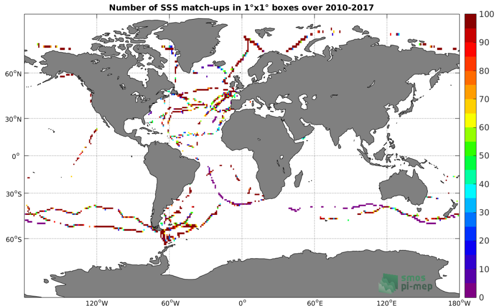
Figure 4: Number of SSS match-ups between TSG-GOSUD-Sailing-ship SSS and the SMOS-L3-CATDS-CECOS-IFREMER-V2-1DAY-0.5DEG SSS product for the Global Ocean Pi-MEP region over 1^\circ \times 1^\circ boxes and for the full satellite product period.
