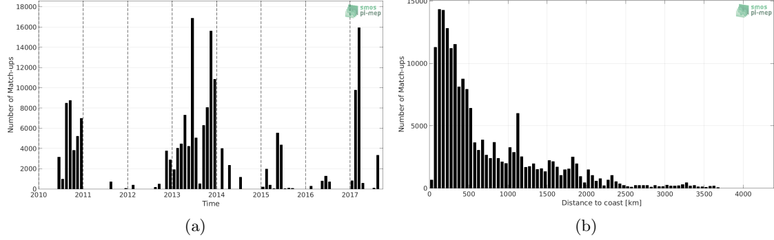
Figure 1: Number of match-ups between TSG-GOSUD-Sailing-ship and SMOS-L3-CATDS-CECOS-IFREMER-V2-1DAY-0.5DEG SSS as a function of time (a) and as function of the distance to coast (b) over the Global Ocean Pi-MEP region and for the full satellite product period.
