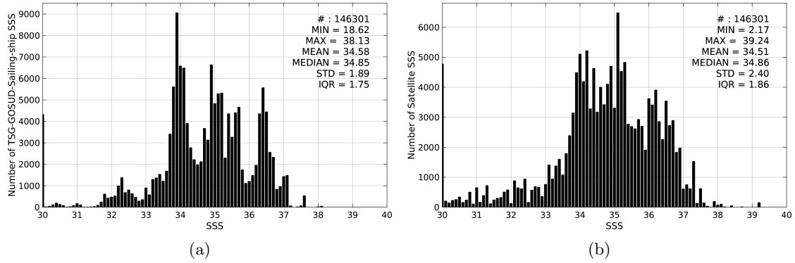
Figure 2: Histograms of SSS from TSG-GOSUD-Sailing-ship (a) and SMOS-L3-CATDS-CECOS-IFREMER-V2-1DAY-0.5DEG (b) considering all match-up pairs per bins of 0.1 over the Global Ocean Pi-MEP region and for the full satellite product period.
