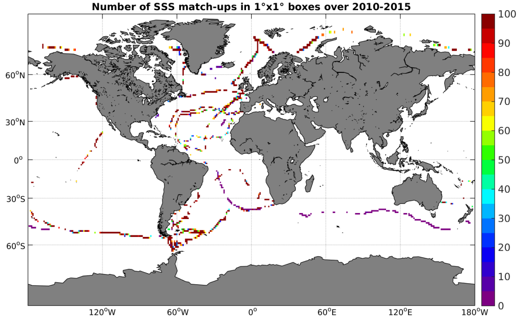
Figure 4: Number of SSS match-ups between TSG-GOSUD-Sailing-ship SSS and the SMOS-L3-CATDS-CECOS-IFREMER-V2-1DAY-0.5deg SSS product for the Global Ocean Pi-MEP region over 1°x1° boxes and for the full satellite product period.
