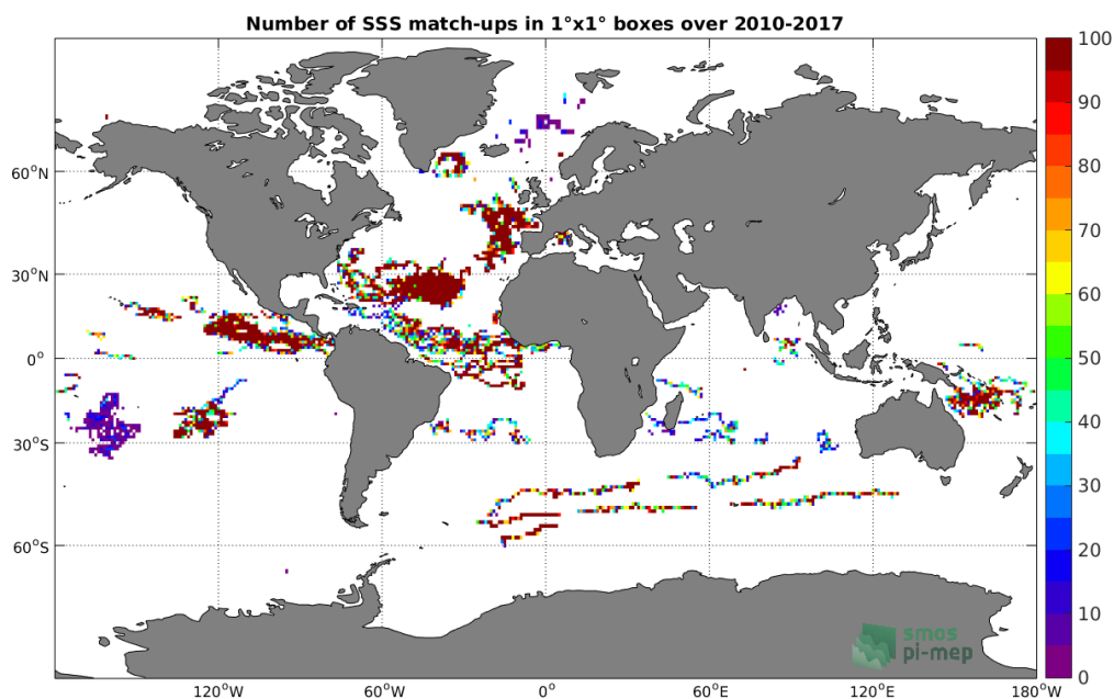
Figure 3: Number of SSS match-ups between Surface drifters SSS and the SMOS-L3-CATDS-CECOS-IFREMER-V2-1DAY-0.5DEG SSS product for the Global Ocean Pi-MEP region over 1^\circ \times 1^\circ boxes and for the full satellite product period.
