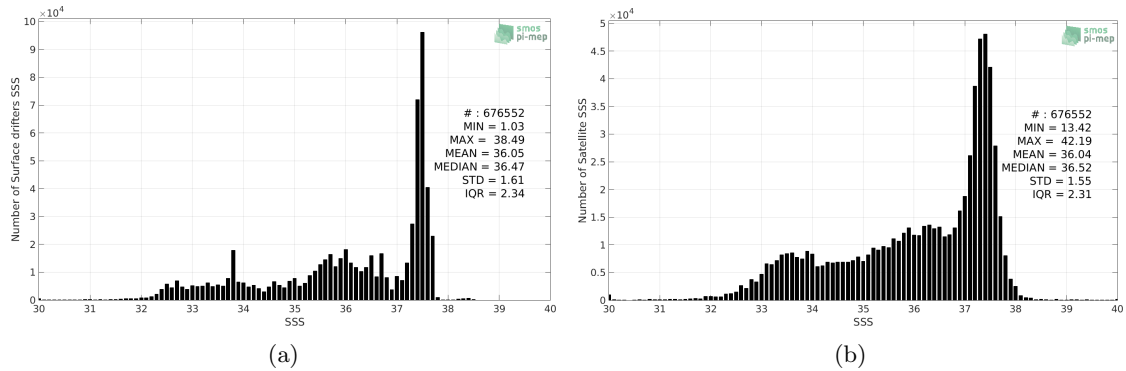
Figure 2: Histograms of SSS from Surface drifters (a) and SMOS-L3-CATDS-CECOS-IFREMER-V2-1DAY-0.5DEG (b) considering all match-up pairs per bins of 0.1 over the Global Ocean Pi-MEP region and for the full satellite product period.
