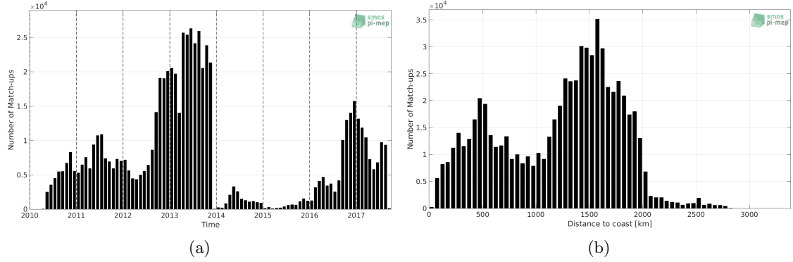
Figure 1: Number of match-ups between Surface drifters and SMOS-L3-CATDS-CECOS-IFREMER-V2-1DAY-0.5DEG SSS as a function of time (a) and as function of the distance to coast (b) over the Global Ocean Pi-MEP region and for the full satellite product period.
