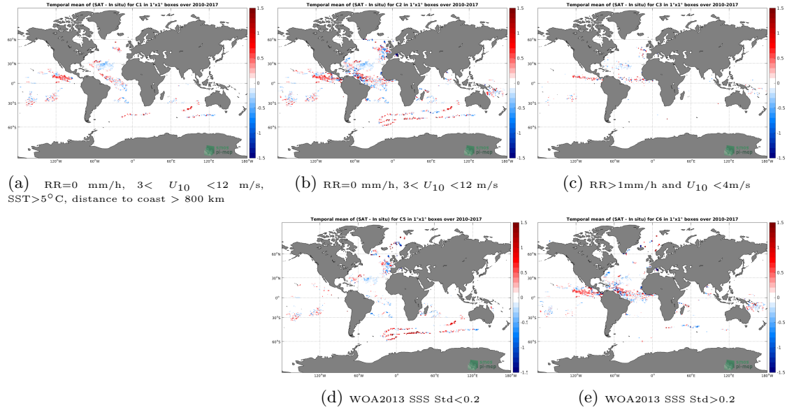
Figure 11: Temporal mean gridded over spatial boxes of size 1^\circ \times 1^\circ of \Delta SSS (SMOS-L3-CATDS-CECOS-IFREMER-V2-1DAY-0.5DEG - Surface drifters) for 5 different subdatasets corresponding to: RR=0 mm/h, 3 < U_{10} < 12 m/s, SST >5^\circ C, distance to coast > 800 km (a), RR=0 mm/h, 3 < U_{10} < 12 m/s (b), RR >1 mm/h and U_{10} < 4 m/s (c), WOA2013 SSS Std <0.2 (d), WOA2013 SSS Std >0.2 (e).
