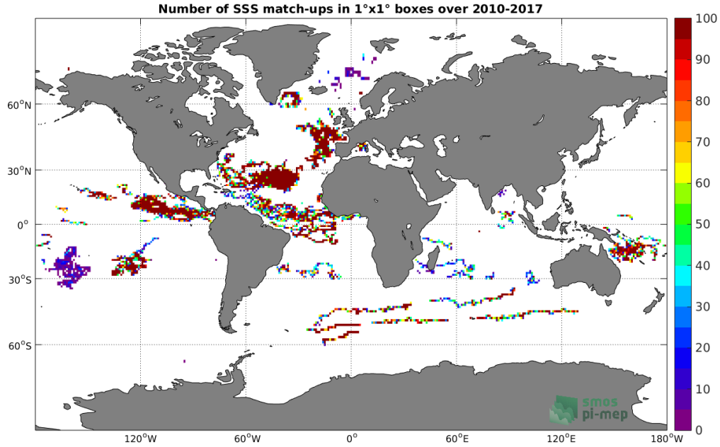
Figure 3: Number of SSS match-ups between Surface drifters SSS and the SMOS-L3-CATDS-CECOS-IFREMER-V2-1DAY-0.5DEG SSS product for the Global Ocean Pi-MEP region over 1^\circ \times 1^\circ boxes and for the full satellite product period.
