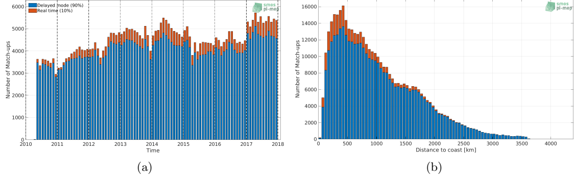
Figure 1: Number of match-ups between Argo and SMOS SSS L3 v2 - Daily - 0.5 Deg (CATDS-CECOS-IFREMER) SSS as a function of time (a) and as function of the distance to coast (b) over the Global Ocean Pi-MEP region and for the full satellite product period.
