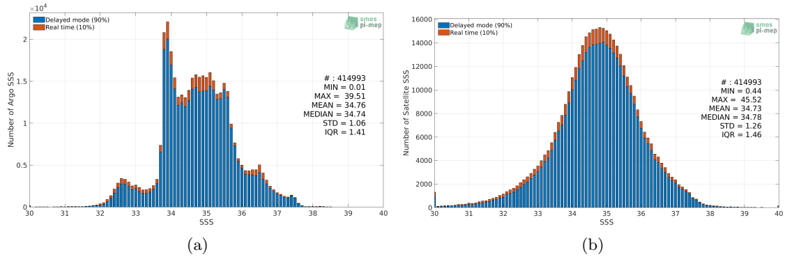
Figure 2: Histograms of SSS from Argo (a) and SMOS SSS L3 v2 - Daily - 0.5 Deg (CATDS-CECOS-IFREMER) (b) considering all match-up pairs per bins of 0.1 over the Global Ocean Pi-MEP region and for the full satellite product period.
