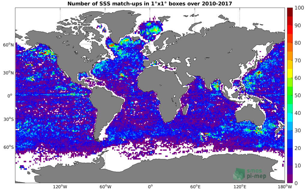
Figure 4: Number of SSS match-ups between Argo SSS and the SMOS SSS L3 v2 - Daily - 0.5 Deg (CATDS-CECOS-IFREMER) SSS product for the Global Ocean Pi-MEP region over 1^\circ \times 1^\circ boxes and for the full satellite product period.
