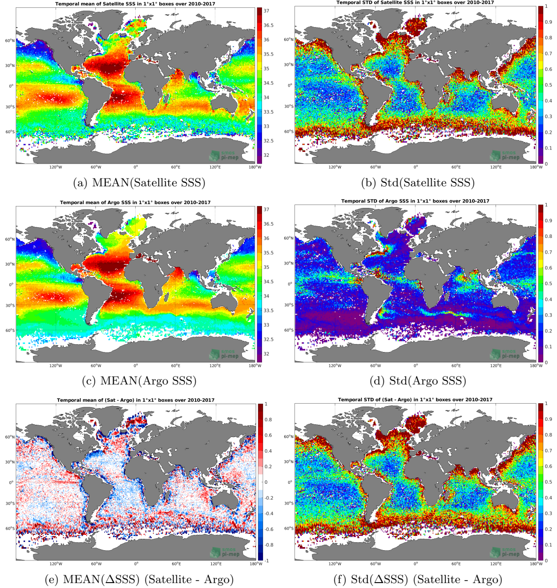
Figure 6: Temporal mean (left) and Std (right) of SSS from SMOS SSS L3 v2 - Daily - 0.5 Deg (CATDS-CECOS-IFREMER) (top), Argo (middle), and of \Delta SSS (Satellite - Argo). Only match-up pairs are used to generate these maps.
