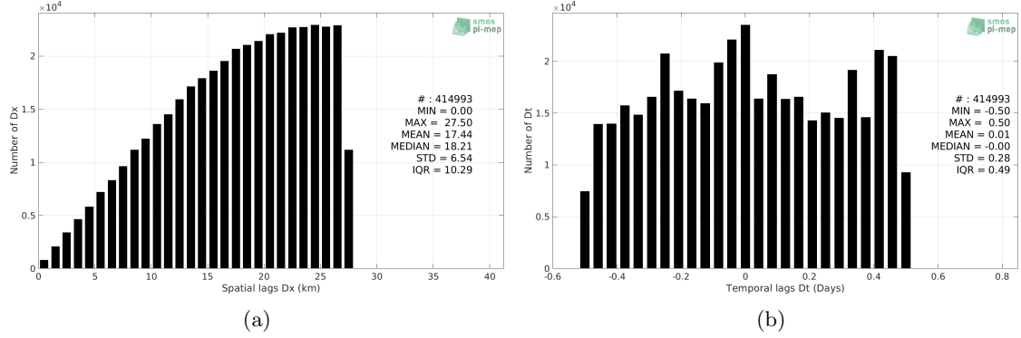
Figure 5: Histograms of the spatial (a) and temporal (b) lags between the location/time of the Argo measurement and the date of the corresponding SMOS SSS L3 v2 - Daily - 0.5 Deg (CATDS-CECOS-IFREMER) SSS pixel.
