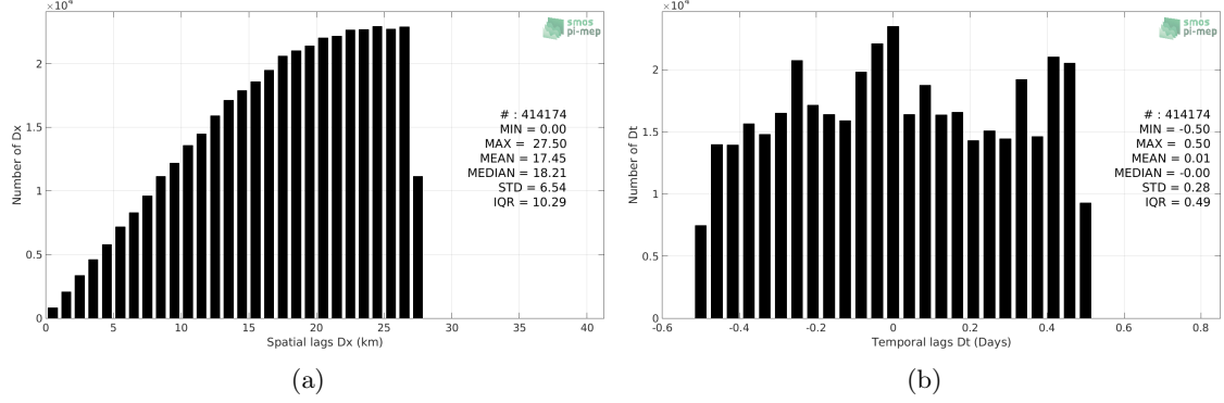
Figure 5: Histograms of the spatial (a) and temporal (b) lags between the time of the Argo measurements and the date of the corresponding SMOS SSS L3 v2 - Daily - 0.5 Deg (CATDS-CECOS-IFREMER) SSS product.
