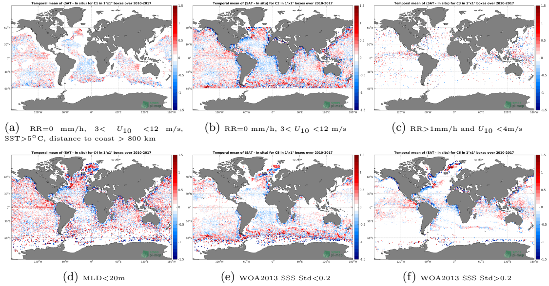
Figure 12: Temporal mean gridded over spatial boxes of size 1^\circ \times 1^\circ of \Delta SSS (SMOS-L3-CATDS-CECOS-IFREMER-V2-1DAY-0.5DEG - Argo) for 6 different subdatasets corresponding to: RR=0 mm/h, 3 < U_{10} < 12 m/s, SST >5^\circ\text{C} , distance to coast > 800 km (a), RR=0 mm/h, 3 < U_{10} < 12 m/s (b), RR >1 mm/h and U_{10} < 4 m/s (c),MLD <20 m (d),WOA2013 SSS Std <0.2 (e),WOA2013 SSS Std >0.2 (f).
