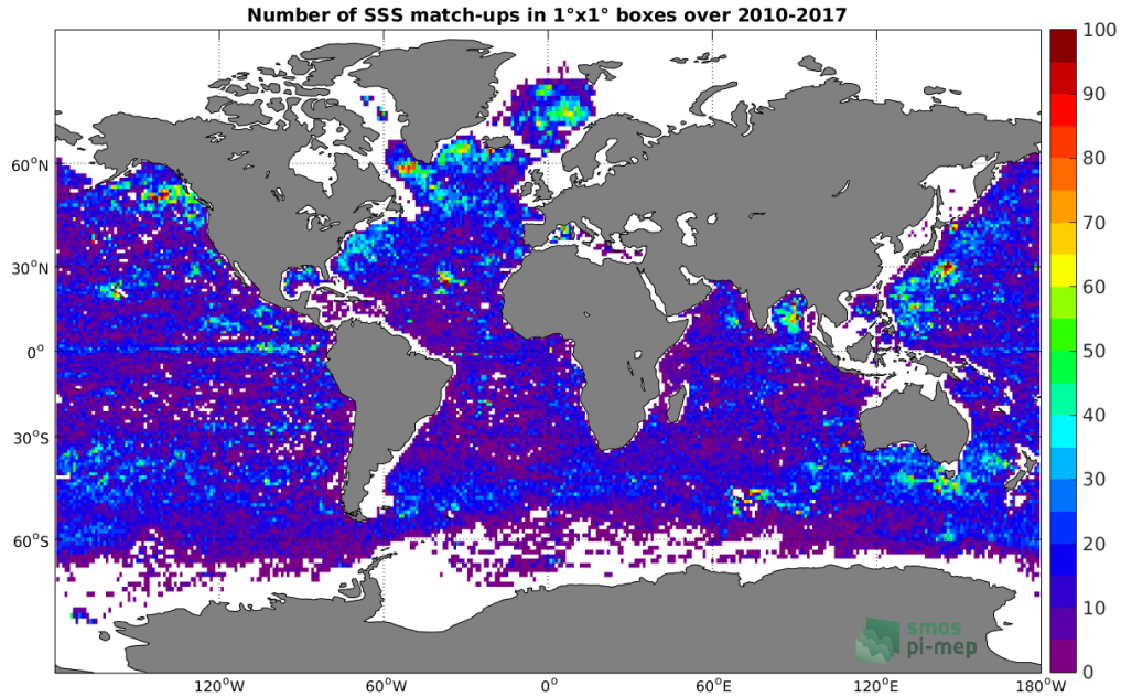
Figure 4: Number of SSS match-ups between Argo SSS and the SMOS-L3-CATDS-CECOS-IFREMER-V2-1DAY-0.5DEG SSS product for the Global Ocean Pi-MEP region over 1°x1° boxes and for the full satellite product period.
