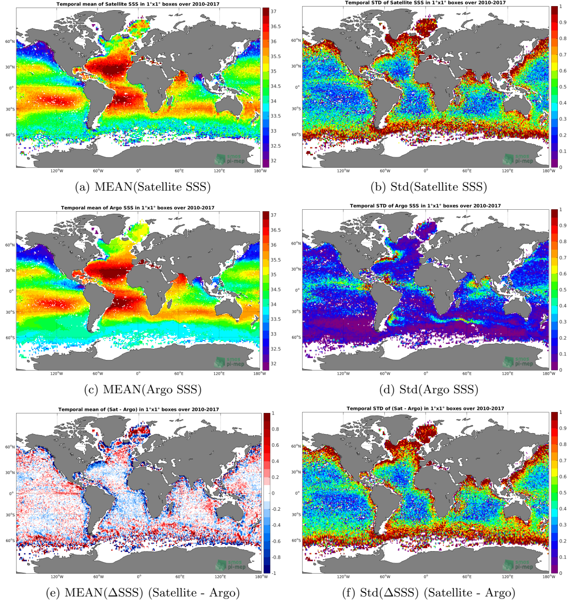
Figure 6: Temporal mean (left) and Std (right) of SSS from SMOS-L3-CATDS-CECOS-IFREMER-V2-1DAY-0.5DEG (top), Argo (middle), and of \Delta SSS (Satellite - Argo). Only match-up pairs are used to generate these maps.
