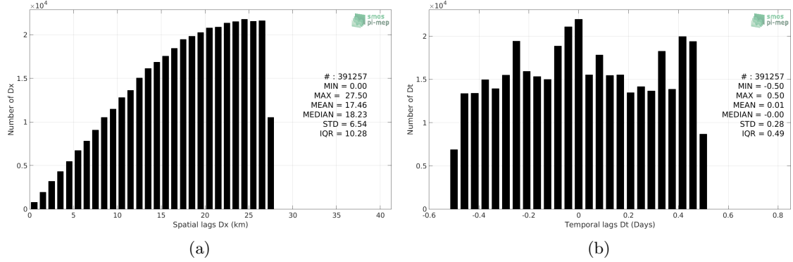
Figure 5: Histograms of the spatial (a) and temporal (b) lags between the time of the Argo measurements and the date of the corresponding SMOS-L3-CATDS-CECOS-IFREMER-V2-1DAY-0.5DEG SSS product.
