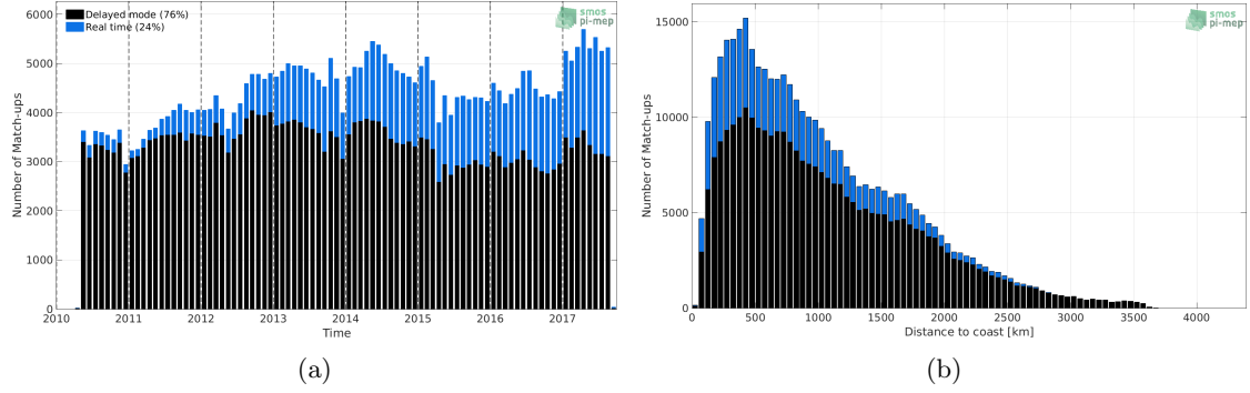
Figure 1: Number of match-ups between Argo and SMOS-L3-CATDS-CECOS-IFREMER-V2-1DAY-0.5DEG SSS as a function of time (a) and as function of the distance to coast (b) over the Global Ocean Pi-MEP region and for the full satellite product period.
