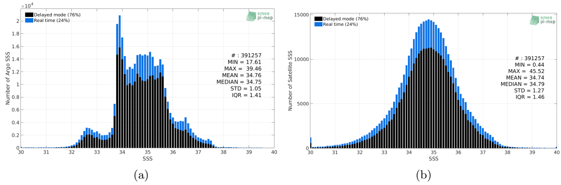
Figure 2: Histograms of SSS from Argo (a) and SMOS-L3-CATDS-CECOS-IFREMER-V2-1DAY-0.5DEG (b) considering all match-up pairs per bins of 0.1 over the Global Ocean Pi-MEP region and for the full satellite product period.
