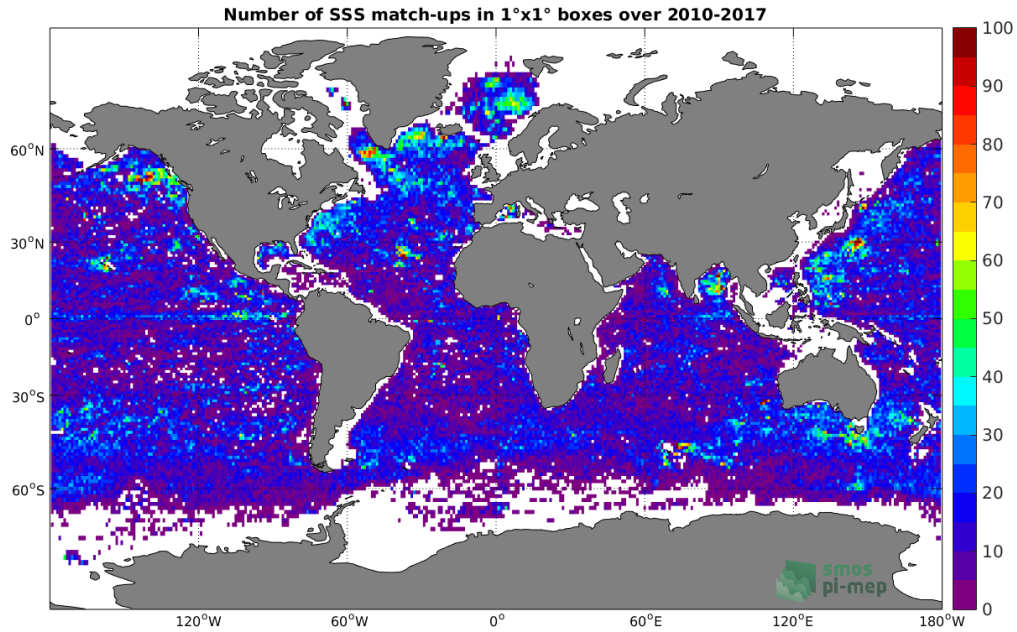
Figure 4: Number of SSS match-ups between Argo SSS and the SMOS-L3-CATDS-CECOS-IFREMER-V2-1DAY-0.5DEG SSS product for the Global Ocean Pi-MEP region over 1^\circ \times 1^\circ boxes and for the full satellite product period.
