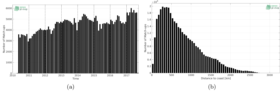
Figure 1: Number of match-ups between Argo and SMOS-L3-CATDS-CECOS-IFREMER-V2-1DAY-0.5DEG SSS as a function of time (a) and as function of the distance to coast (b) over the Global Ocean Pi-MEP region and for the full satellite product period.
