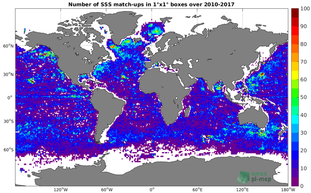
Figure 4: Number of SSS match-ups between Argos SSS and the SMOS-L3-CATDS-CECOS-IFREMER-V2-1DAY-0.5DEG SSS product for the Global Ocean Pi-MEP region over 1^\circ \times 1^\circ boxes and for the full satellite product period.
