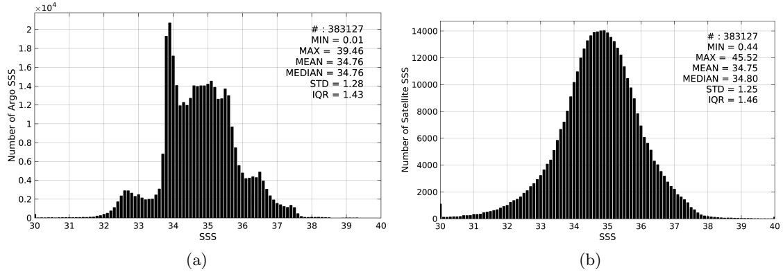
Figure 2: Histograms of SSS from Argos (a) and SMOS-L3-CATDS-CECOS-IFREMER-V2-1DAY-0.5deg (b) considering all match-up pairs per bins of 0.1 over the Global Ocean Pi-MEP region and for the full satellite product period.
