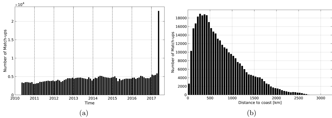
Figure 1: Number of match-ups between Argo and SMOS-L3-CATDS-CECOS-IFREMER-V2-1DAY-0.5deg SSS as a function of time (a) and as function of the distance to coast (b) over the Global Ocean Pi-MEP region and for the full satellite product period.
