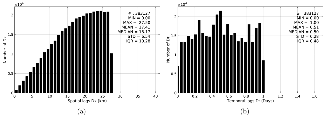
Figure 5: Histograms of the spatial (a) and temporal (b) lags between the time of the Argo measurements and the date of the corresponding SMOS-L3-CATDS-CECOS-IFREMER-V2-1DAY-0.5deg SSS product.
