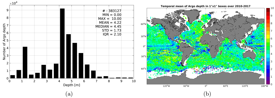
Figure 3: Histograms of the depth of the upper level SSS measurements from Argos in the Match-up DataBase for the Global Ocean Pi-MEP region (a) and temporal mean spatial distribution of pressure of the in situ SSS data over 1^\circ \times 1^\circ boxes and for the full satellite product period (b).
