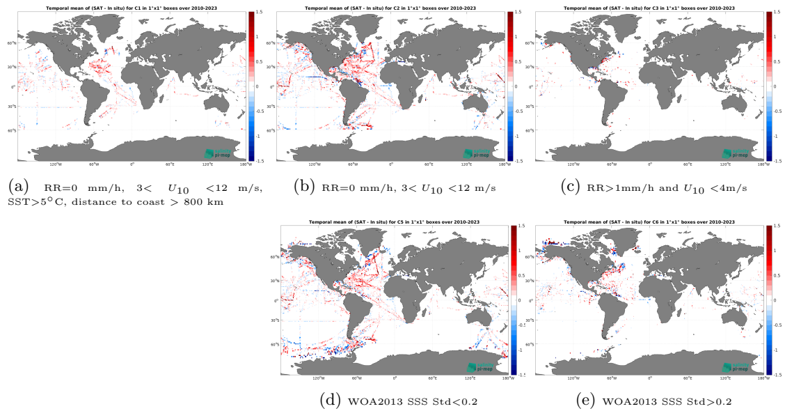
Figure 12: Temporal mean gridded over spatial boxes of size 1^\circ \times 1^\circ of \Delta\text{SSS} (SMOS SSS L3 v335 - Monthly - 25 km (CATDS-CPDC) - TSG (SAMOS)) for 5 different subdatasets corresponding to:RR=0 mm/h, 3 < U_{10} < 12 m/s, SST >5^\circ\text{C} , distance to coast > 800 km (a), RR=0 mm/h, 3 < U_{10} < 12 m/s (b), RR >1 mm/h and U_{10} < 4 m/s (c), WOA2013 SSS Std <0.2 (d), WOA2013 SSS Std >0.2 (e).
