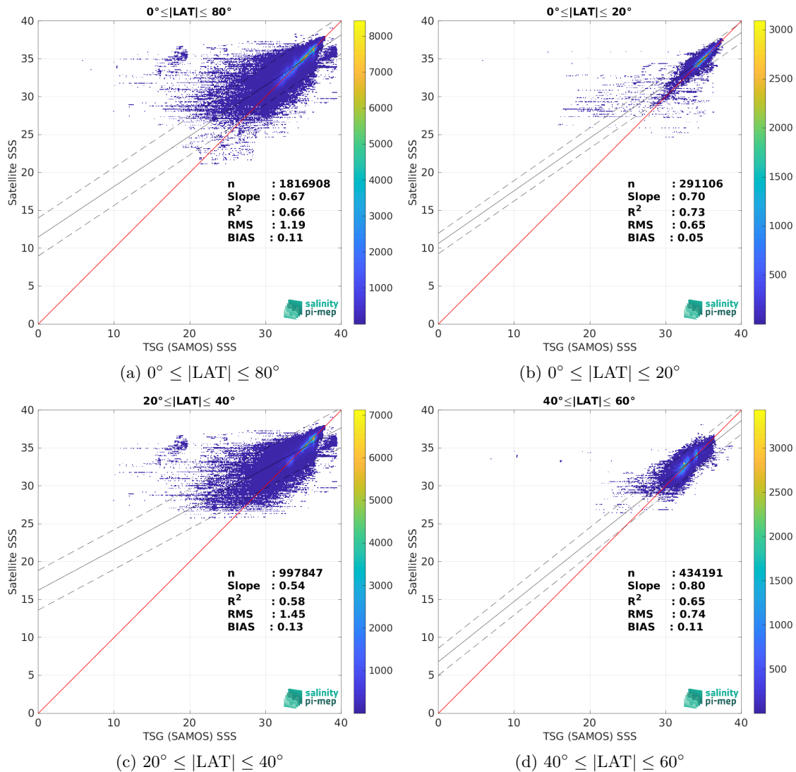
Figure 9: Contour maps of the concentration of SMOS SSS L3 v335 - Monthly - 25 km (CATDS-CPDC) SSS (y-axis) versus TSG (SAMOS) SSS (x-axis) at match-up pairs for different latitude bands. For each plot, the red line shows x=y . The black thin and dashed lines indicate a linear fit through the data cloud and the \pm 95\% confidence levels, respectively. The number match-up pairs n , the slope and R^2 coefficient of the linear fit, the root mean square (RMS) and the mean bias between satellite and in situ data are indicated for each latitude band in each plot.
