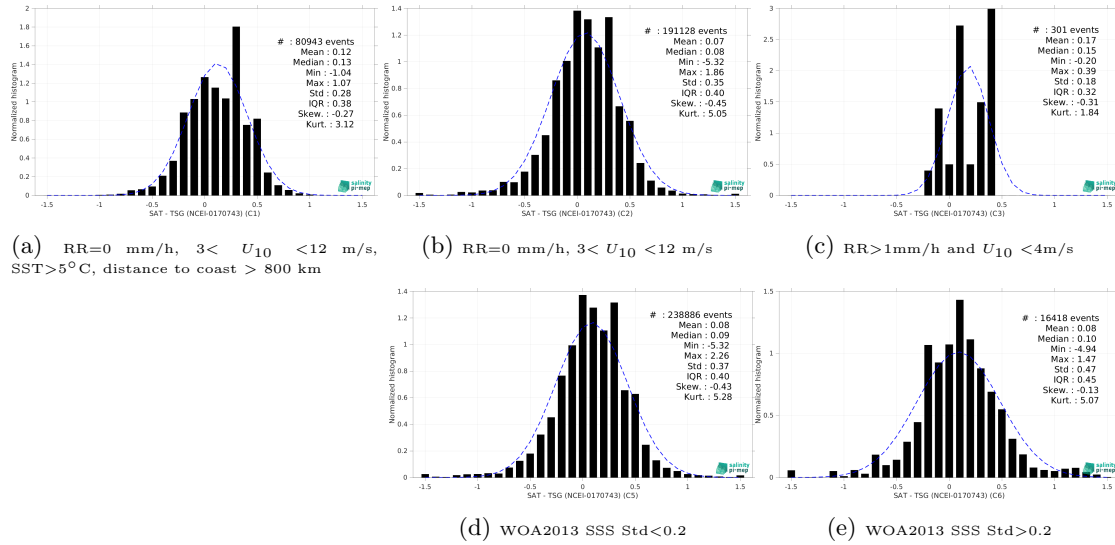
Figure 13: Normalized histogram of \Delta SSS (SMOS SSS L3 v335 - Monthly - 25 km (CATDS-CPDC) - TSG (NCEI-0170743)) for 5 different subdatasets corresponding to: RR=0 mm/h, 3 < U_{10} < 12 m/s, SST>5°C, distance to coast > 800 km (a), RR=0 mm/h, 3 < U_{10} < 12 m/s (b), RR>1mm/h and U_{10} < 4 m/s (c), WOA2013 SSS Std<0.2 (d), WOA2013 SSS Std>0.2 (e).
