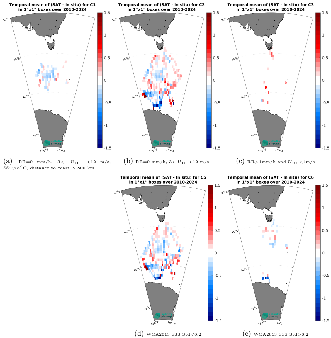
Figure 14: Temporal mean gridded over spatial boxes of size 1^\circ \times 1^\circ of \Delta\text{SSS} (SMOS SSS L3 v335 - Monthly - 25 km (CATDS-CPDC) - TSG (LEGOS-Survostral)) for 5 different subdatasets corresponding to: RR=0 mm/h, 3 < U_{10} < 12 m/s, SST > 5^\circ\text{C} , distance to coast > 800 km (a), RR=0 mm/h, 3 < U_{10} < 12 m/s (b), RR > 1 mm/h and U_{10} < 4 m/s (c), WOA2013 SSS Std < 0.2 (d), WOA2013 SSS Std > 0.2 (e).
