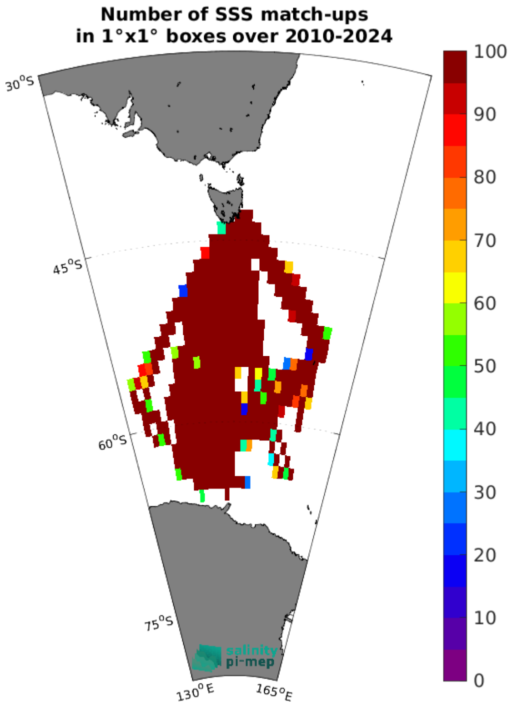
Figure 5: Number of SSS match-ups between TSG (LEGOS-Survostral) SSS and the SMOS SSS L3 v335 - Monthly - 25 km (CATDS-CPDC) SSS product for the Global Ocean Pi-MEP region over 1°x1° boxes and for the full satellite product period.
