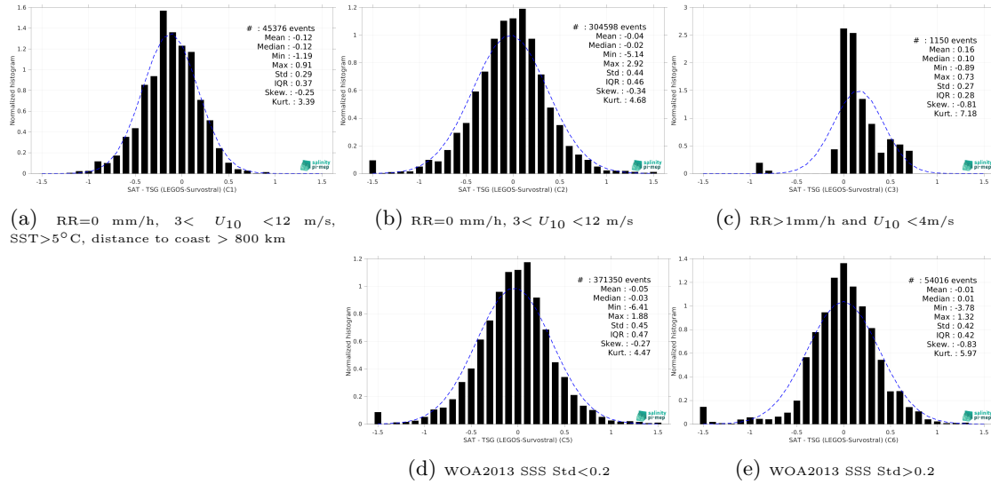
Figure 15: Normalized histogram of \Delta SSS (SMOS SSS L3 v335 - Monthly - 25 km (CATDS-CPDC) - TSG (LEGOS-Survostral)) for 5 different subdatasets corresponding to: RR=0 mm/h, 3 < U_{10} < 12 m/s, SST>5°C, distance to coast > 800 km (a), RR=0 mm/h, 3 < U_{10} < 12 m/s (b), RR>1mm/h and U_{10} < 4 m/s (c), WOA2013 SSS Std<0.2 (d), WOA2013 SSS Std>0.2 (e).
