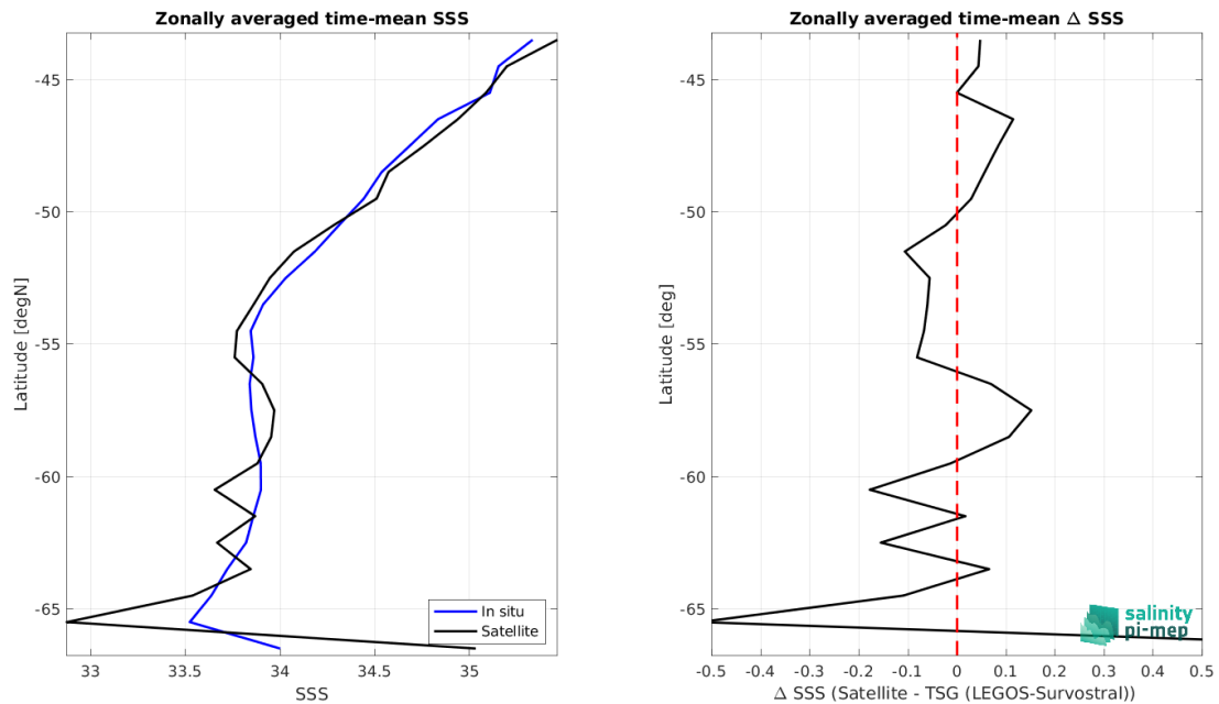
Figure 9: Left panel: Zonal mean SSS from SMOS SSS L3 v335 - Monthly - 25 km (CATDS-CPDC) satellite product (black) and from TSG (LEGOS-Survostral) (blue). Right panel: Zonal mean of \Delta SSS (Satellite - TSG (LEGOS-Survostral)) for all the collected Pi-MEP match-up pairs estimated over the full satellite product period.
