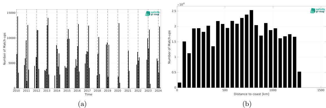
Figure 2: Number of match-ups between TSG (LEGOS-Survostral) and SMOS SSS L3 v335 - Monthly - 25 km (CATDS-CPDC) SSS as a function of time (a) and as function of the distance to coast (b) over the Global Ocean Pi-MEP region and for the full satellite product period.
