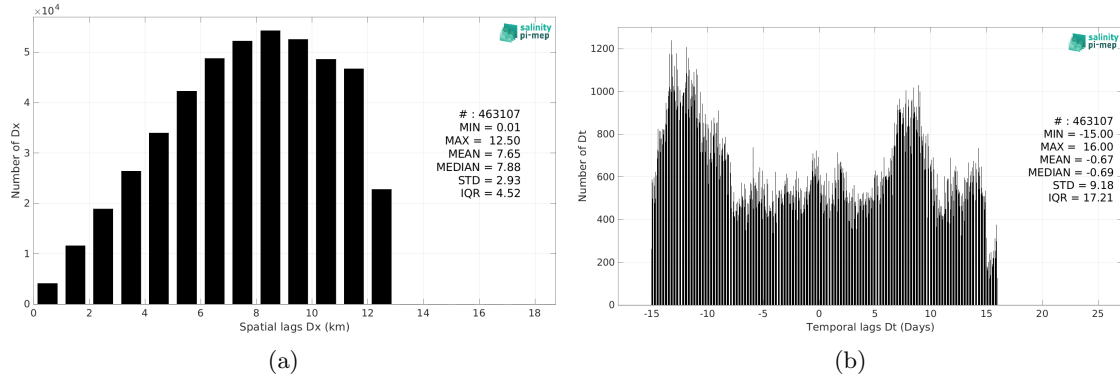
Figure 6: Histograms of the spatial (a) and temporal (b) lags between the location/time of the TSG (LEGOS-Survostral) measurement and the date of the corresponding SMOS SSS L3 v335 - Monthly - 25 km (CATDS-CPDC) SSS pixel.
