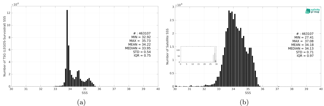
Figure 3: Histograms of SSS from TSG (LEGOS-Survostral) (a) and SMOS SSS L3 v335 - Monthly - 25 km (CATDS-CPDC) (b) considering all match-up pairs per bins of 0.1 over the Global Ocean Pi-MEP region and for the full satellite product period.
