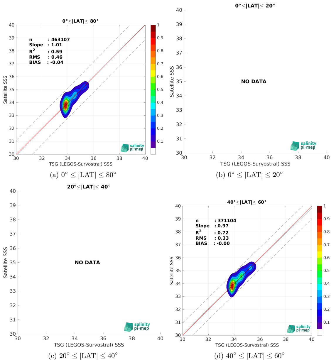
Figure 10: Contour maps of the concentration of SMOS SSS L3 v335 - Monthly - 25 km (CATDS-CPDC) SSS (y-axis) versus TSG (LEGOS-Survostral) SSS (x-axis) at match-up pairs for different latitude bands. For each plot, the red line shows x=y . The black thin and dashed lines indicate a linear fit through the data cloud and the \pm 95\% confidence levels, respectively. The number match-up pairs n , the slope and R^2 coefficient of the linear fit, the root mean square (RMS) and the mean bias between satellite and in situ data are indicated for each latitude band in each plots.
