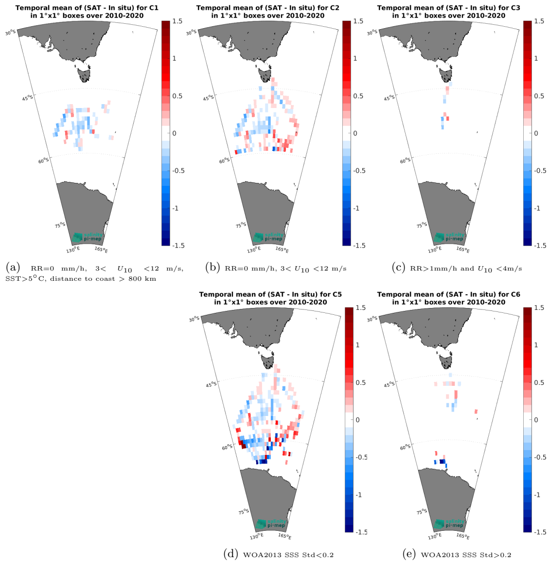
Figure 12: Temporal mean gridded over spatial boxes of size 1^\circ \times 1^\circ of \Delta\text{SSS} (SMOS SSS L3 v335 - Monthly - 25 km (CATDS-CPDC) - TSG (LEGOS-Survostral)) for 5 different subdatasets corresponding to: RR=0 mm/h, 3 < U_{10} < 12 m/s, SST > 5^\circ\text{C} , distance to coast > 800 km (a), RR=0 mm/h, 3 < U_{10} < 12 m/s (b), RR > 1 mm/h and U_{10} < 4 m/s (c), WOA2013 SSS Std < 0.2 (d), WOA2013 SSS Std > 0.2 (e).
