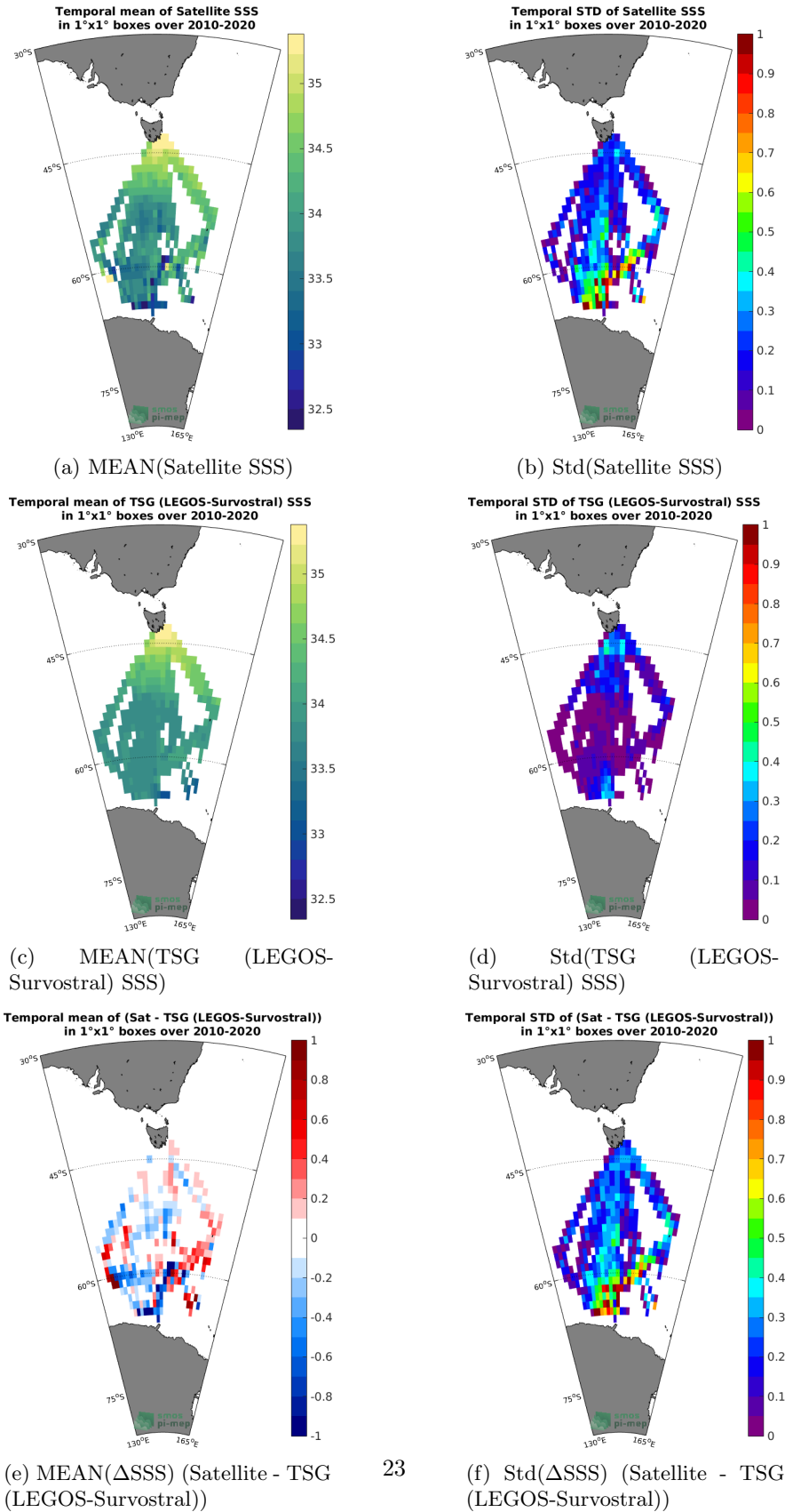
Figure 6: Temporal mean (left) and Std (right) of SSS from SMOS SSS L3 v335 - Monthly - 25 km (CATDS-CPDC) (top), TSG (LEGOS-Survostral) (middle), and of \Delta SSS (Satellite - TSG (LEGOS-Survostral)). Only match-up pairs are used to generate these maps.
