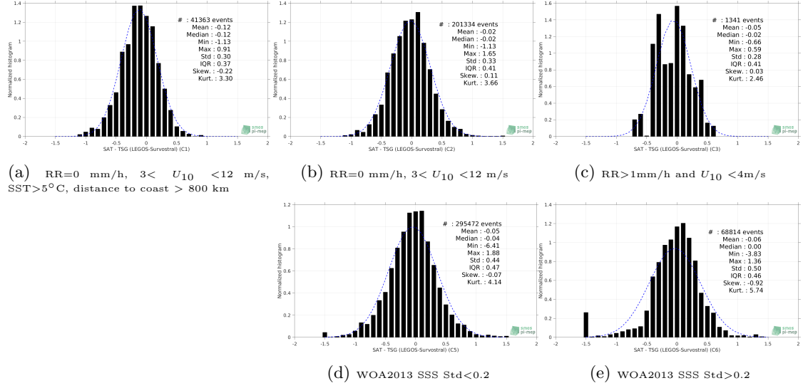
Figure 13: Normalized histogram of \Delta SSS (SMOS SSS L3 v335 - Monthly - 25 km (CATDS-CPDC) - TSG (LEGOS-Survostral)) for 5 different subdatasets corresponding to: RR=0 mm/h, 3 < U_{10} < 12 m/s, SST>5°C, distance to coast > 800 km (a), RR=0 mm/h, 3 < U_{10} < 12 m/s (b), RR>1mm/h and U_{10} < 4 m/s (c), WOA2013 SSS Std<0.2 (d), WOA2013 SSS Std>0.2 (e).
