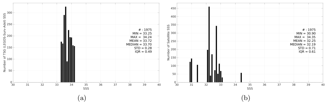
Figure 3: Histograms of SSS from TSG (LEGOS-Surv-Adel) (a) and SMOS SSS L3 v335 - Monthly - 25 km (CATDS-CPDC) (b) considering all match-up pairs per bins of 0.1 over the Global Ocean Pi-MEP region and for the full satellite product period.
