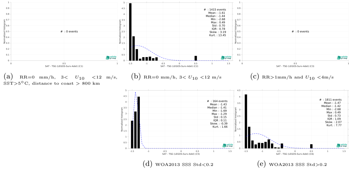
Figure 15: Normalized histogram of \Delta SSS (SMOS SSS L3 v335 - Monthly - 25 km (CATDS-CPDC) - TSG (LEGOS-Surv-Adel)) for 5 different subdatasets corresponding to: RR=0 mm/h, 3 < U_{10} < 12 m/s, SST > 5°C, distance to coast > 800 km (a), RR=0 mm/h, 3 < U_{10} < 12 m/s (b), RR > 1mm/h and U_{10} < 4 m/s (c), WOA2013 SSS Std < 0.2 (d), WOA2013 SSS Std > 0.2 (e).
