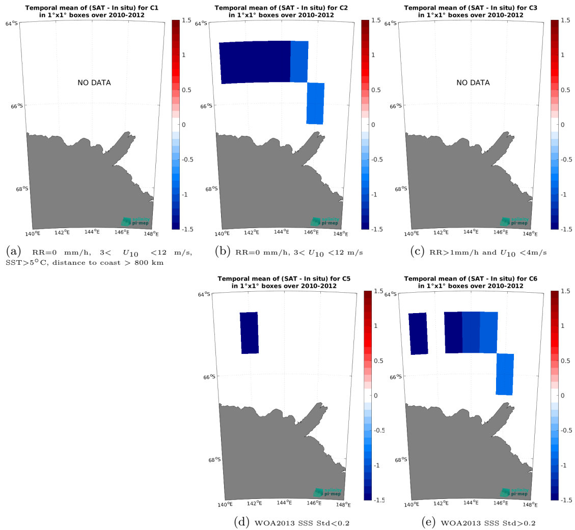
Figure 14: Temporal mean gridded over spatial boxes of size 1^{\circ}\times 1^{\circ} of \Delta SSS (SMOS SSS L3 v335 - Monthly - 25 km (CATDS-CPDC) - TSG (LEGOS-Surv-Adel)) for 5 different subdatasets corresponding to:RR=0 mm/h, 3 < U_{10} < 12 m/s, SST>5°C, distance to coast > 800 km (a), RR=0 mm/h, 3 < U_{10} < 12 m/s (b), RR>1mm/h and U_{10} < 4 m/s (c), WOA2013 SSS Std<0.2 (d), WOA2013 SSS Std>0.2 (e).
