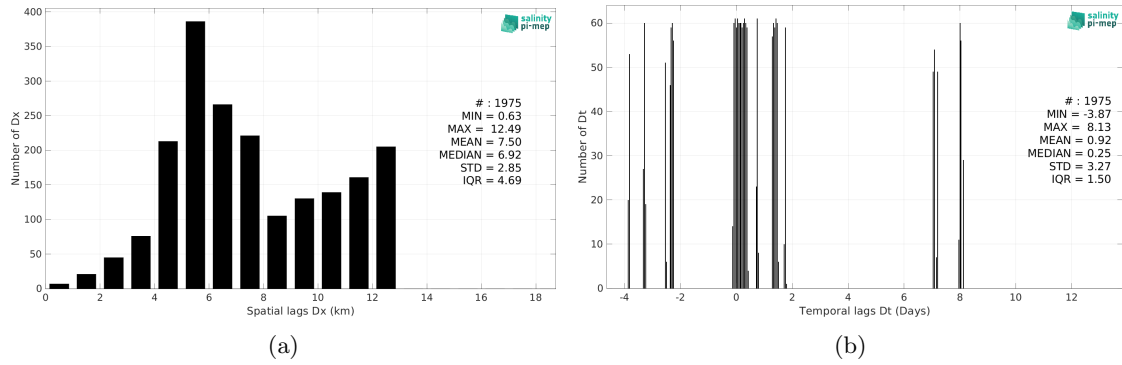
Figure 6: Histograms of the spatial (a) and temporal (b) lags between the location/time of the TSG (LEGOS-Surv-Adel) measurement and the date of the corresponding SMOS SSS L3 v335 - Monthly - 25 km (CATDS-CPDC) SSS pixel.
