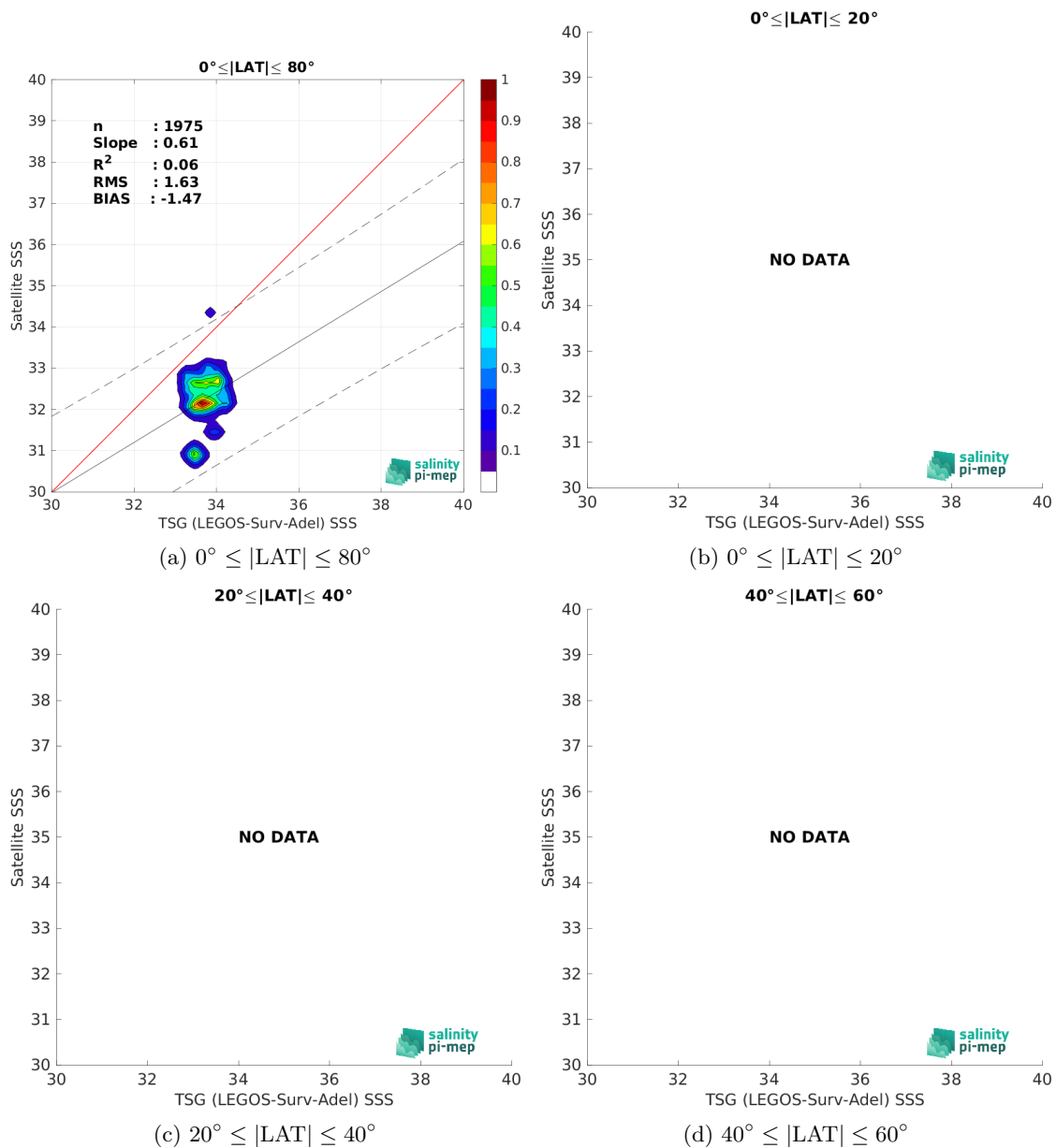
Figure 10: Contour maps of the concentration of SMOS SSS L3 v335 - Monthly - 25 km (CATDS-CPDC) SSS (y-axis) versus TSG (LEGOS-Surv-Adel) SSS (x-axis) at match-up pairs for different latitude bands. For each plot, the red line shows x=y . The black thin and dashed lines indicate a linear fit through the data cloud and the \pm 95\% confidence levels, respectively. The number match-up pairs n , the slope and R^2 coefficient of the linear fit, the root mean square (RMS) and the mean bias between satellite and in situ data are indicated for each latitude band in each plots.
