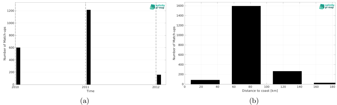
Figure 2: Number of match-ups between TSG (LEGOS-Surv-Adel) and SMOS SSS L3 v335 - Monthly - 25 km (CATDS-CPDC) SSS as a function of time (a) and as function of the distance to coast (b) over the Global Ocean Pi-MEP region and for the full satellite product period.
