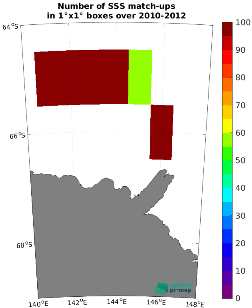
Figure 5: Number of SSS match-ups between TSG (LEGOS-Surv-Adel) SSS and the SMOS SSS L3 v335 - Monthly - 25 km (CATDS-CPDC) SSS product for the Global Ocean Pi-MEP region over 1°x1° boxes and for the full satellite product period.
