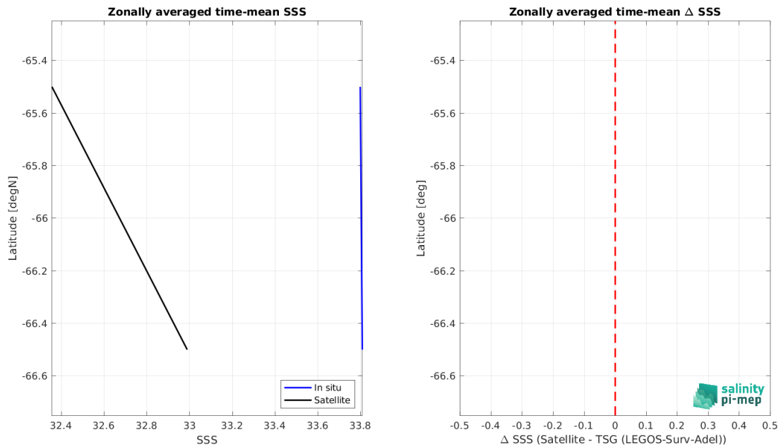
Figure 9: Left panel: Zonal mean SSS from SMOS SSS L3 v335 - Monthly - 25 km (CATDS-CPDC) satellite product (black) and from TSG (LEGOS-Surv-Adel) (blue). Right panel: Zonal mean of \Delta SSS (Satellite - TSG (LEGOS-Surv-Adel)) for all the collected Pi-MEP match-up pairs estimated over the full satellite product period.
