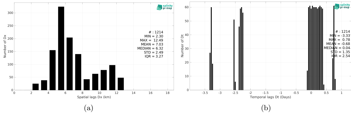
Figure 6: Histograms of the spatial (a) and temporal (b) lags between the location/time of the TSG (LEGOS-Surv-Adel) measurement and the date of the corresponding SMOS SSS L3 v335 - Monthly - 25 km (CATDS-CPDC) SSS pixel.
