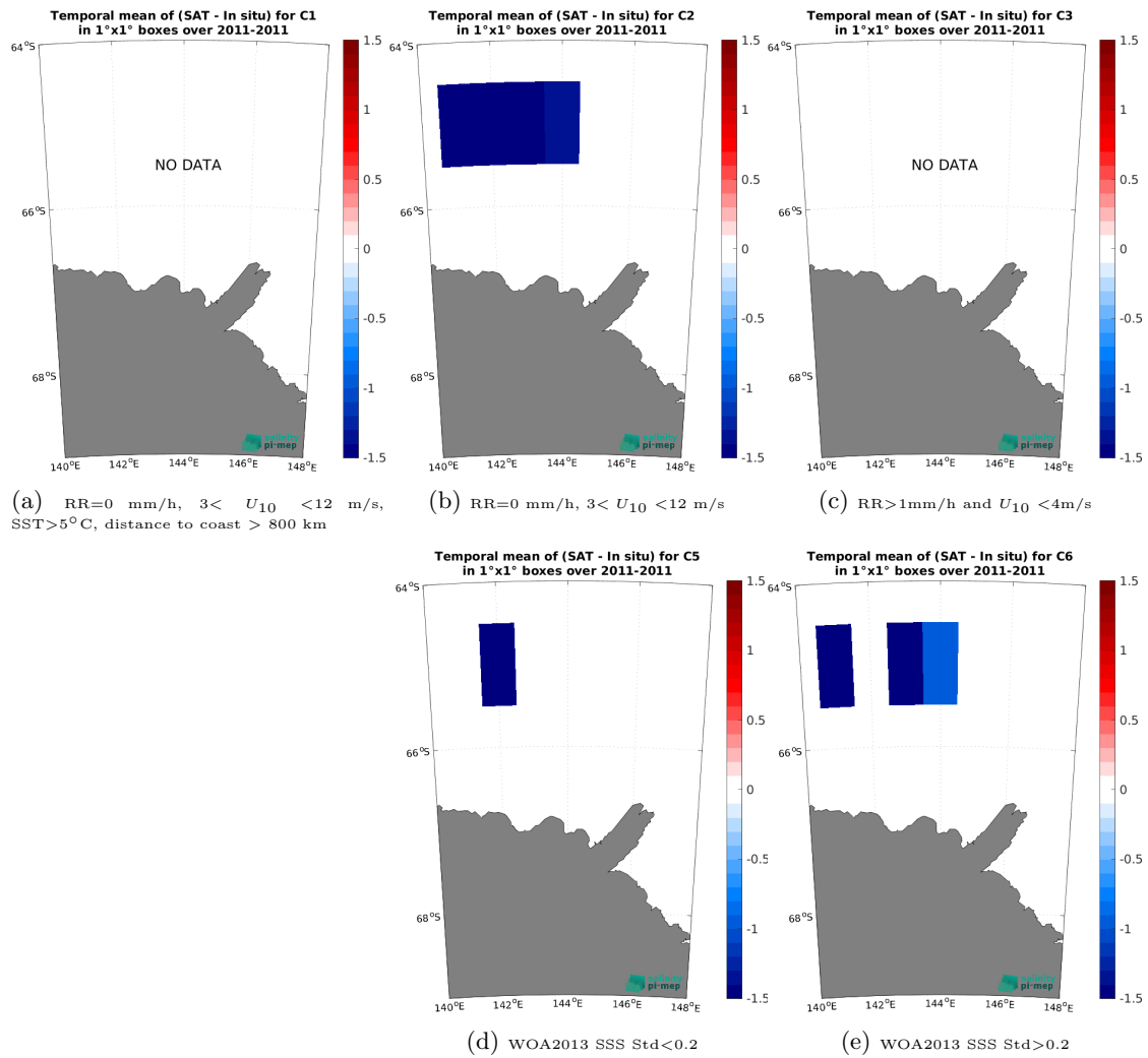
Figure 14: Temporal mean gridded over spatial boxes of size 1^\circ \times 1^\circ of \Delta SSS (SMOS SSS L3 v335 - Monthly - 25 km (CATDS-CPDC) - TSG (LEGOS-Surv-Adel)) for 5 different subdatasets corresponding to: RR=0 mm/h, 3 < U_{10} < 12 m/s, SST>5°C, distance to coast > 800 km (a), RR=0 mm/h, 3 < U_{10} < 12 m/s (b), RR>1mm/h and U_{10} < 4 m/s (c), WOA2013 SSS Std<0.2 (d), WOA2013 SSS Std>0.2 (e).
