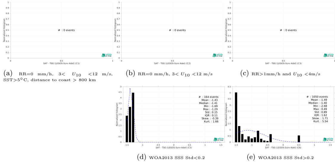
Figure 13: Normalized histogram of \Delta SSS (SMOS SSS L3 v335 - Monthly - 25 km (CATDS-CPDC) - TSG (LEGOS-Surv-Adel)) for 5 different subdatasets corresponding to: RR=0 mm/h, 3 < U_{10} < 12 m/s, SST>5°C, distance to coast > 800 km (a), RR=0 mm/h, 3 < U_{10} < 12 m/s (b), RR>1mm/h and U_{10} < 4 m/s (c), WOA2013 SSS Std<0.2 (d), WOA2013 SSS Std>0.2 (e).
