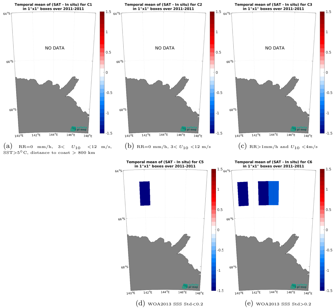
Figure 12: Temporal mean gridded over spatial boxes of size 1^\circ \times 1^\circ of \Delta\text{SSS} (SMOS SSS L3 v335 - Monthly - 25 km (CATDS-CPDC) - TSG (LEGOS-Surv-Adel)) for 5 different subdatasets corresponding to: RR=0 mm/h, 3 < U_{10} < 12 m/s, SST > 5^\circ\text{C} , distance to coast > 800 km (a), RR=0 mm/h, 3 < U_{10} < 12 m/s (b), RR > 1 mm/h and U_{10} < 4 m/s (c), WOA2013 SSS Std < 0.2 (d), WOA2013 SSS Std > 0.2 (e).
