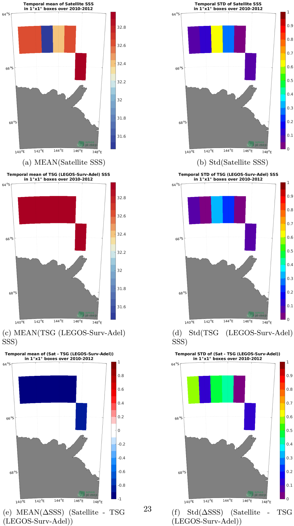
Figure 6: Temporal mean (left) and Std (right) of SSS from SMOS SSS L3 v335 - Monthly - 25 km (CATDS-CPDC) (top), TSG (LEGOS-Surv-Adel) (middle), and of \Delta SSS (Satellite - TSG (LEGOS-Surv-Adel)). Only match-up pairs are used to generate these maps.
