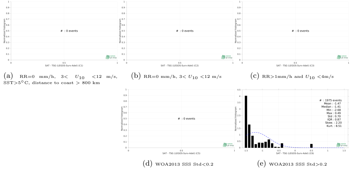
Figure 13: Normalized histogram of \Delta SSS (SMOS SSS L3 v335 - Monthly - 25 km (CATDS-CPDC) - TSG (LEGOS-Surv-Adel)) for 5 different subdatasets corresponding to: RR=0 mm/h, 3 < U_{10} < 12 m/s, SST>5°C, distance to coast > 800 km (a), RR=0 mm/h, 3 < U_{10} < 12 m/s (b), RR>1mm/h and U_{10} < 4 m/s (c), WOA2013 SSS Std<0.2 (d), WOA2013 SSS Std>0.2 (e).
