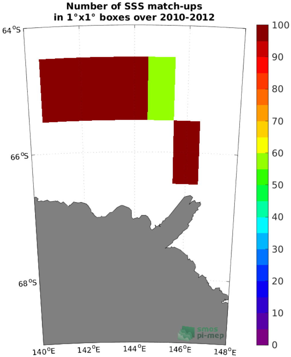
Figure 4: Number of SSS match-ups between TSG (LEGOS-Surv-Adel) SSS and the SMOS SSS L3 v335 - Monthly - 25 km (CATDS-CPDC) SSS product for the Global Ocean Pi-MEP region over 1^\circ \times 1^\circ boxes and for the full satellite product period.
