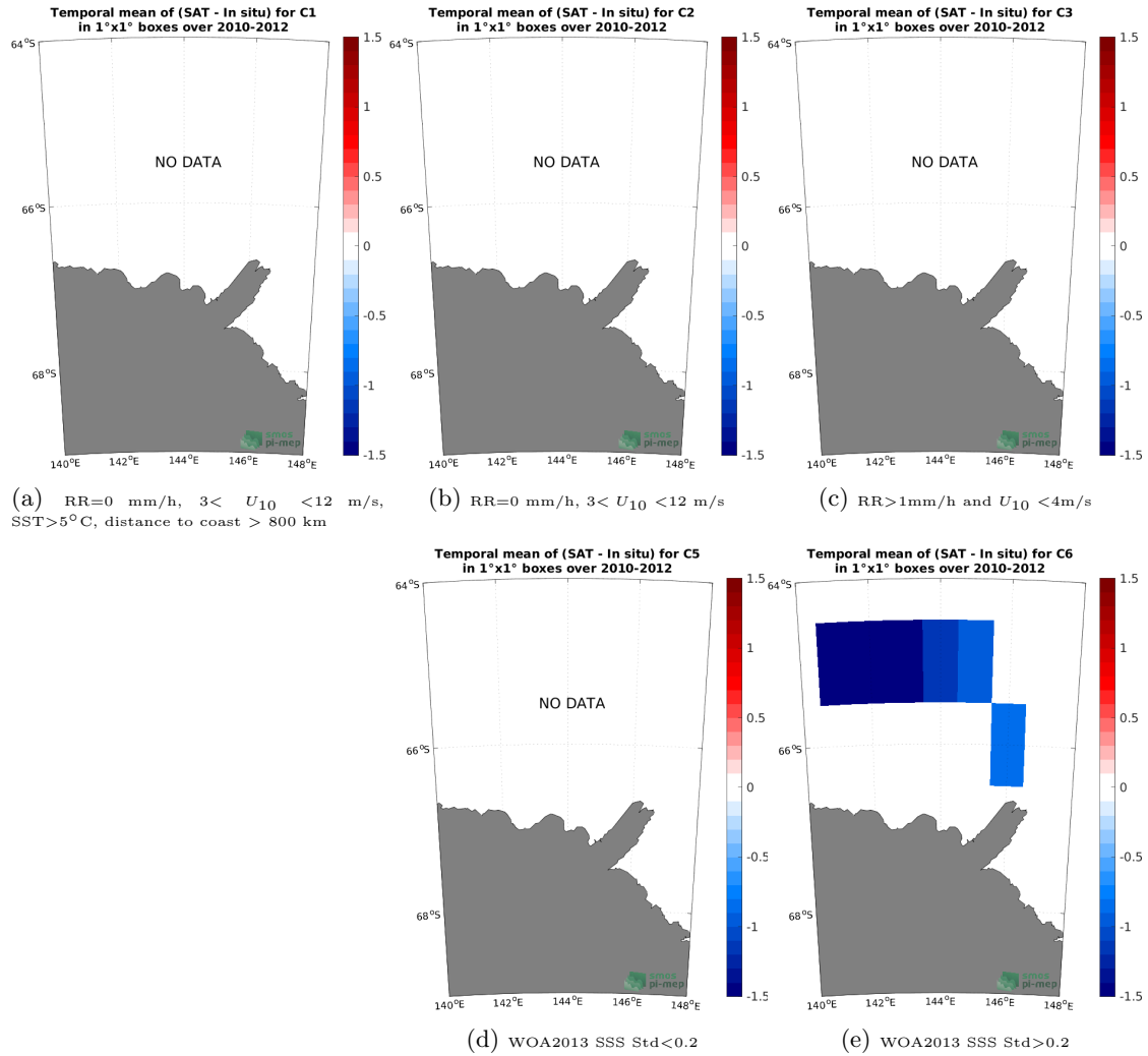
Figure 12: Temporal mean gridded over spatial boxes of size 1°x1° of \Delta SSS (SMOS SSS L3 v335 - Monthly - 25 km (CATDS-CPDC) - TSG (LEGOS-Surv-Adel)) for 5 different subdatasets corresponding to:RR=0 mm/h, 3 < U_{10} < 12 m/s, SST>5°C, distance to coast > 800 km (a), RR=0 mm/h, 3 < U_{10} < 12 m/s (b), RR>1mm/h and U_{10} < 4 m/s (c), WOA2013 SSS Std<0.2 (d), WOA2013 SSS Std>0.2 (e).
