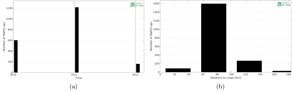
Figure 1: Number of match-ups between TSG (LEGOS-Surv-Adel) and SMOS SSS L3 v335 - Monthly - 25 km (CATDS-CPDC) SSS as a function of time (a) and as function of the distance to coast (b) over the Global Ocean Pi-MEP region and for the full satellite product period.
