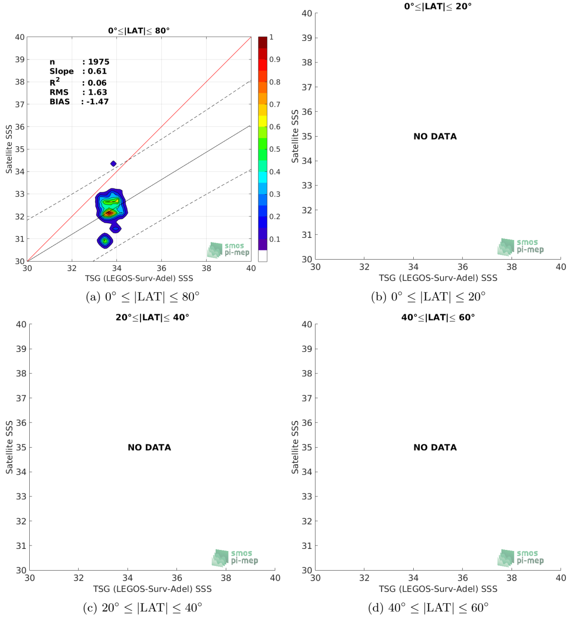
Figure 9: Contour maps of the concentration of SMOS SSS L3 v335 - Monthly - 25 km (CATDS-CPDC) SSS (y-axis) versus TSG (LEGOS-Surv-Adel) SSS (x-axis) at match-up pairs for different latitude bands. For each plot, the red line shows x=y . The black thin and dashed lines indicate a linear fit through the data cloud and the \pm 95\% confidence levels, respectively. The number match-up pairs n , the slope and R^2 coefficient of the linear fit, the root mean square (RMS) and the mean bias between satellite and in situ data are indicated for each latitude band in each plots.
