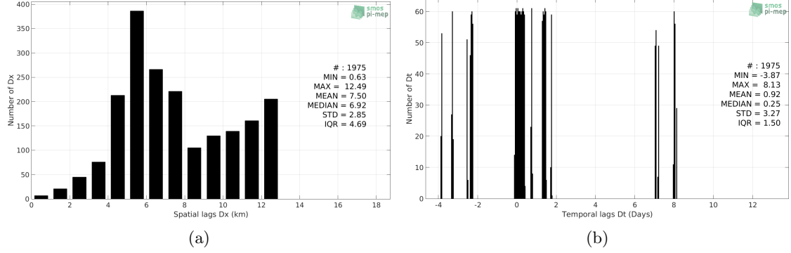
Figure 5: Histograms of the spatial (a) and temporal (b) lags between the location/time of the TSG (LEGOS-Surv-Adel) measurement and the date of the corresponding SMOS SSS L3 v335 - Monthly - 25 km (CATDS-CPDC) SSS pixel.
