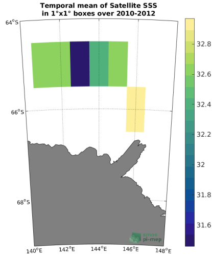
(a) MEAN(Satellite SSS)
