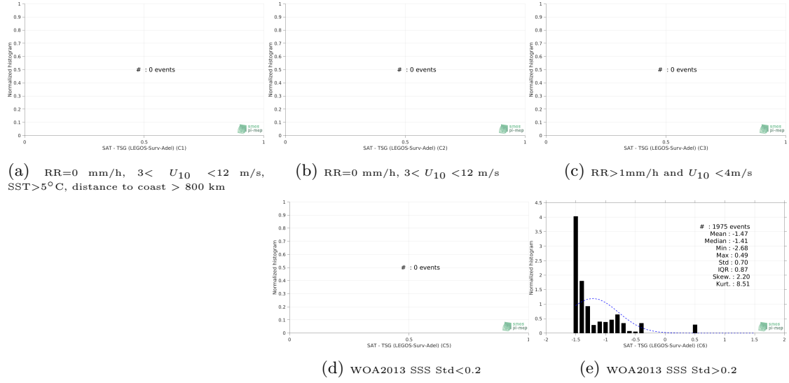
Figure 13: Normalized histogram of \Delta\text{SSS} (SMOS SSS L3 v335 - Monthly - 25 km (CATDS-CPDC) - TSG (LEGOS-Surv-Adel)) for 5 different subdatasets corresponding to: RR=0 mm/h, 3 < U_{10} < 12 m/s, SST > 5^\circ\text{C} , distance to coast > 800 km (a), RR=0 mm/h, 3 < U_{10} < 12 m/s (b), RR > 1\text{mm/h} and U_{10} < 4\text{m/s} (c), WOA2013 SSS Std < 0.2 (d), WOA2013 SSS Std > 0.2 (e).
