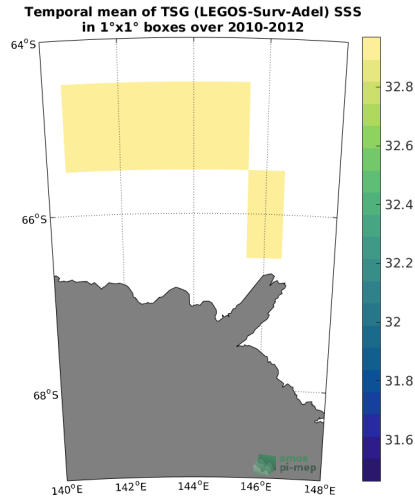
(c) MEAN(TSG (LEGOS-Surv-Adel) SSS)
