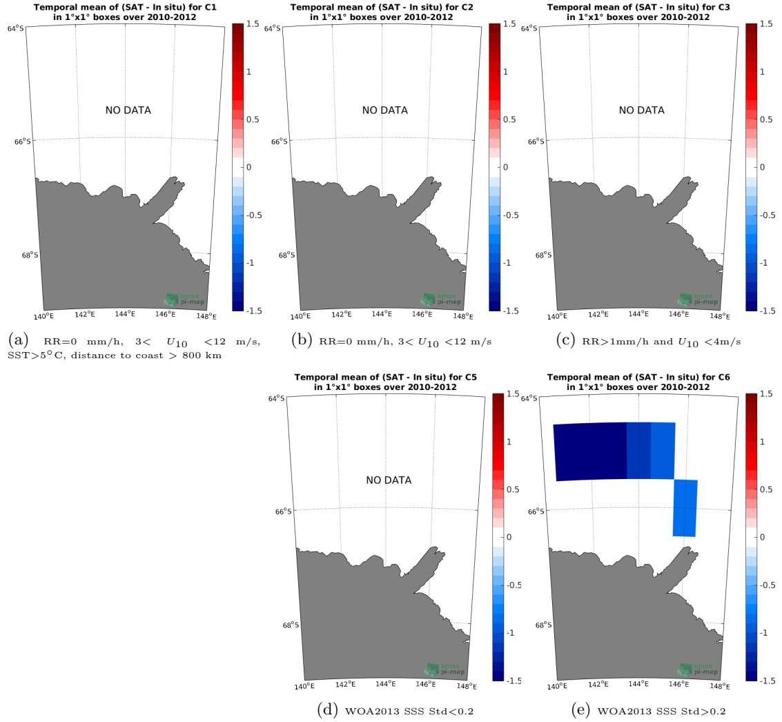
Figure 12: Temporal mean gridded over spatial boxes of size 1^{\circ} \times 1^{\circ} of \Delta\text{SSS} (SMOS SSS L3 v335 - Monthly - 25 km (CATDS-CPDC) - TSG (LEGOS-Surv-Adel)) for 5 different subdatasets corresponding to: RR=0 mm/h, 3 < U_{10} < 12 m/s, SST > 5^{\circ}\text{C} , distance to coast > 800 km (a), RR=0 mm/h, 3 < U_{10} < 12 m/s (b), RR > 1 mm/h and U_{10} < 4 m/s (c), WOA2013 SSS Std < 0.2 (d), WOA2013 SSS Std > 0.2 (e).
