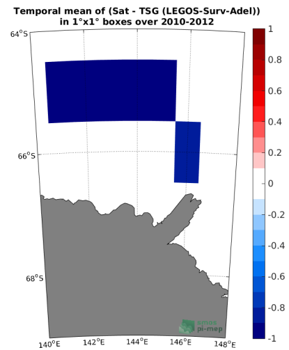
(e) MEAN( \Delta SSS) (Satellite - TSG (LEGOS-Surv-Adel))
