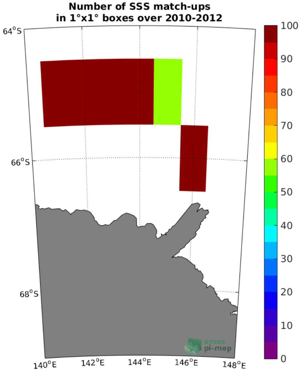
Figure 4: Number of SSS match-ups between TSG (LEGOS-Surv-Adel) SSS and the SMOS SSS L3 v335 - Monthly - 25 km (CATDS-CPDC) SSS product for the Global Ocean Pi-MEP region over 1°x1° boxes and for the full satellite product period.
