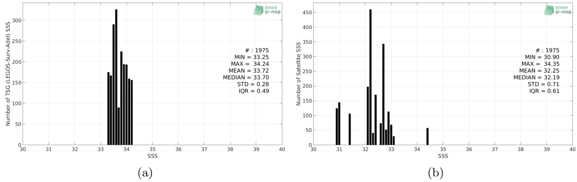
Figure 2: Histograms of SSS from TSG (LEGOS-Surv-Adel) (a) and SMOS SSS L3 v335 - Monthly - 25 km (CATDS-CPDC) (b) considering all match-up pairs per bins of 0.1 over the Global Ocean Pi-MEP region and for the full satellite product period.
