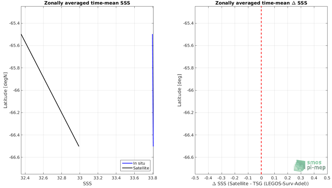
Figure 8: Left panel: Zonal mean SSS from SMOS SSS L3 v335 - Monthly - 25 km (CATDS-CPDC) satellite product (black) and from TSG (LEGOS-Surv-Adel) (blue). Right panel: Zonal mean of \Delta SSS (Satellite - TSG (LEGOS-Surv-Adel)) for all the collected Pi-MEP match-up pairs estimated over the full satellite product period.
