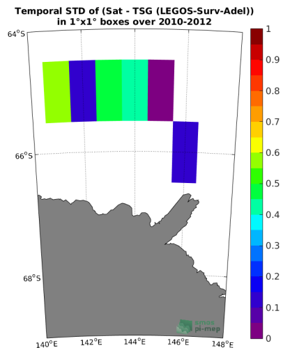
(f) Std( \Delta SSS) (Satellite - TSG (LEGOS-Surv-Adel))
