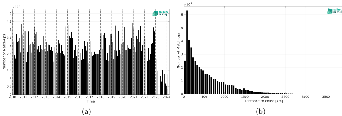
Figure 2: Number of match-ups between TSG (LEGOS-DM) and SMOS SSS L3 v335 - Monthly - 25 km (CATDS-CPDC) SSS as a function of time (a) and as function of the distance to coast (b) over the Global Ocean Pi-MEP region and for the full satellite product period.
