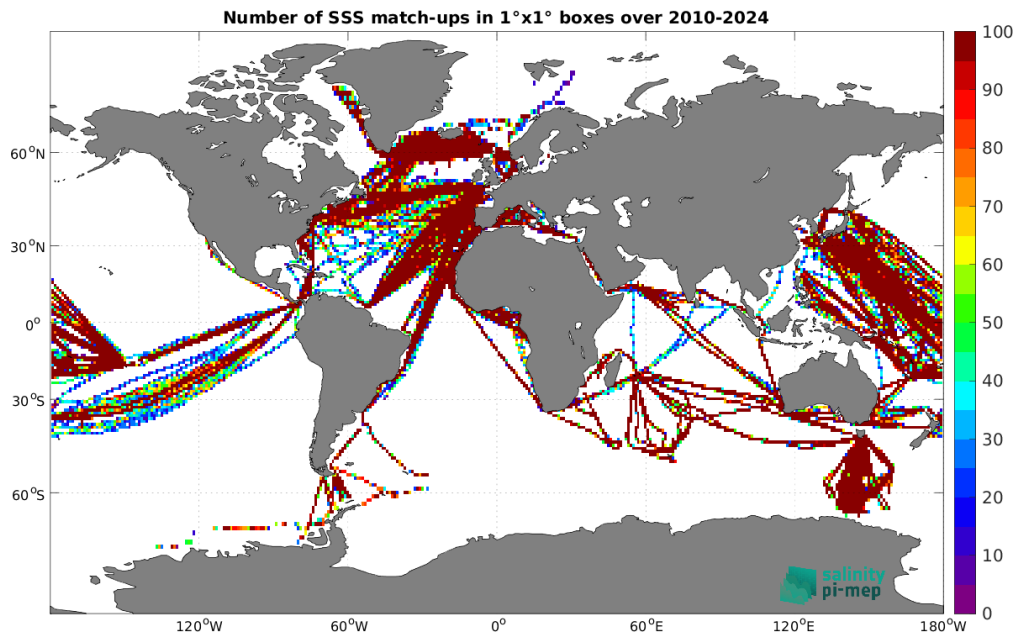
Figure 5: Number of SSS match-ups between TSG (LEGOS-DM) SSS and the SMOS SSS L3 v335 - Monthly - 25 km (CATDS-CPDC) SSS product for the Global Ocean Pi-MEP region over 1^\circ \times 1^\circ boxes and for the full satellite product period.
