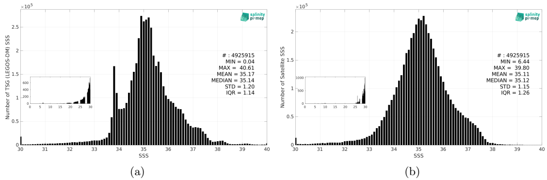
Figure 3: Histograms of SSS from TSG (LEGOS-DM) (a) and SMOS SSS L3 v335 - Monthly - 25 km (CATDS-CPDC) (b) considering all match-up pairs per bins of 0.1 over the Global Ocean Pi-MEP region and for the full satellite product period.
