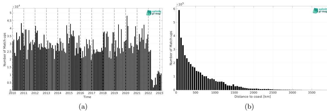
Figure 2: Number of match-ups between TSG (LEGOS-DM) and SMOS SSS L3 v335 - Monthly - 25 km (CATDS-CPDC) SSS as a function of time (a) and as function of the distance to coast (b) over the Global Ocean Pi-MEP region and for the full satellite product period.
