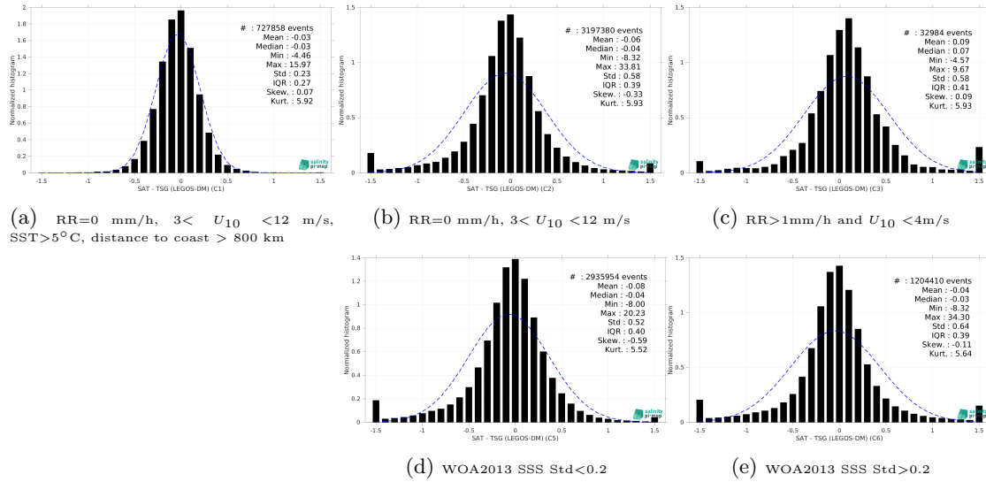
Figure 15: Normalized histogram of \Delta\text{SSS} (SMOS SSS L3 v335 - Monthly - 25 km (CATDS-CPDC) - TSG (LEGOS-DM)) for 5 different subdatasets corresponding to: RR=0 mm/h, 3 < U_{10} < 12 m/s, SST>5°C, distance to coast > 800 km (a), RR=0 mm/h, 3 < U_{10} < 12 m/s (b), RR>1mm/h and U_{10} < 4 m/s (c), WOA2013 SSS Std<0.2 (d), WOA2013 SSS Std>0.2 (e).
