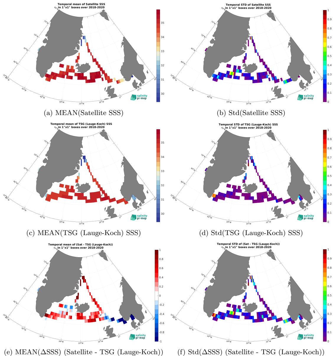
Figure 7: Temporal mean (left) and Std (right) of SSS from SMOS SSS L3 v335 - Monthly - 25 km (CATDS-CPDC) (top), TSG (Lauge-Koch) (middle), and of \Delta SSS (Satellite - TSG (Lauge-Koch)). Only match-up pairs are used to generate these maps.
