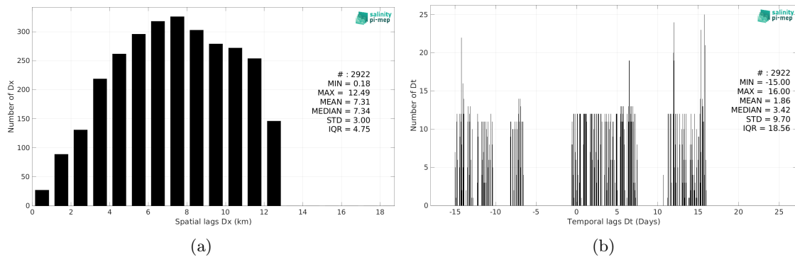
Figure 6: Histograms of the spatial (a) and temporal (b) lags between the location/time of the TSG (Lauge-Koch) measurement and the date of the corresponding SMOS SSS L3 v335 - Monthly - 25 km (CATDS-CPDC) SSS pixel.
