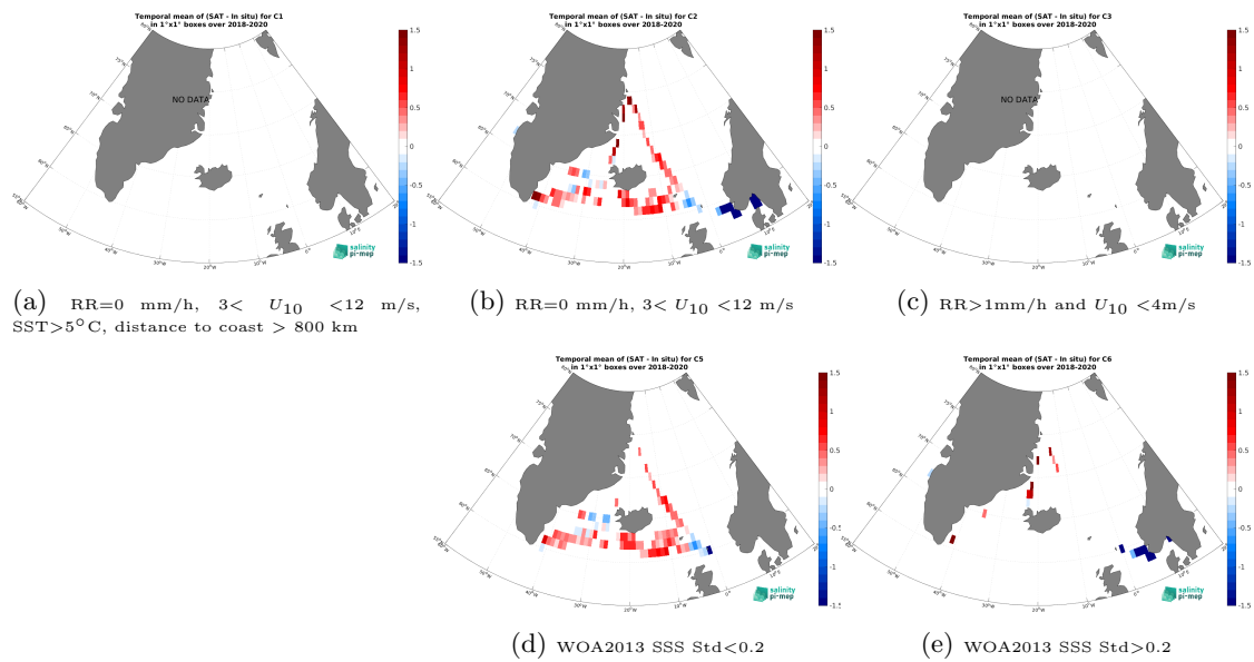
Figure 14: Temporal mean gridded over spatial boxes of size 1^\circ \times 1^\circ of \Delta SSS (SMOS SSS L3 v335 - Monthly - 25 km (CATDS-CPDC) - TSG (Lauge-Koch)) for 5 different subdatasets corresponding to: RR=0 mm/h, 3 < U_{10} < 12 m/s, SST > 5^\circ\text{C} , distance to coast > 800 km (a), RR=0 mm/h, 3 < U_{10} < 12 m/s (b), RR > 1 mm/h and U_{10} < 4 m/s (c), WOA2013 SSS Std < 0.2 (d), WOA2013 SSS Std > 0.2 (e).
