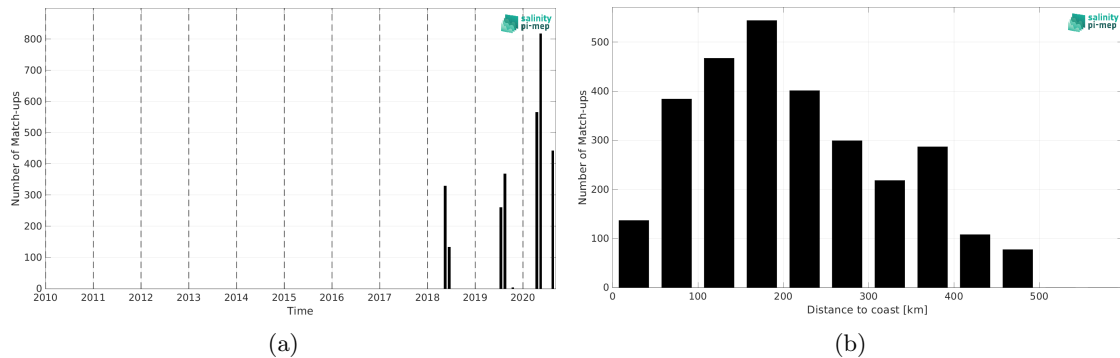
Figure 2: Number of match-ups between TSG (Lauge-Koch) and SMOS SSS L3 v335 - Monthly - 25 km (CATDS-CPDC) SSS as a function of time (a) and as function of the distance to coast (b) over the Global Ocean Pi-MEP region and for the full satellite product period.
