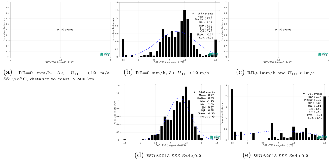
Figure 15: Normalized histogram of \Delta SSS (SMOS SSS L3 v335 - Monthly - 25 km (CATDS-CPDC) - TSG (Lauge-Koch)) for 5 different subdatasets corresponding to: RR=0 mm/h, 3 < U_{10} < 12 m/s, SST>5°C, distance to coast > 800 km (a), RR=0 mm/h, 3 < U_{10} < 12 m/s (b), RR>1mm/h and U_{10} < 4 m/s (c), WOA2013 SSS Std<0.2 (d), WOA2013 SSS Std>0.2 (e).
