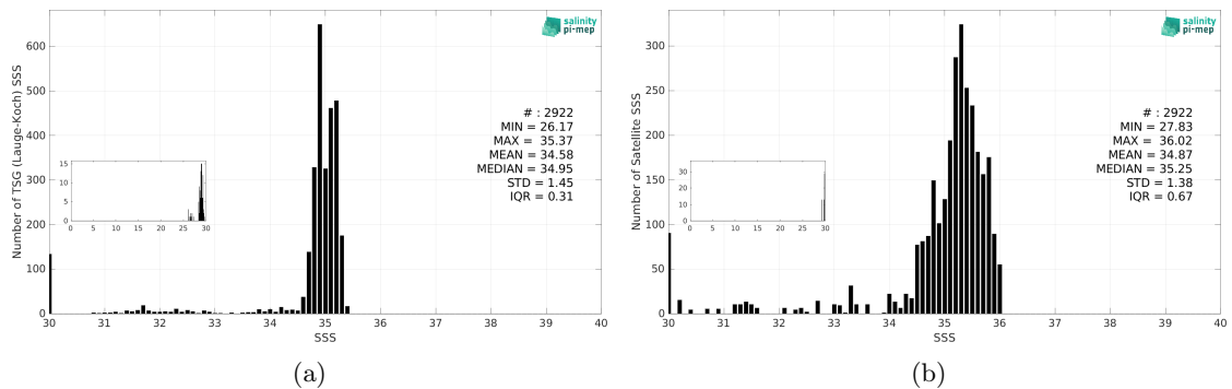
Figure 3: Histograms of SSS from TSG (Lauge-Koch) (a) and SMOS SSS L3 v335 - Monthly - 25 km (CATDS-CPDC) (b) considering all match-up pairs per bins of 0.1 over the Global Ocean Pi-MEP region and for the full satellite product period.
