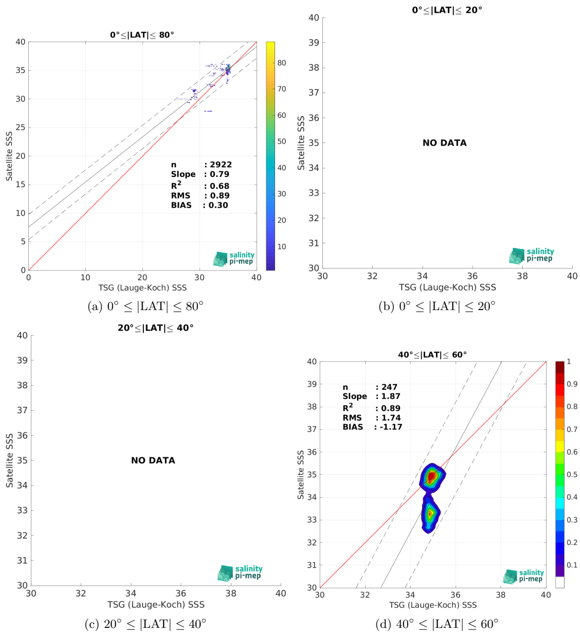
Figure 10: Contour maps of the concentration of SMOS SSS L3 v335 - Monthly - 25 km (CATDS-CPDC) SSS (y-axis) versus TSG (Lauge-Koch) SSS (x-axis) at match-up pairs for different latitude bands. For each plot, the red line shows x=y . The black thin and dashed lines indicate a linear fit through the data cloud and the \pm 95\% confidence levels, respectively. The number match-up pairs n , the slope and R^2 coefficient of the linear fit, the root mean square (RMS) and the mean bias between satellite and in situ data are indicated for each latitude band in each plots.
