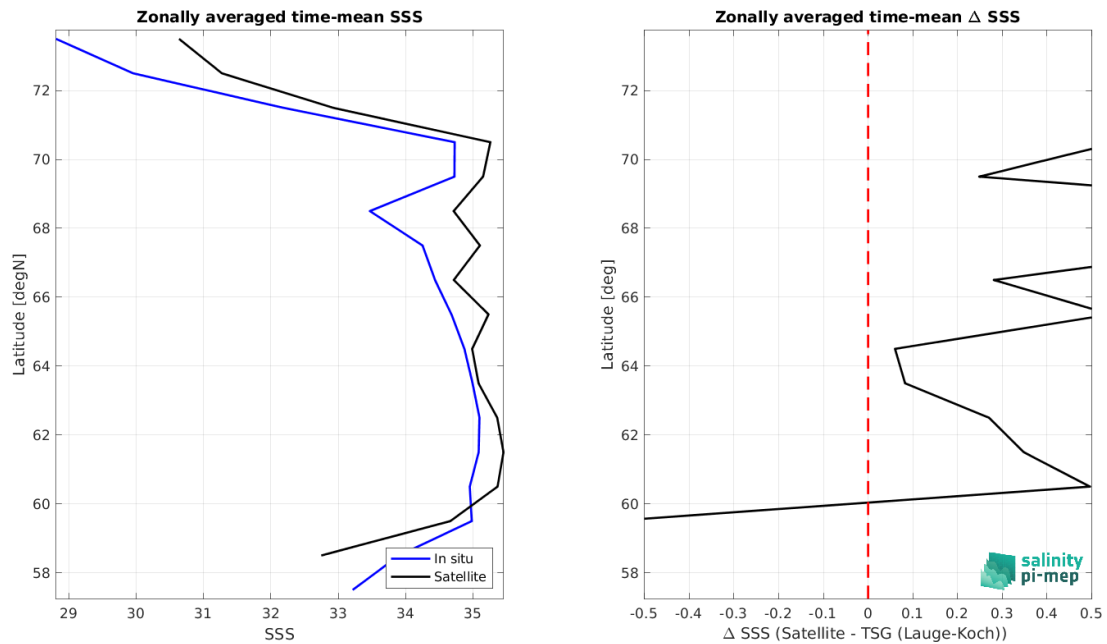
Figure 9: Left panel: Zonal mean SSS from SMOS SSS L3 v335 - Monthly - 25 km (CATDS-CPDC) satellite product (black) and from TSG (Lauge-Koch) (blue). Right panel: Zonal mean of \Delta SSS (Satellite - TSG (Lauge-Koch)) for all the collected Pi-MEP match-up pairs estimated over the full satellite product period.
