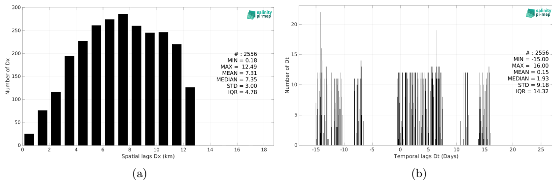
Figure 5: Histograms of the spatial (a) and temporal (b) lags between the location/time of the TSG (Lauge-Koch) measurement and the date of the corresponding SMOS SSS L3 v335 - Monthly - 25 km (CATDS-CPDC) SSS pixel.
