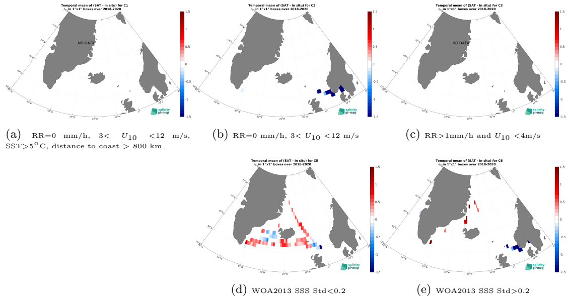
Figure 12: Temporal mean gridded over spatial boxes of size 1^{\circ}\times 1^{\circ} of \Delta\text{SSS} (SMOS SSS L3 v335 - Monthly - 25 km (CATDS-CPDC) - TSG (Lauge-Koch)) for 5 different subdatasets corresponding to:RR=0 mm/h, 3 < U_{10} < 12 m/s, SST >5^{\circ}\text{C} , distance to coast > 800 km (a), RR=0 mm/h, 3 < U_{10} < 12 m/s (b), RR >1 mm/h and U_{10} < 4 m/s (c), WOA2013 SSS Std <0.2 (d), WOA2013 SSS Std >0.2 (e).
