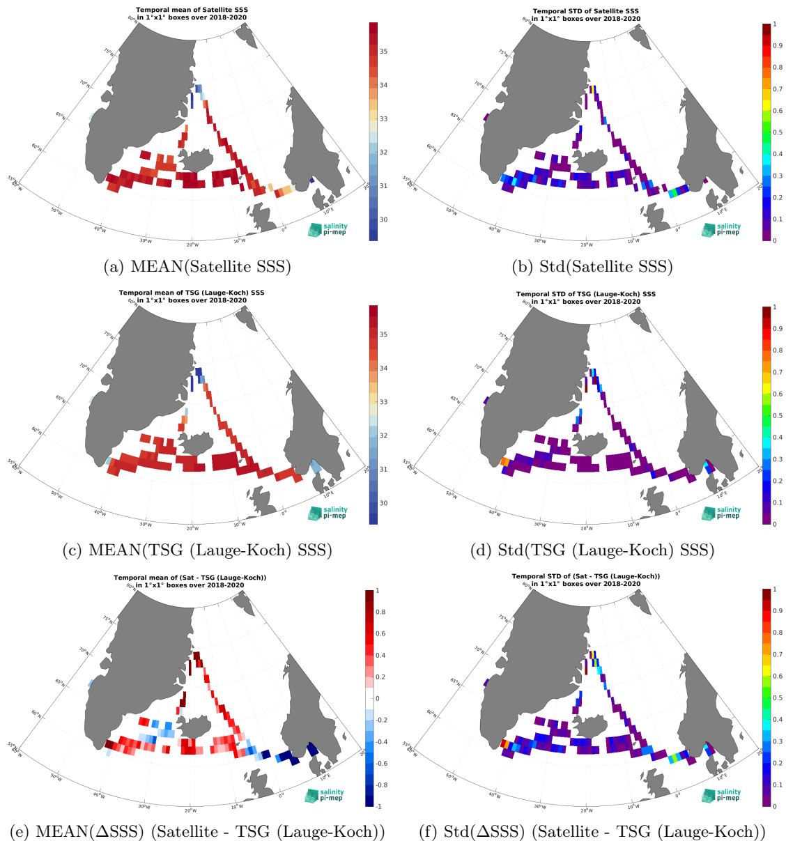
Figure 6: Temporal mean (left) and Std (right) of SSS from SMOS SSS L3 v335 - Monthly - 25 km (CATDS-CPDC) (top), TSG (Lauge-Koch) (middle), and of \Delta SSS (Satellite - TSG (Lauge-Koch)). Only match-up pairs are used to generate these maps.
