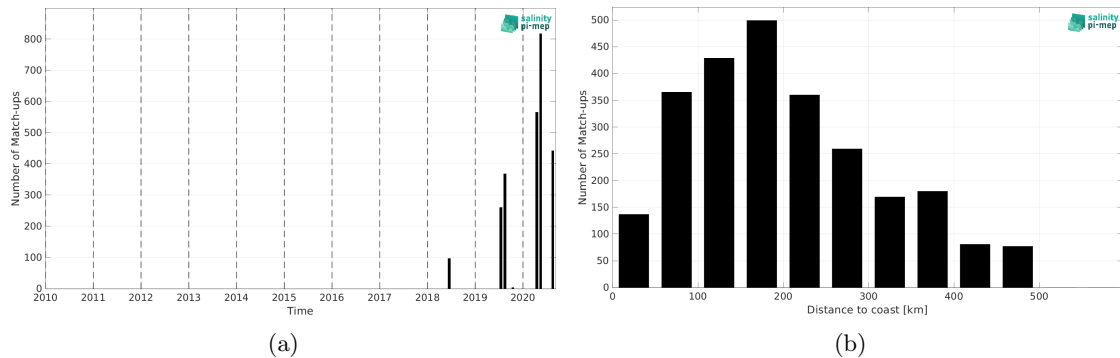
Figure 1: Number of match-ups between TSG (Lauge-Koch) and SMOS SSS L3 v335 - Monthly - 25 km (CATDS-CPDC) SSS as a function of time (a) and as function of the distance to coast (b) over the Global Ocean Pi-MEP region and for the full satellite product period.
