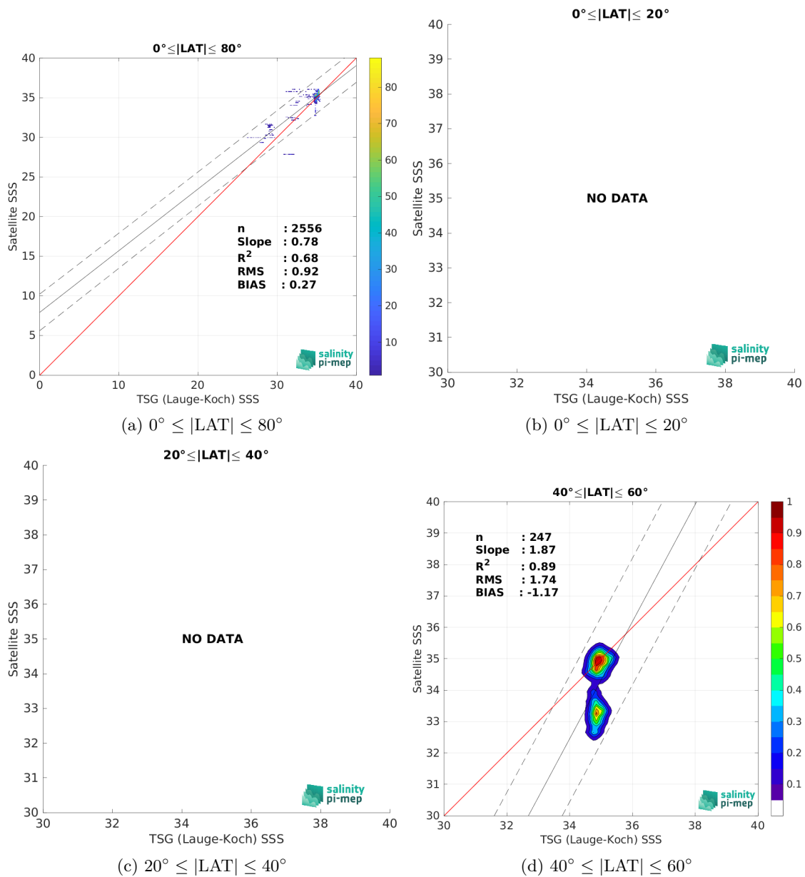
Figure 9: Contour maps of the concentration of SMOS SSS L3 v335 - Monthly - 25 km (CATDS-CPDC) SSS (y-axis) versus TSG (Lauge-Koch) SSS (x-axis) at match-up pairs for different latitude bands. For each plot, the red line shows x=y . The black thin and dashed lines indicate a linear fit through the data cloud and the \pm 95\% confidence levels, respectively. The number match-up pairs n , the slope and R^2 coefficient of the linear fit, the root mean square (RMS) and the mean bias between satellite and in situ data are indicated for each latitude band in each plots.
