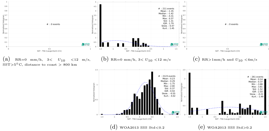
Figure 13: Normalized histogram of \Delta SSS (SMOS SSS L3 v335 - Monthly - 25 km (CATDS-CPDC) - TSG (Lauge-Koch)) for 5 different subdatasets corresponding to: RR=0 mm/h, 3 < U_{10} < 12 m/s, SST > 5°C, distance to coast > 800 km (a), RR=0 mm/h, 3 < U_{10} < 12 m/s (b), RR > 1mm/h and U_{10} < 4 m/s (c), WOA2013 SSS Std < 0.2 (d), WOA2013 SSS Std > 0.2 (e).
