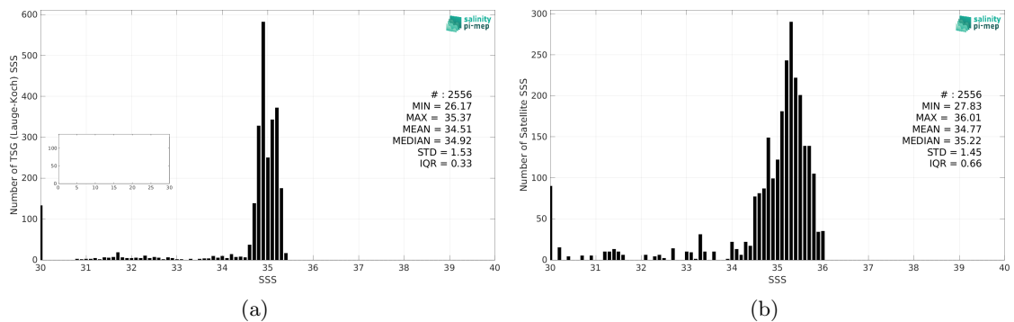
Figure 2: Histograms of SSS from TSG (Lauge-Koch) (a) and SMOS SSS L3 v335 - Monthly - 25 km (CATDS-CPDC) (b) considering all match-up pairs per bins of 0.1 over the Global Ocean Pi-MEP region and for the full satellite product period.
