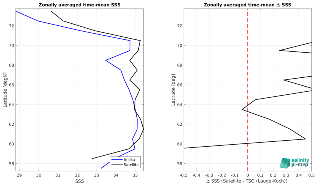
Figure 8: Left panel: Zonal mean SSS from SMOS SSS L3 v335 - Monthly - 25 km (CATDS-CPDC) satellite product (black) and from TSG (Lauge-Koch) (blue). Right panel: Zonal mean of \Delta SSS (Satellite - TSG (Lauge-Koch)) for all the collected Pi-MEP match-up pairs estimated over the full satellite product period.
