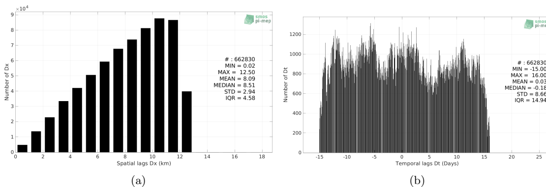
Figure 5: Histograms of the spatial (a) and temporal (b) lags between the location/time of the TSG (GOSUD-Sailing-ship) measurement and the date of the corresponding SMOS SSS L3 v335 - Monthly - 25 km (CATDS-CPDC) SSS pixel.
